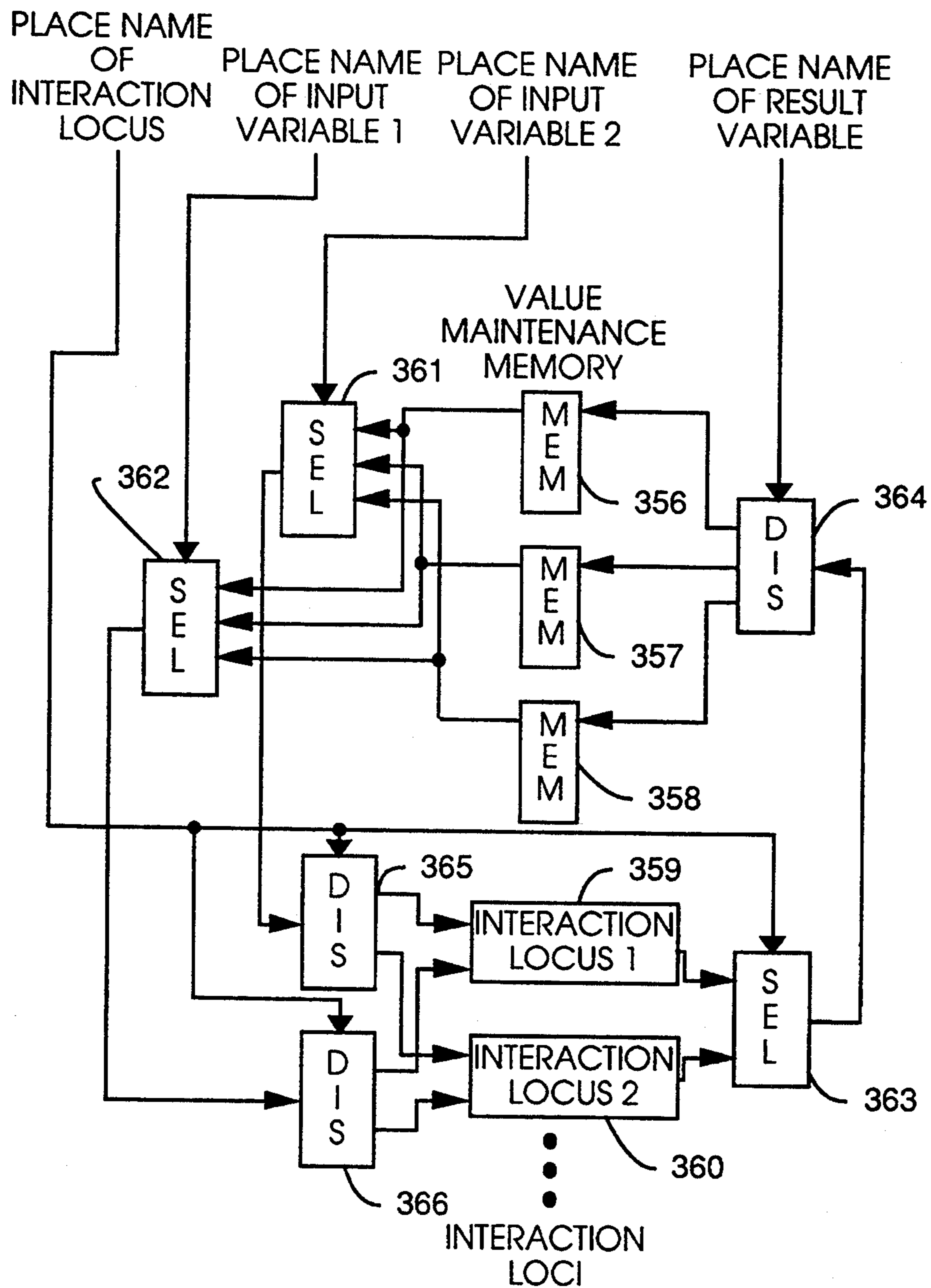
EXPRESSION WITH CONFIGURABLE ASSOCIATION RELATIONSHIPS
