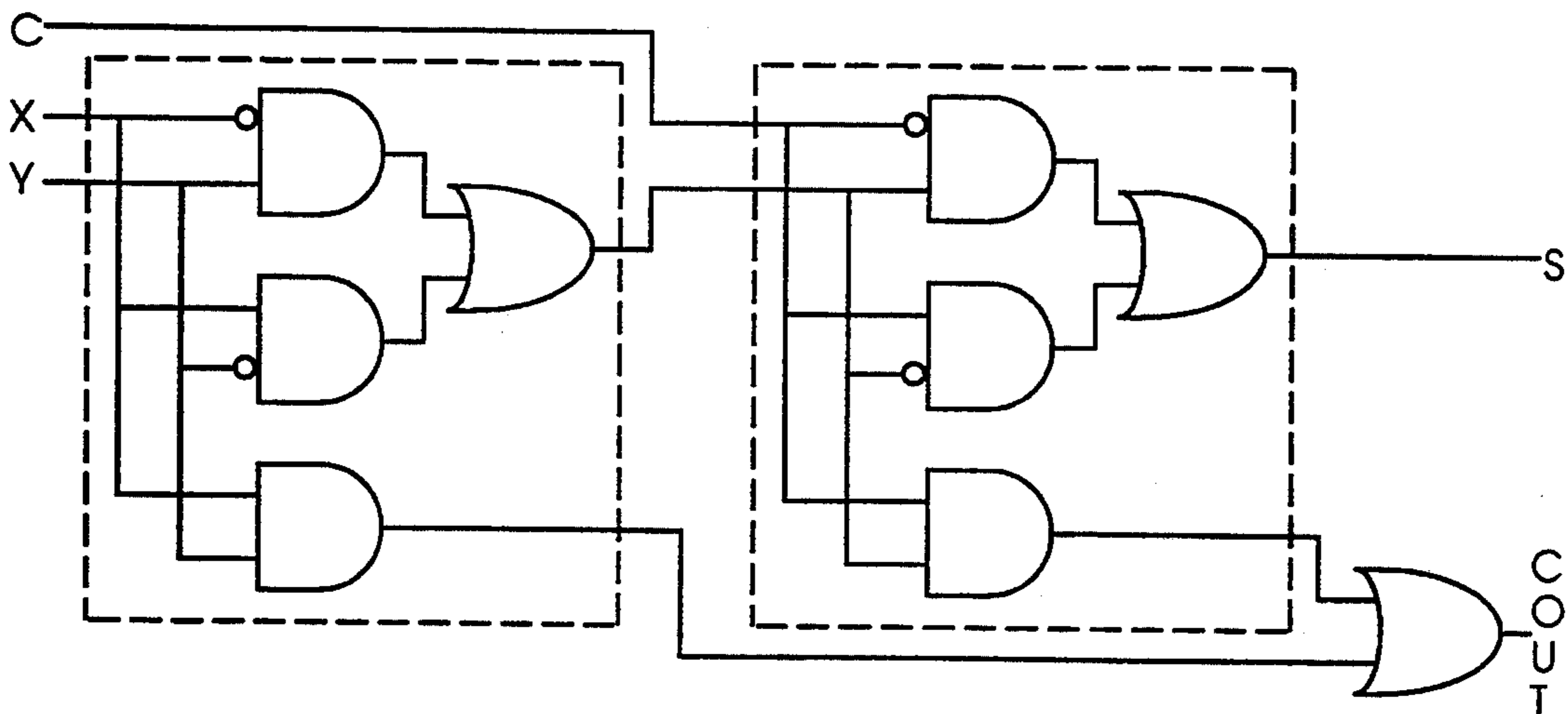
BINARY FULLADDER EXAMPLE EXPRESSION
