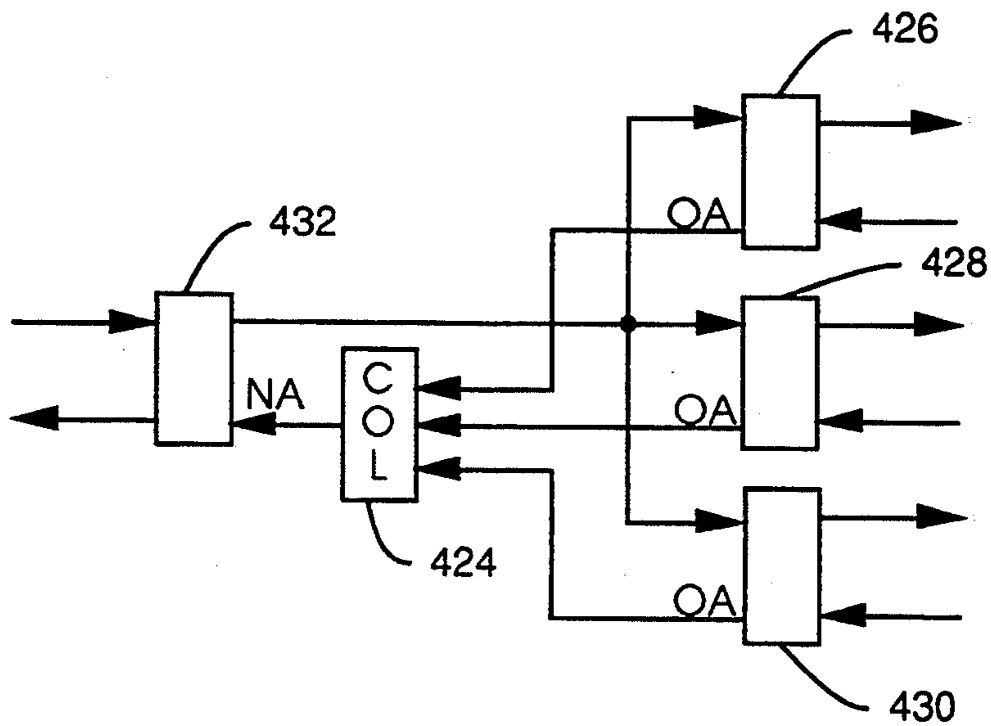
FAN OUT CONFIGURATION OF BOUNDARY ELEMENTS
