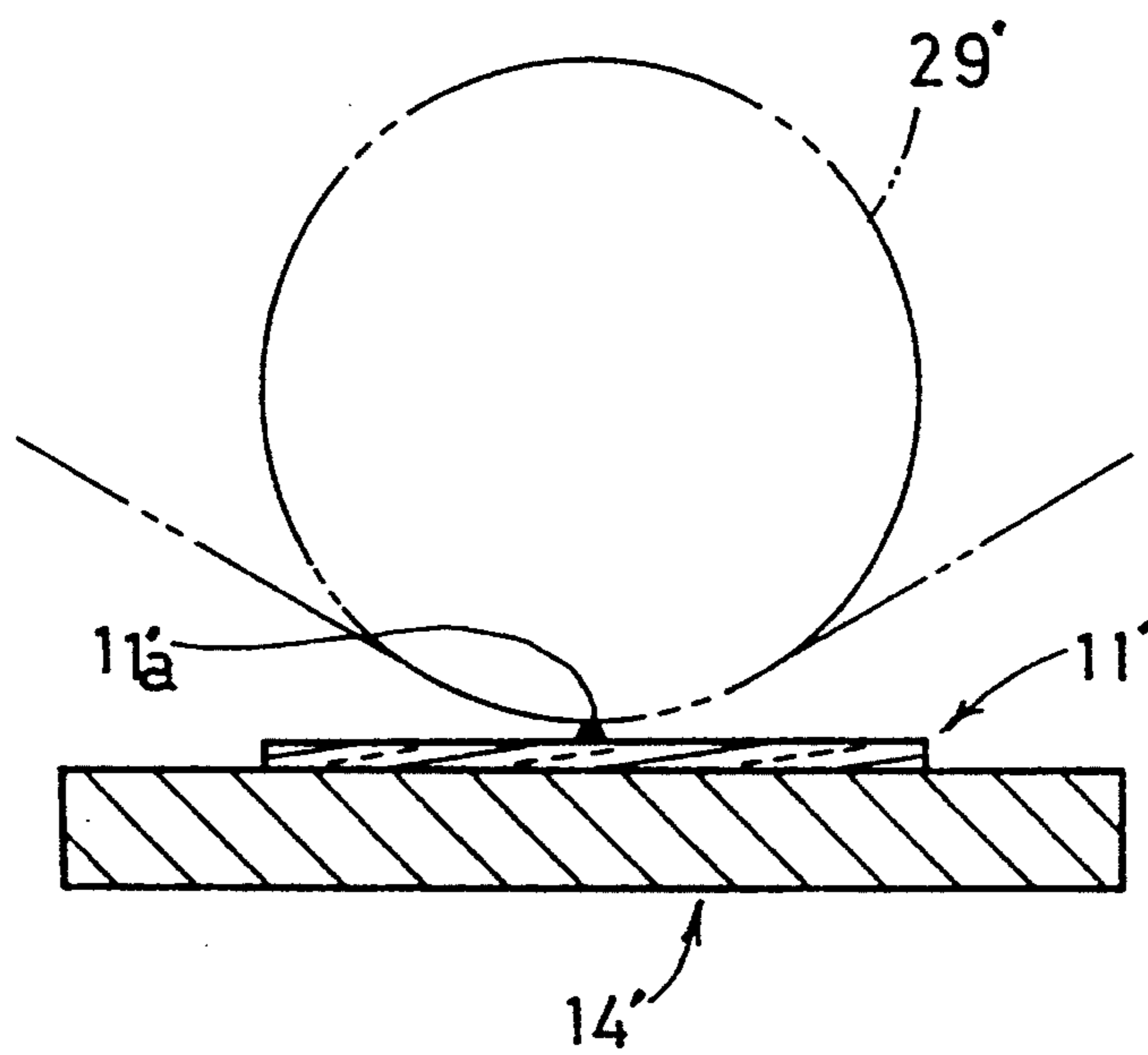
Fig. 14 Prior Art
