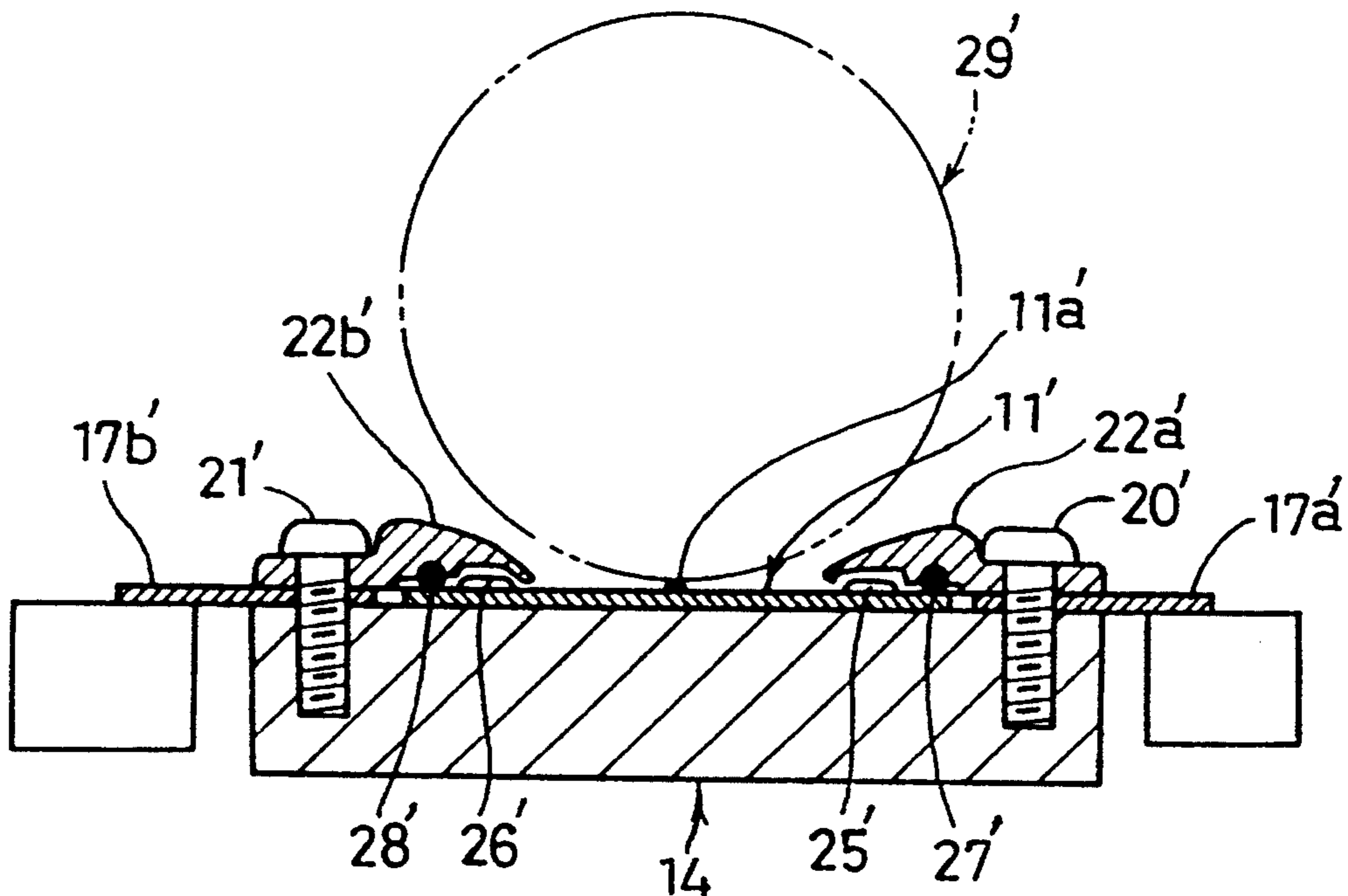
Fig. 16 Prior Art
