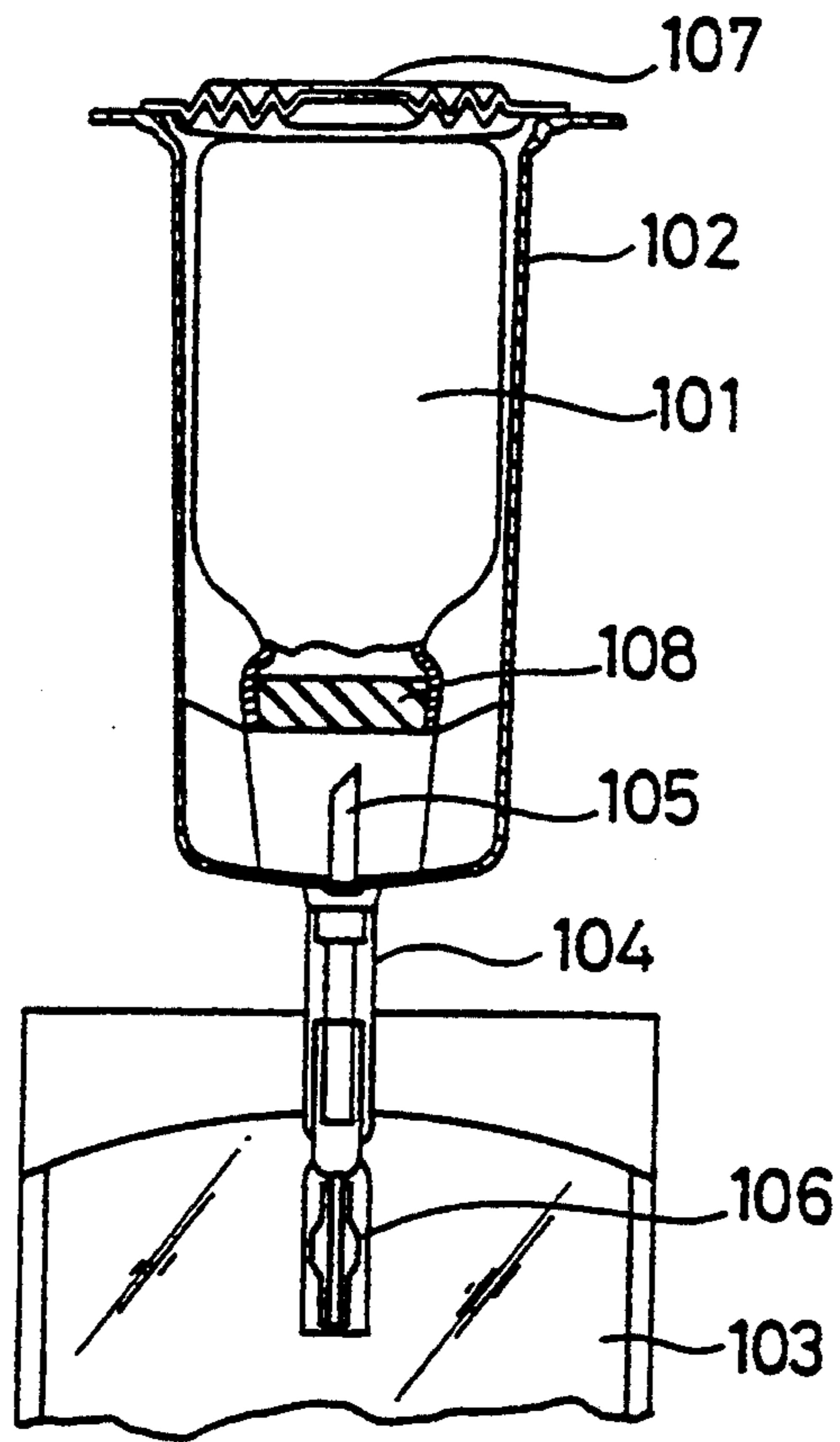
Fig 11 PRIOR ART
