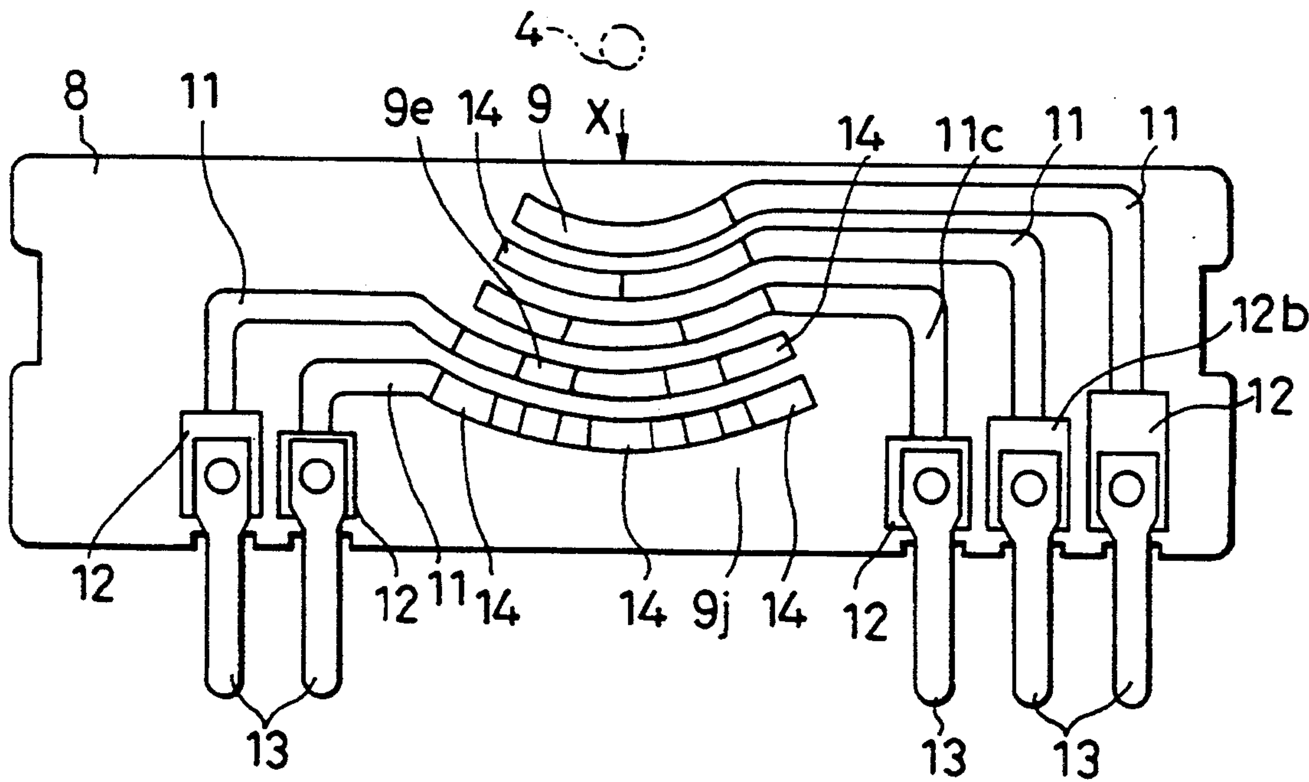
FIG. 7 (PRIOR ART)
