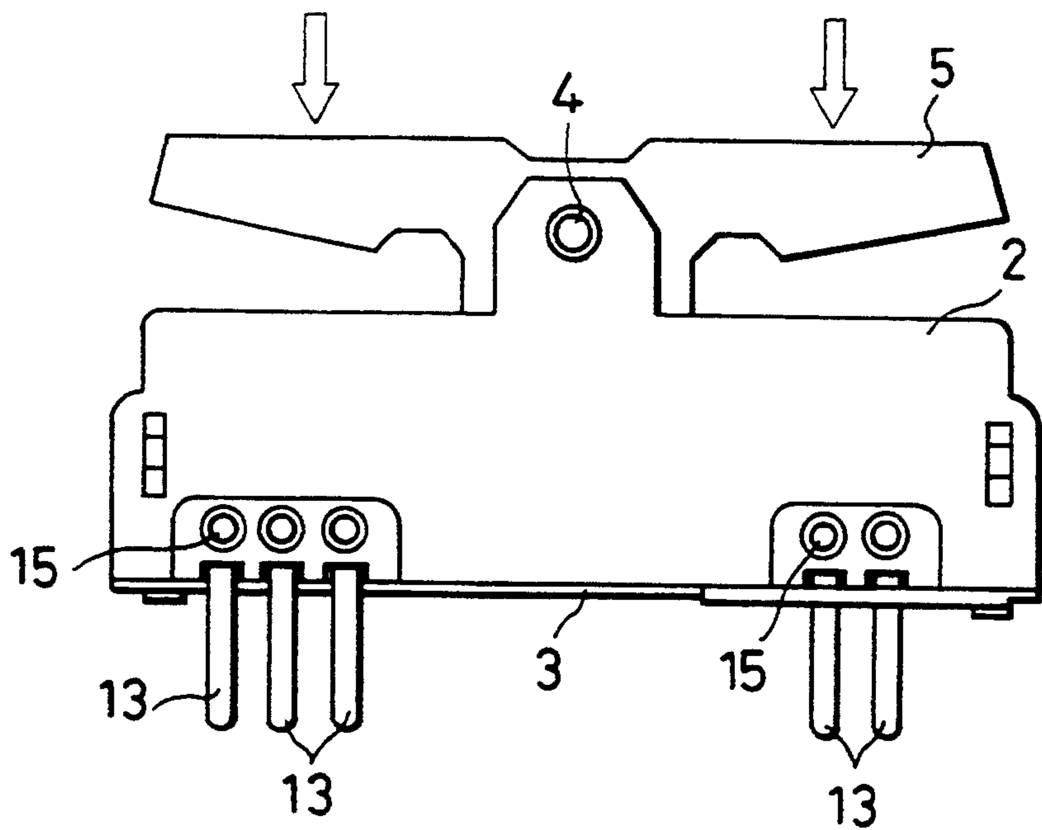
FIG. 6 (PRIOR ART)
