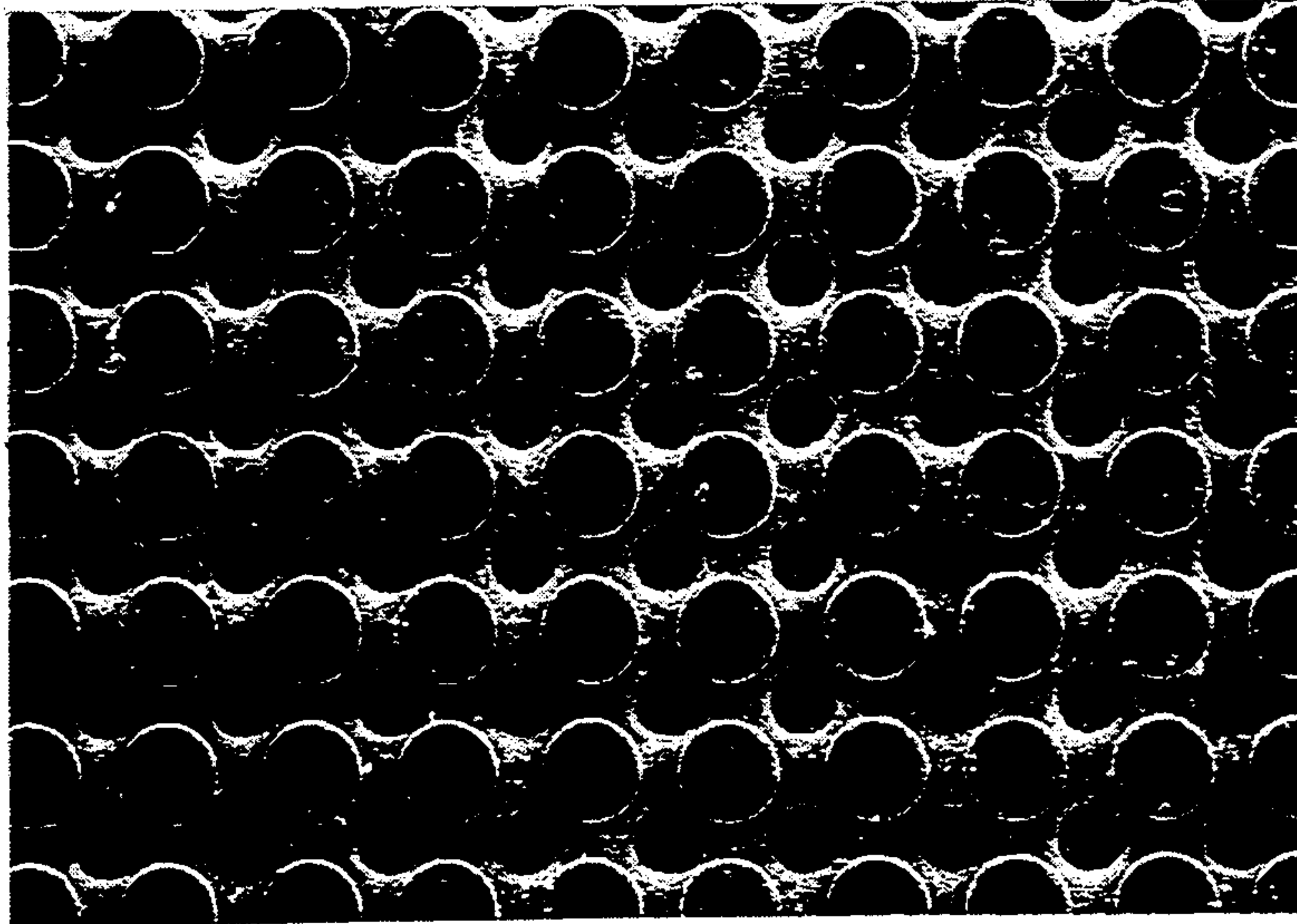
L=SEI EHT=13.0 KV WD=14 mm MAG=X50.0 PHOTO=6 500 \mu m ————— SILICONE REPLICATED SURFACE MESH
