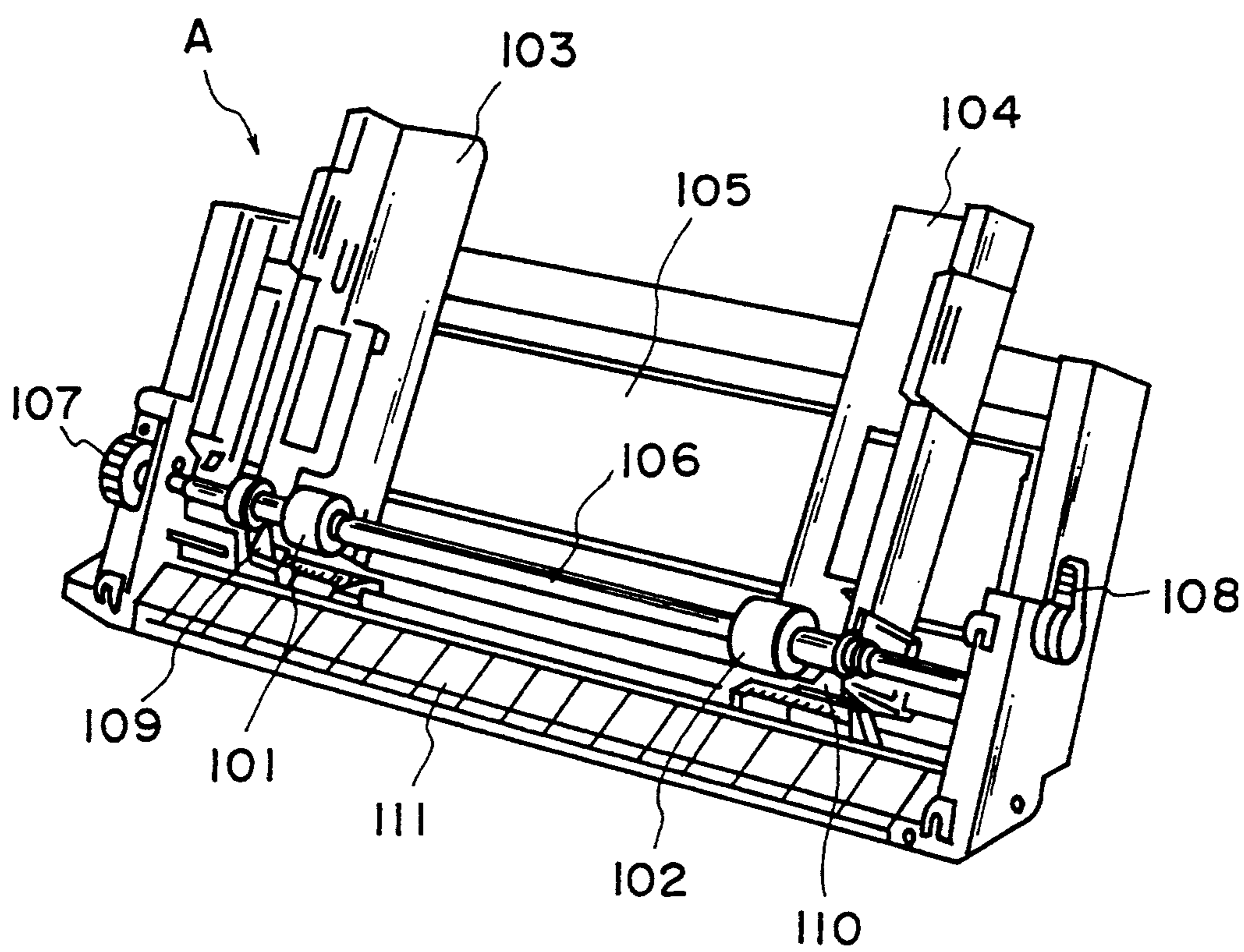
FIG. 12 PRIOR ART
