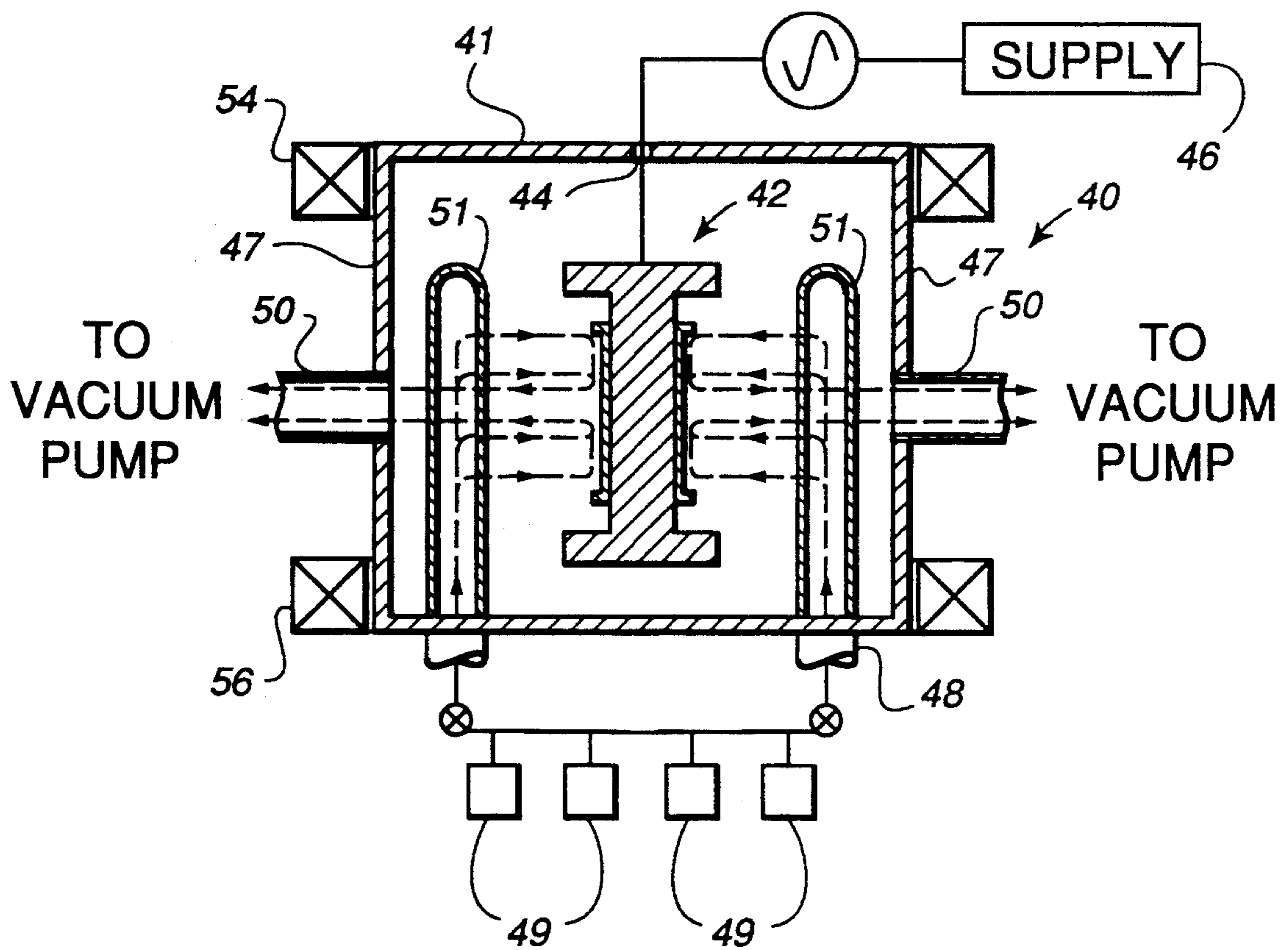
Figure 1 (PRIOR ART)
