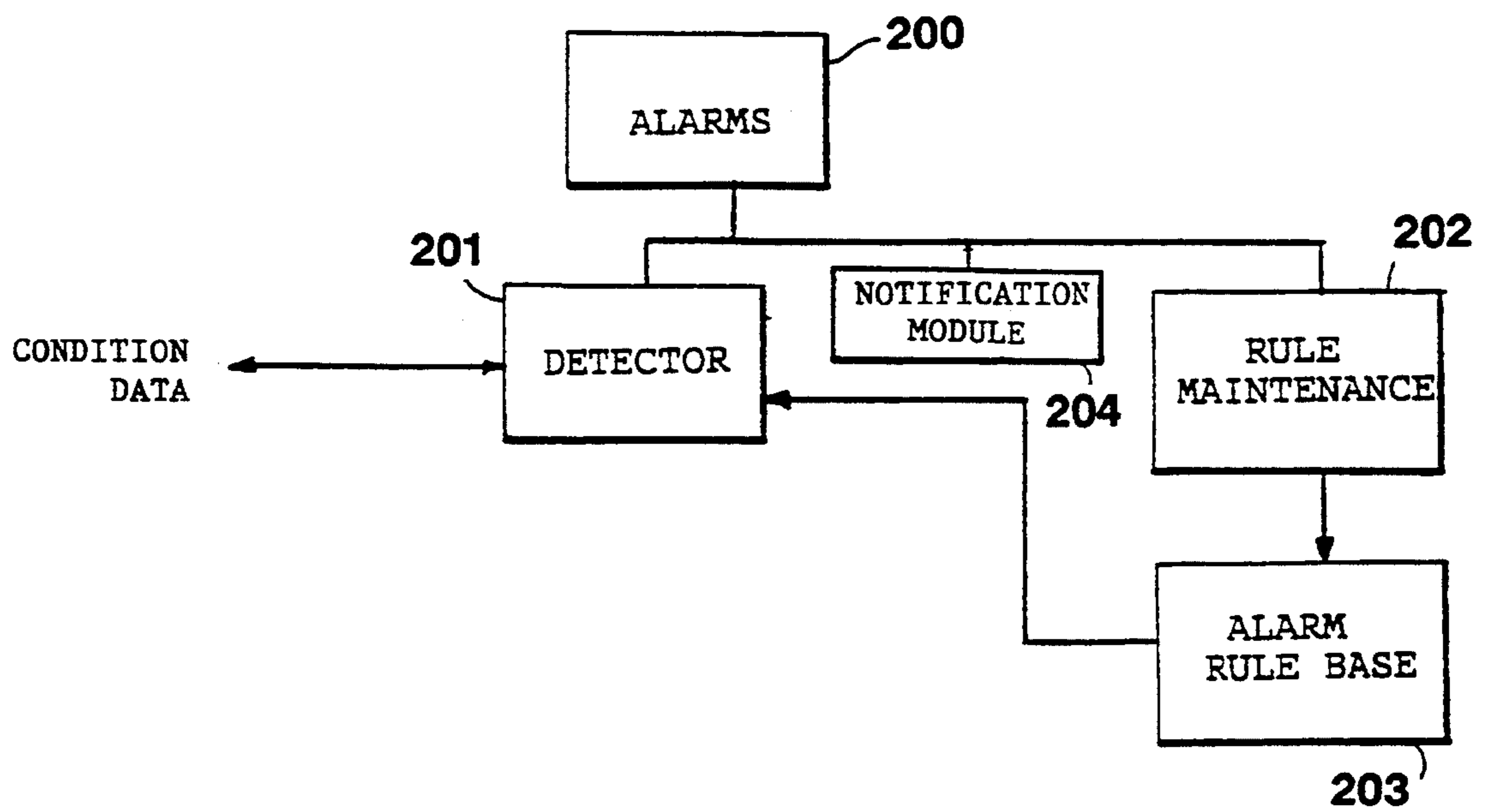
FIG. 10A ALARMS FUNCTIONAL MODULE
