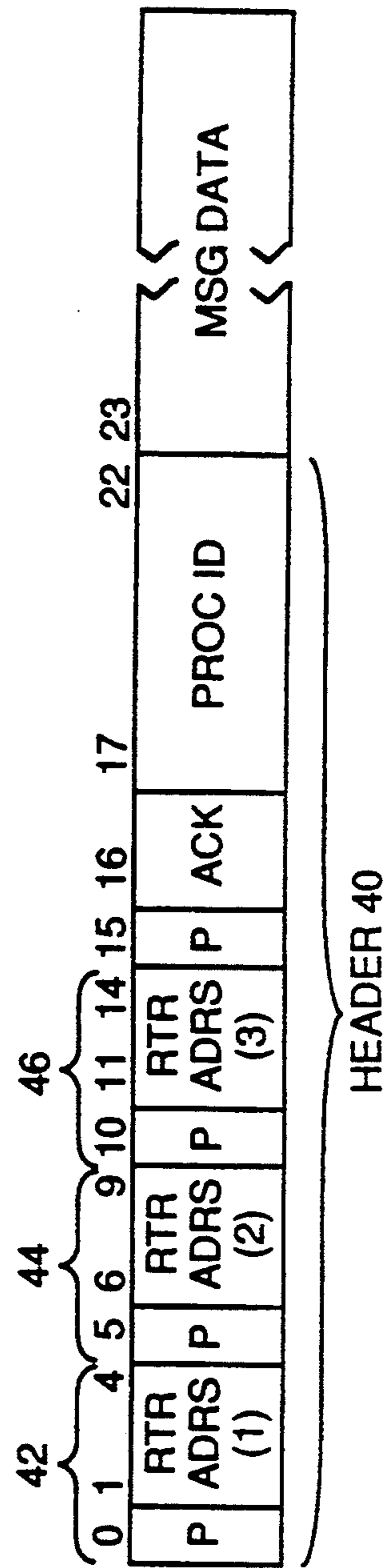
FIG. 2 (PRIOR ART)
