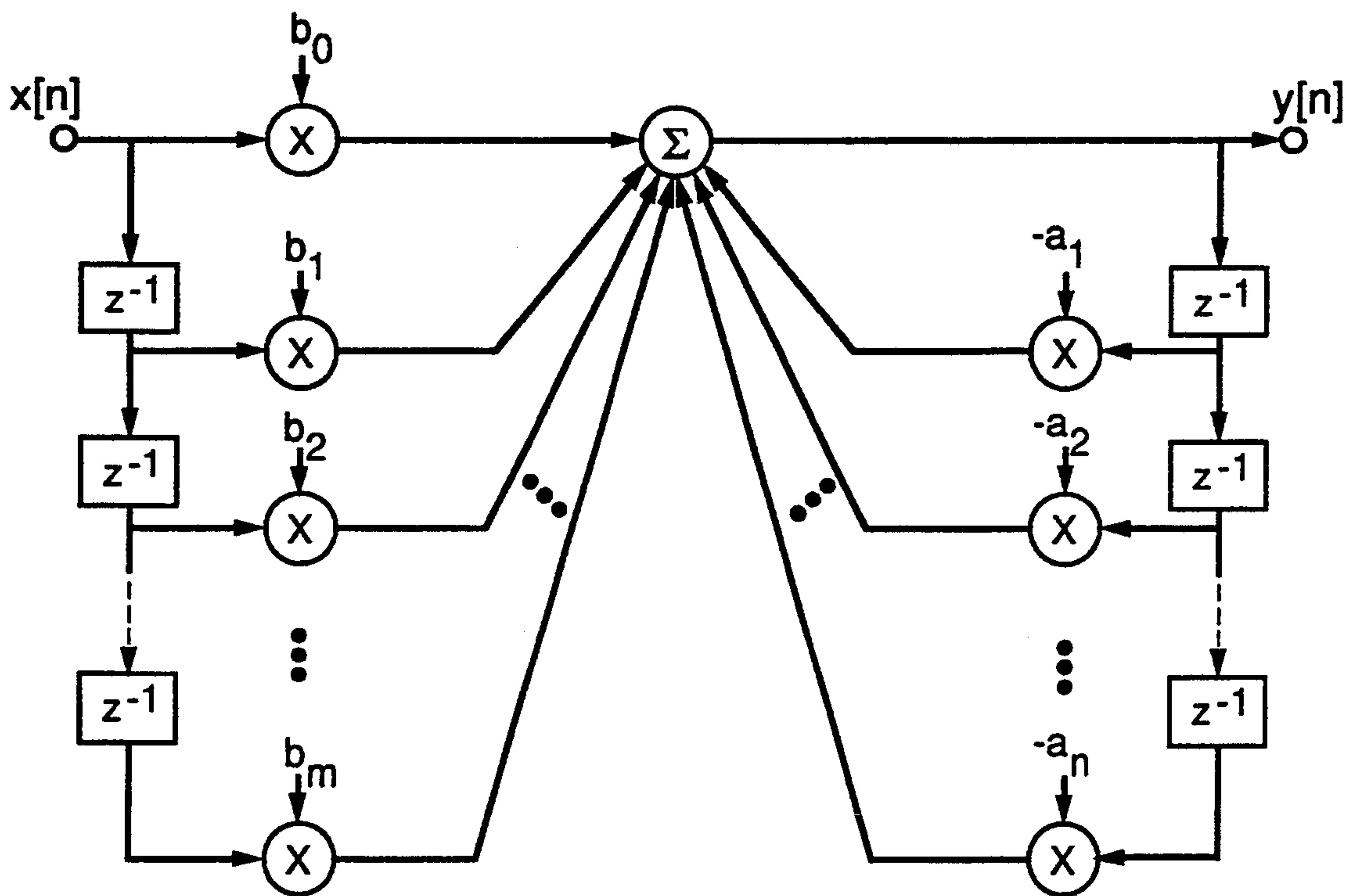
FIG. 10 (PRIOR ART)
