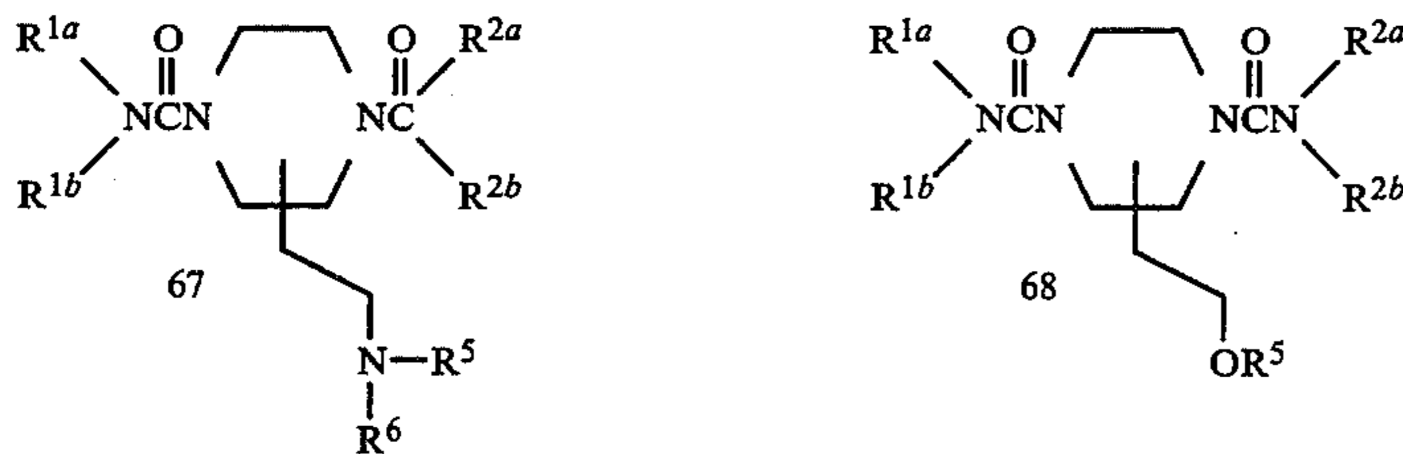
SCHEME 10
