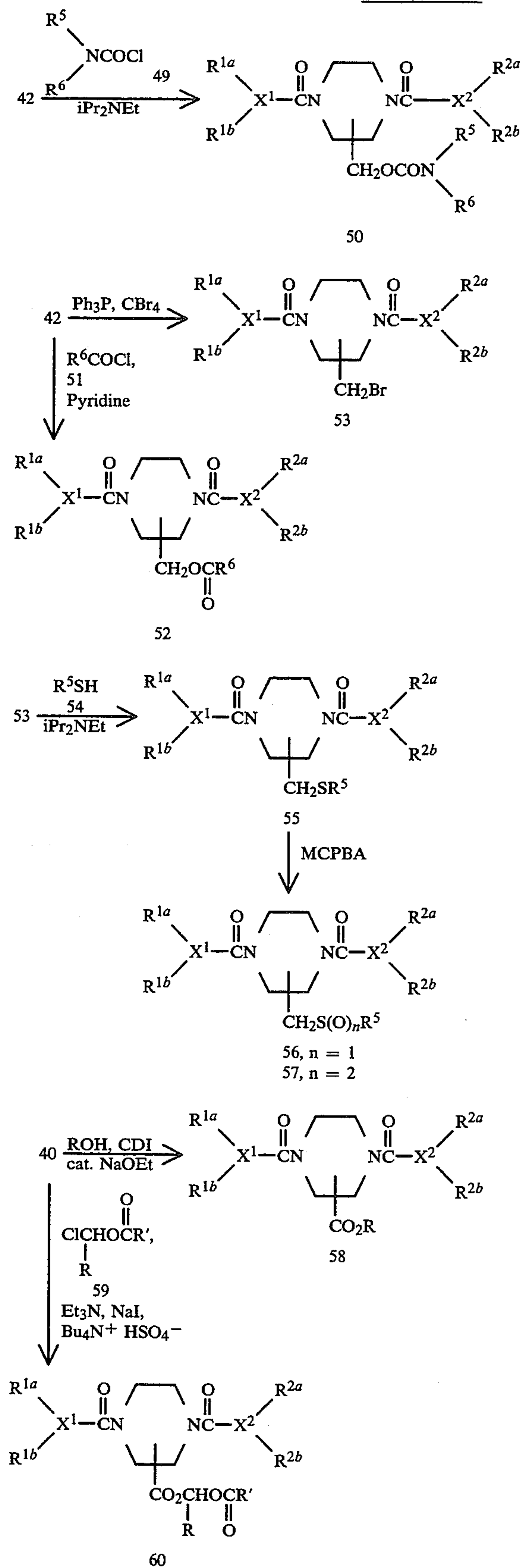
SCHEME 9
