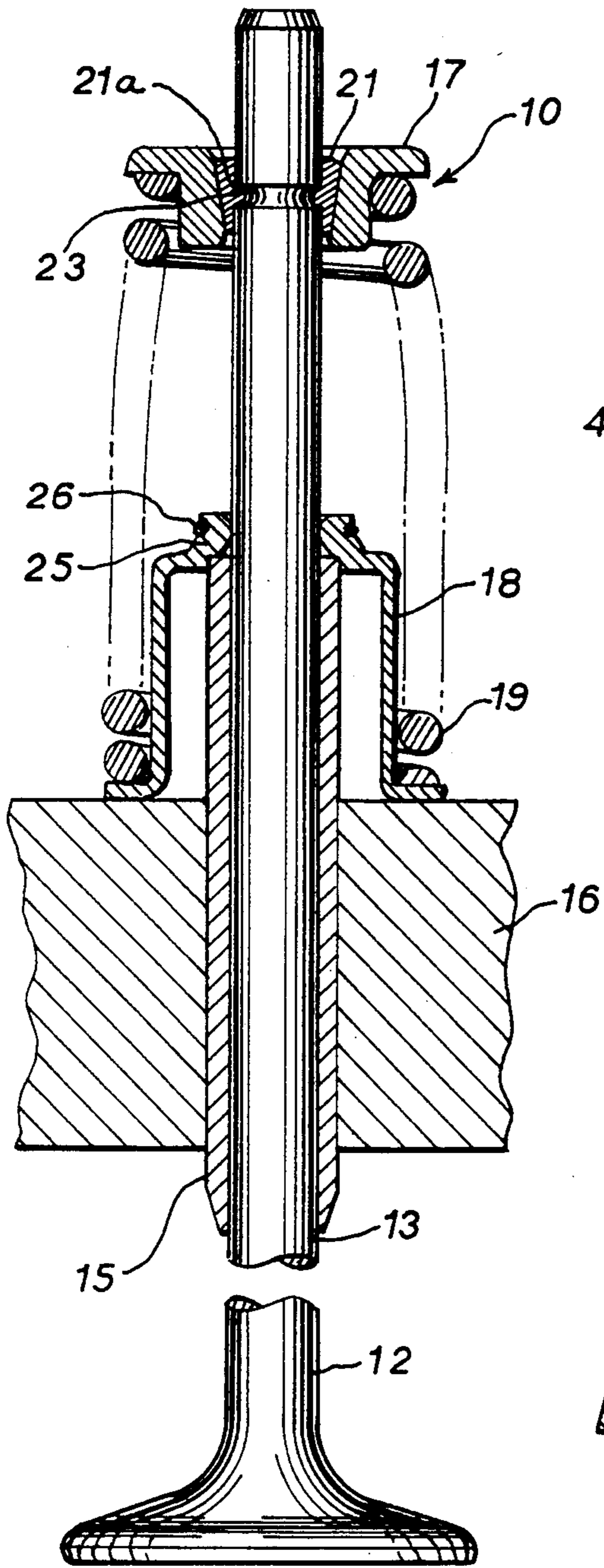
FIG 1 PRIOR ART
