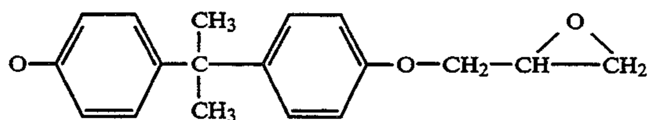
Bisphenol-A Epoxy Resin
