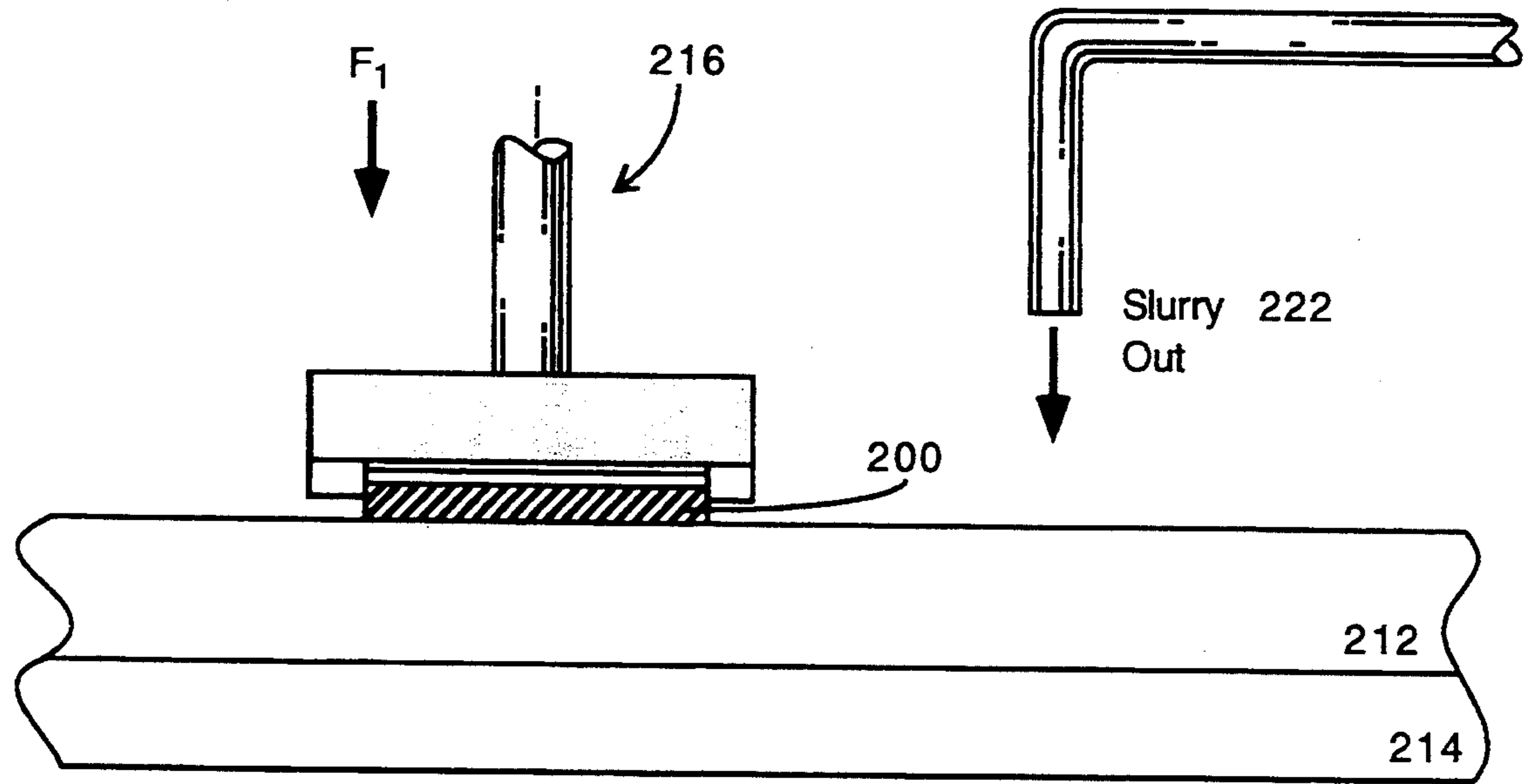
Figure 2c (Prior Art)
