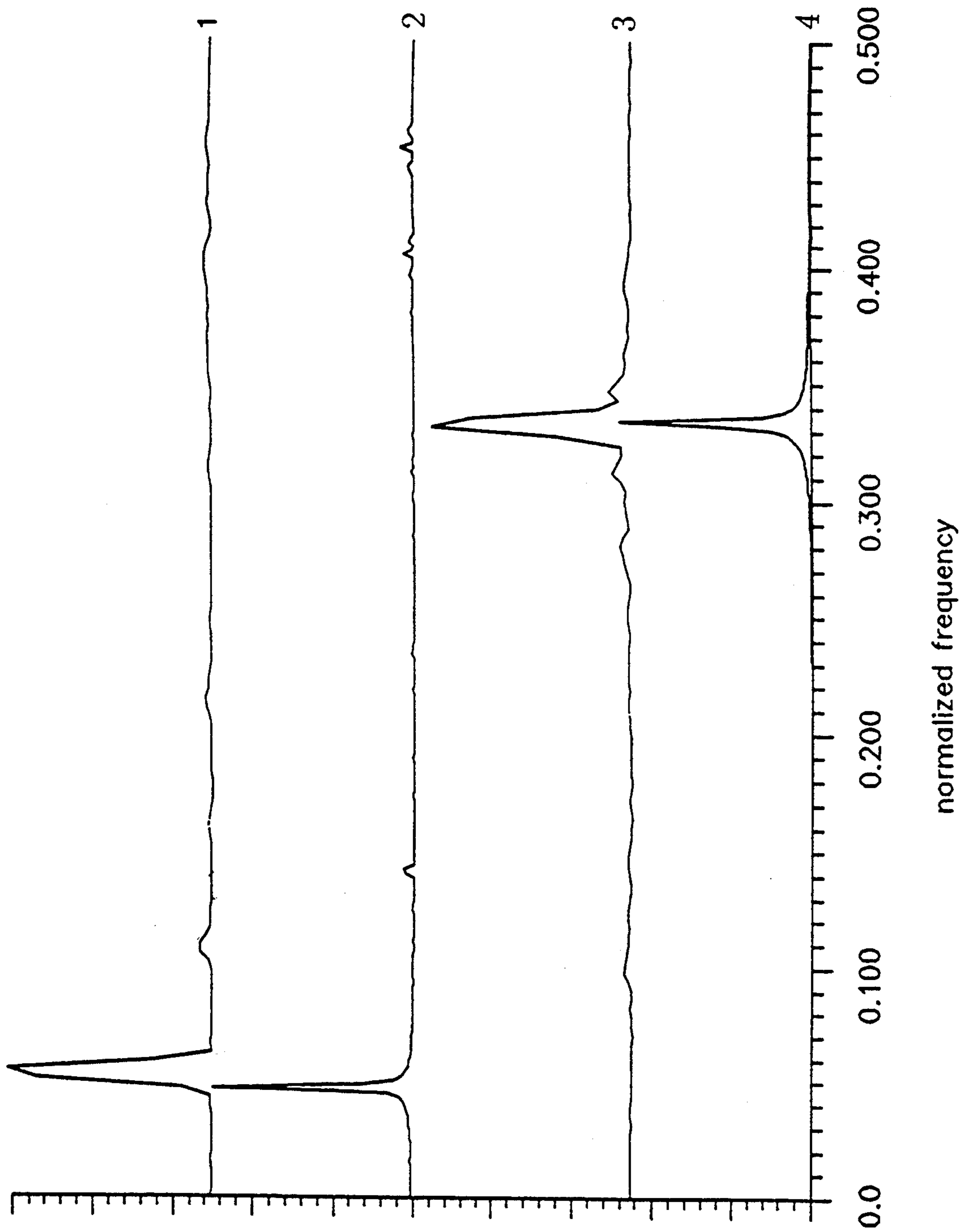
Experimental (1,3) and predicted (2,4) spectra for N=1.94 and 3.5
