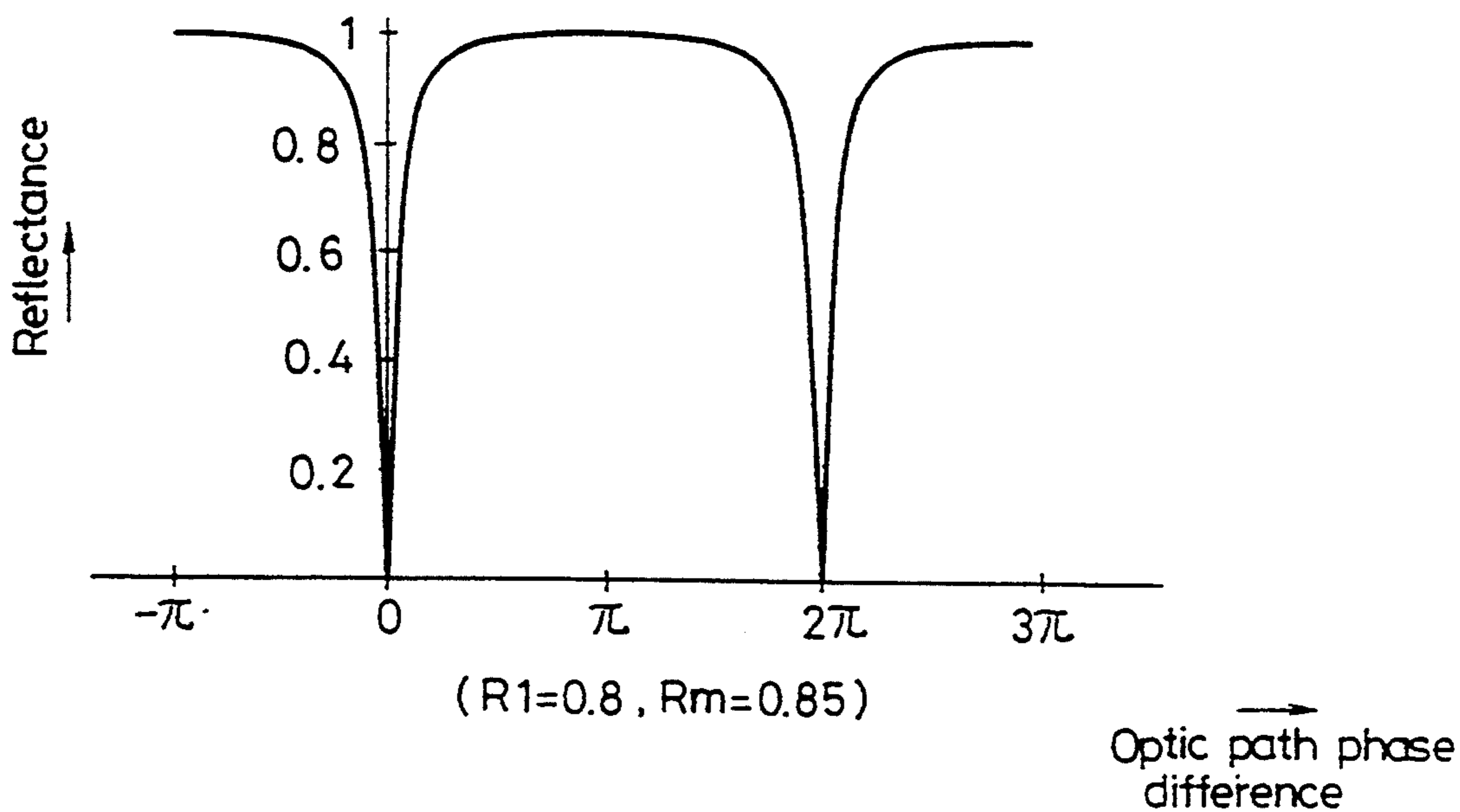
Graph of absolute value of reflectance r
