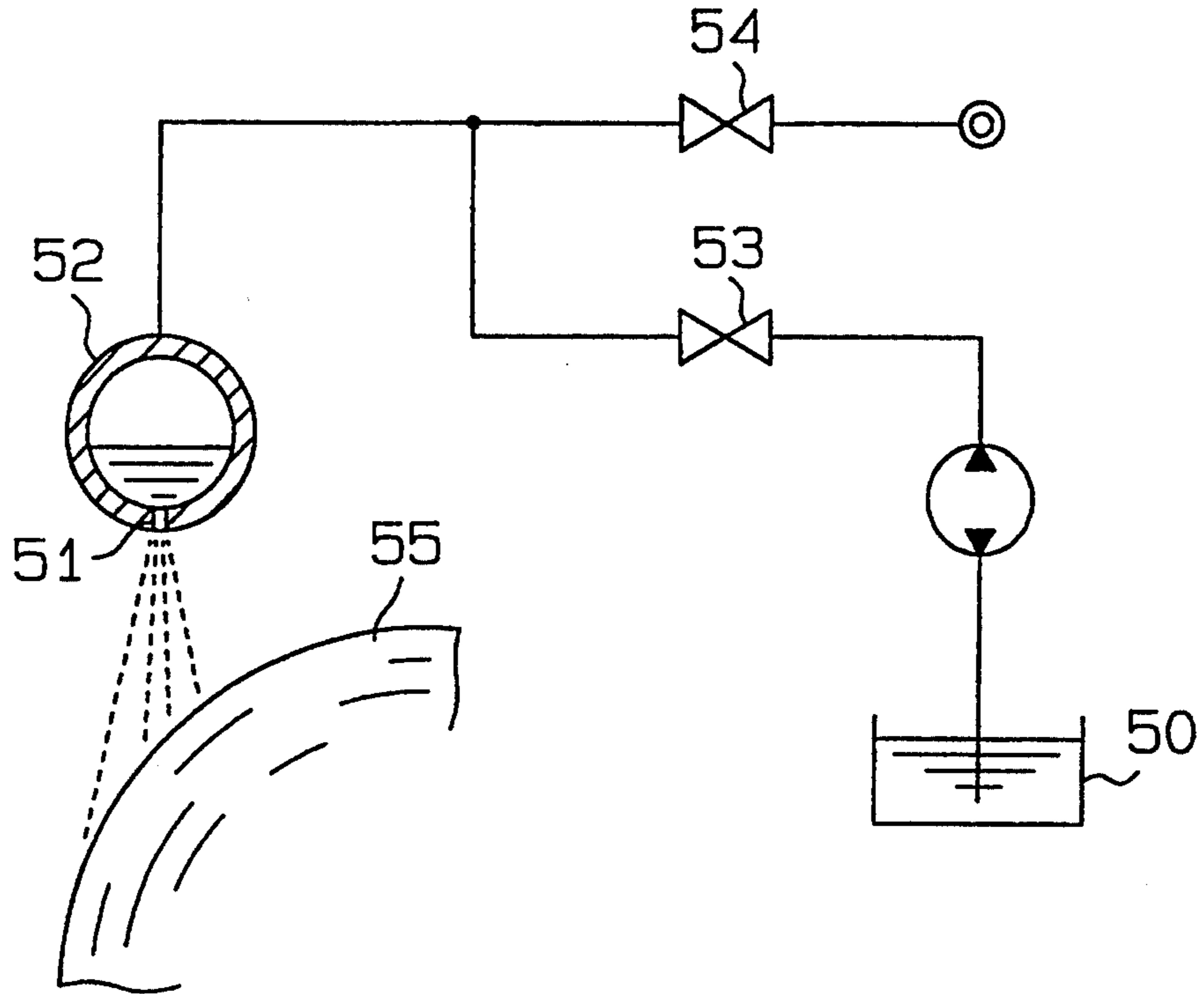
Fig. 9 (Prior Art)
