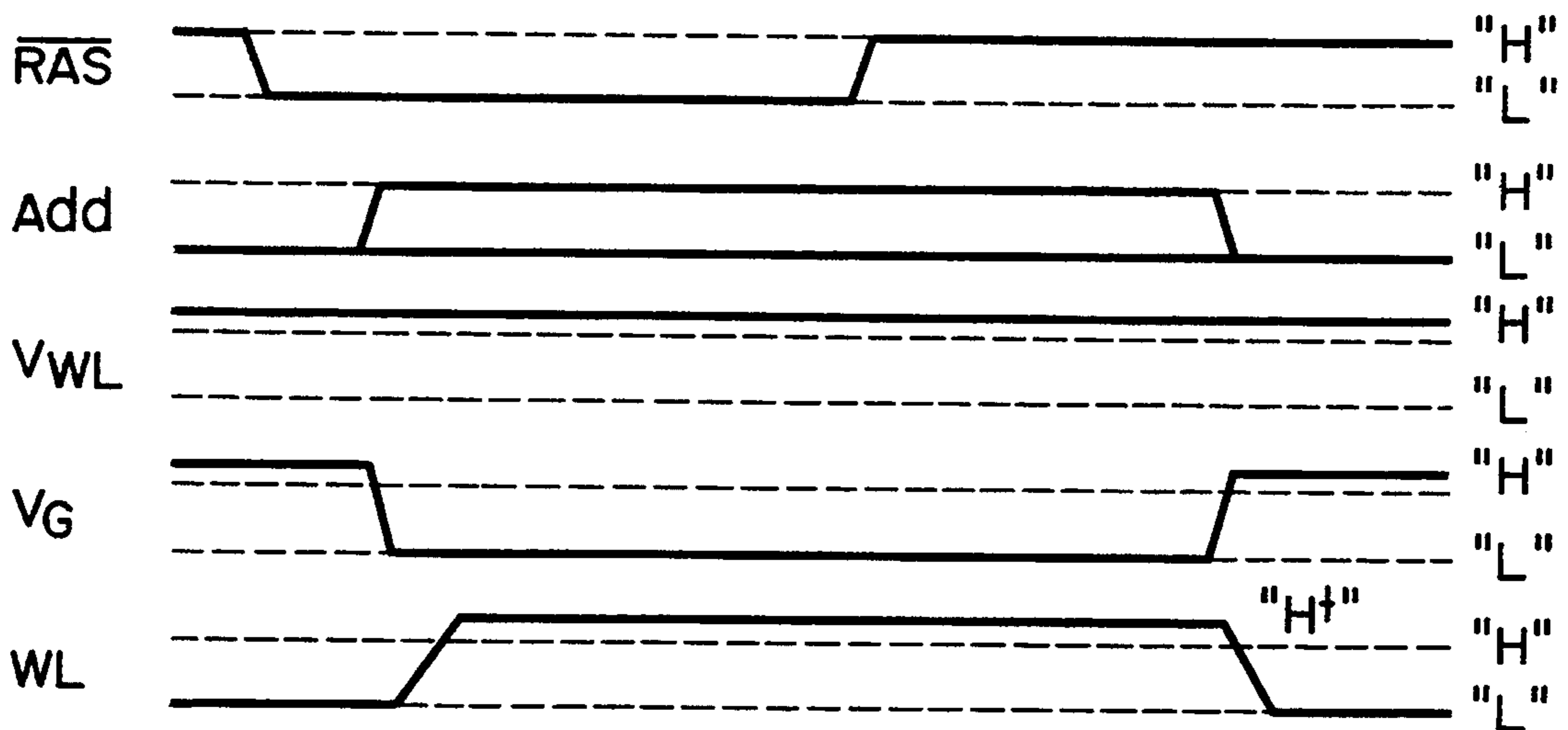
FIG. 4 (PRIOR ART)
