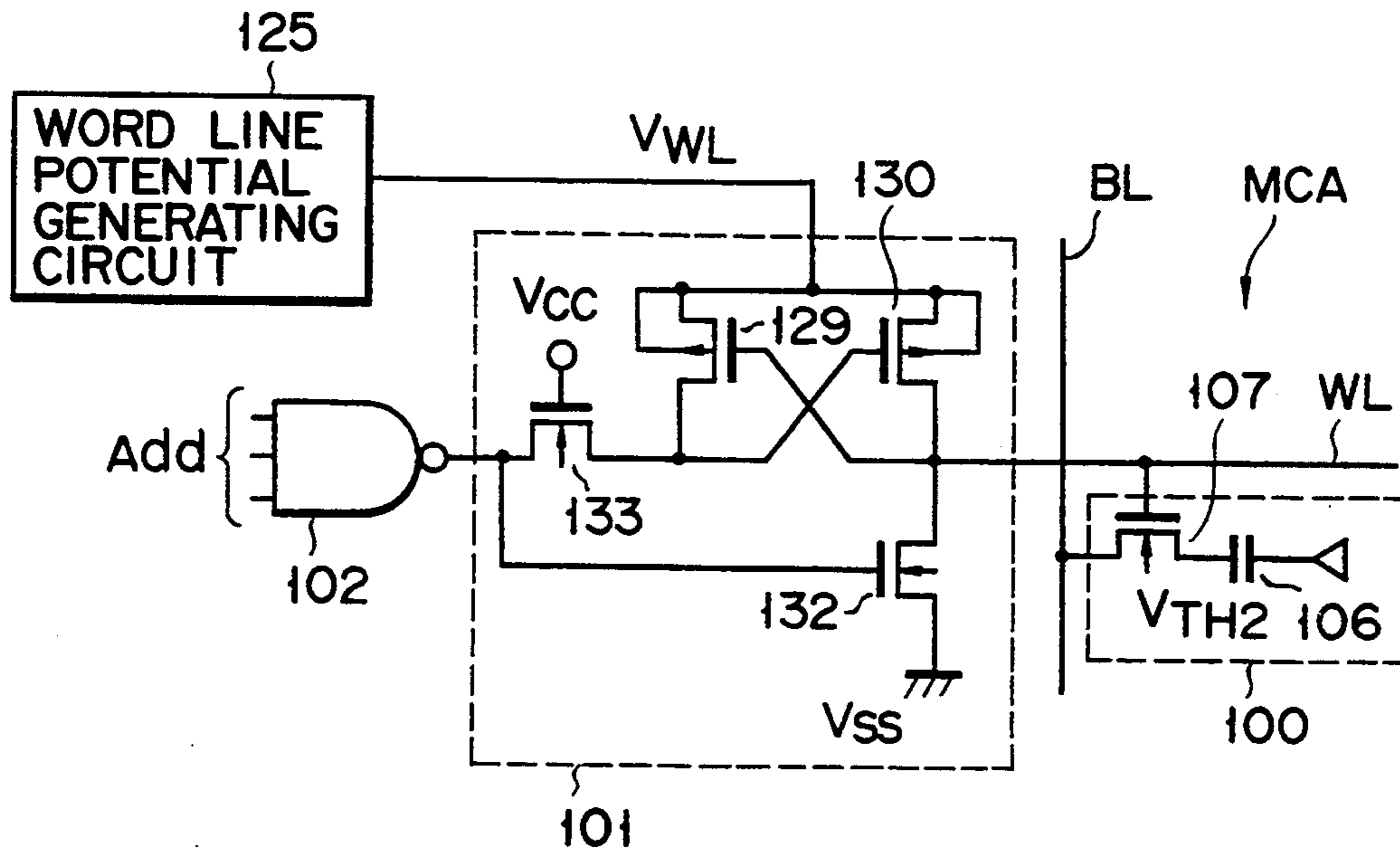
FIG. 3 (PRIOR ART)
