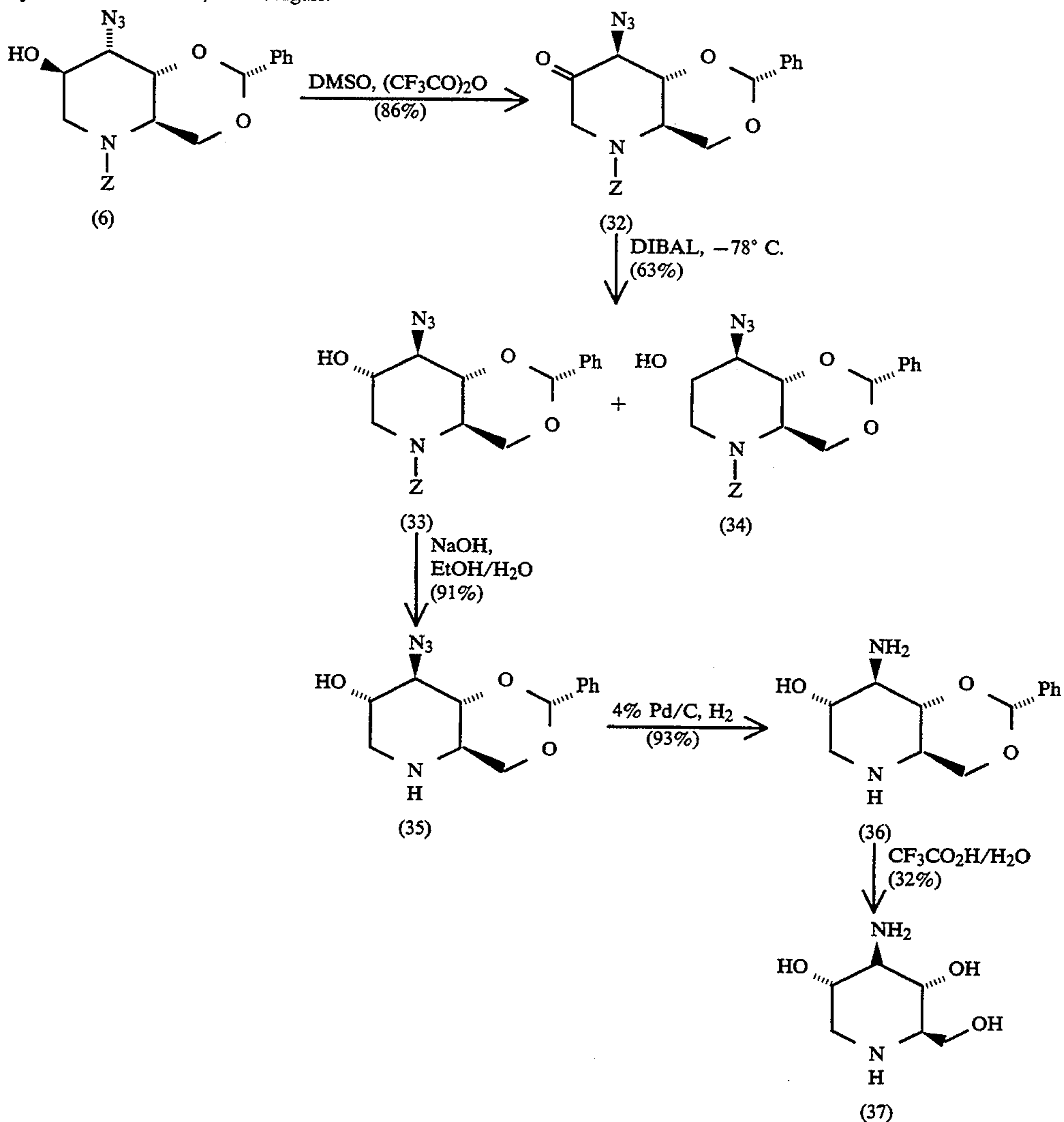
Scheme E: Synthesis of 3-amino-1,5-iminosugars.
