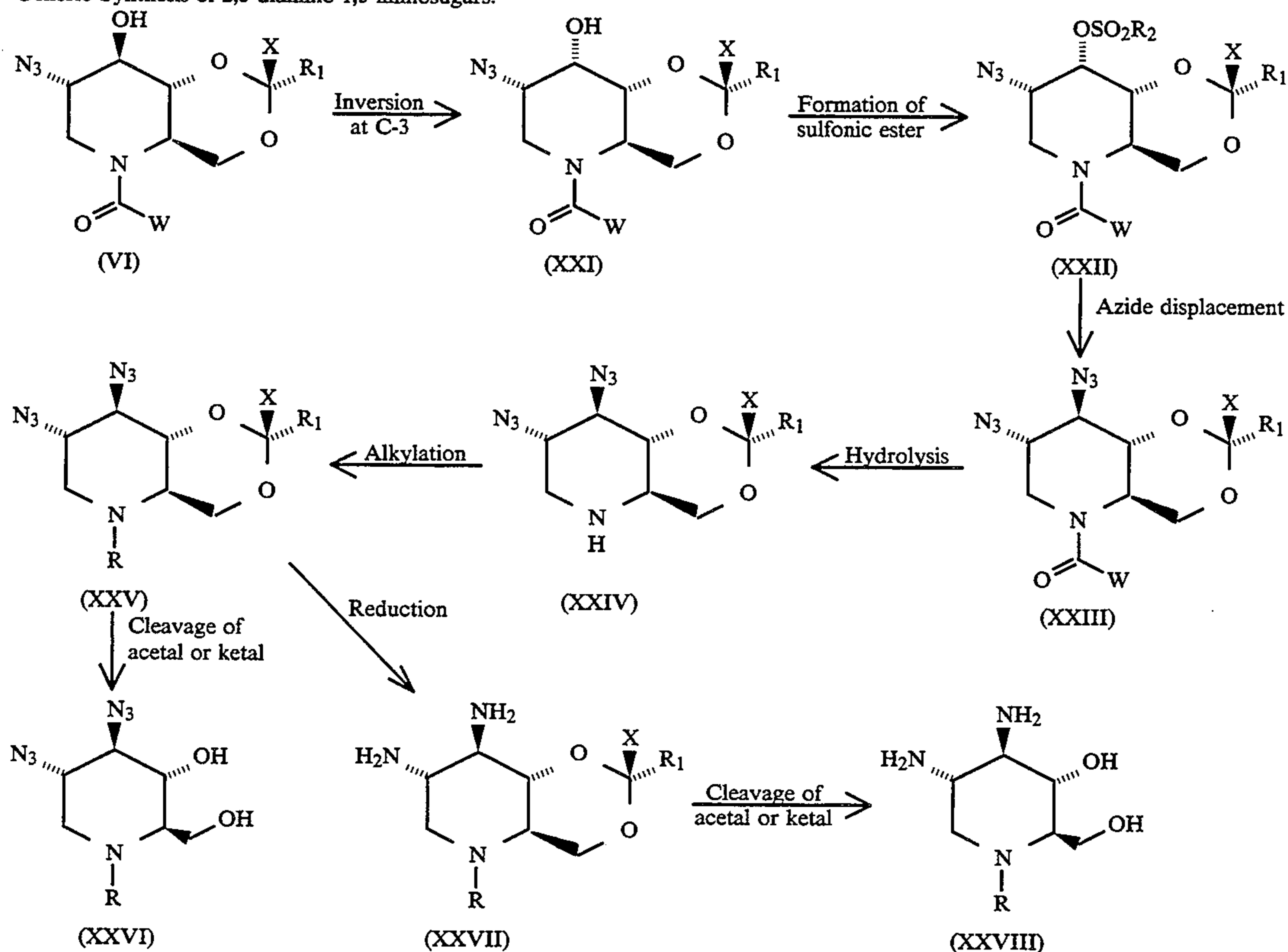
Scheme F: Generic Synthesis of 2,3-diamino-1,5-iminosugars.
