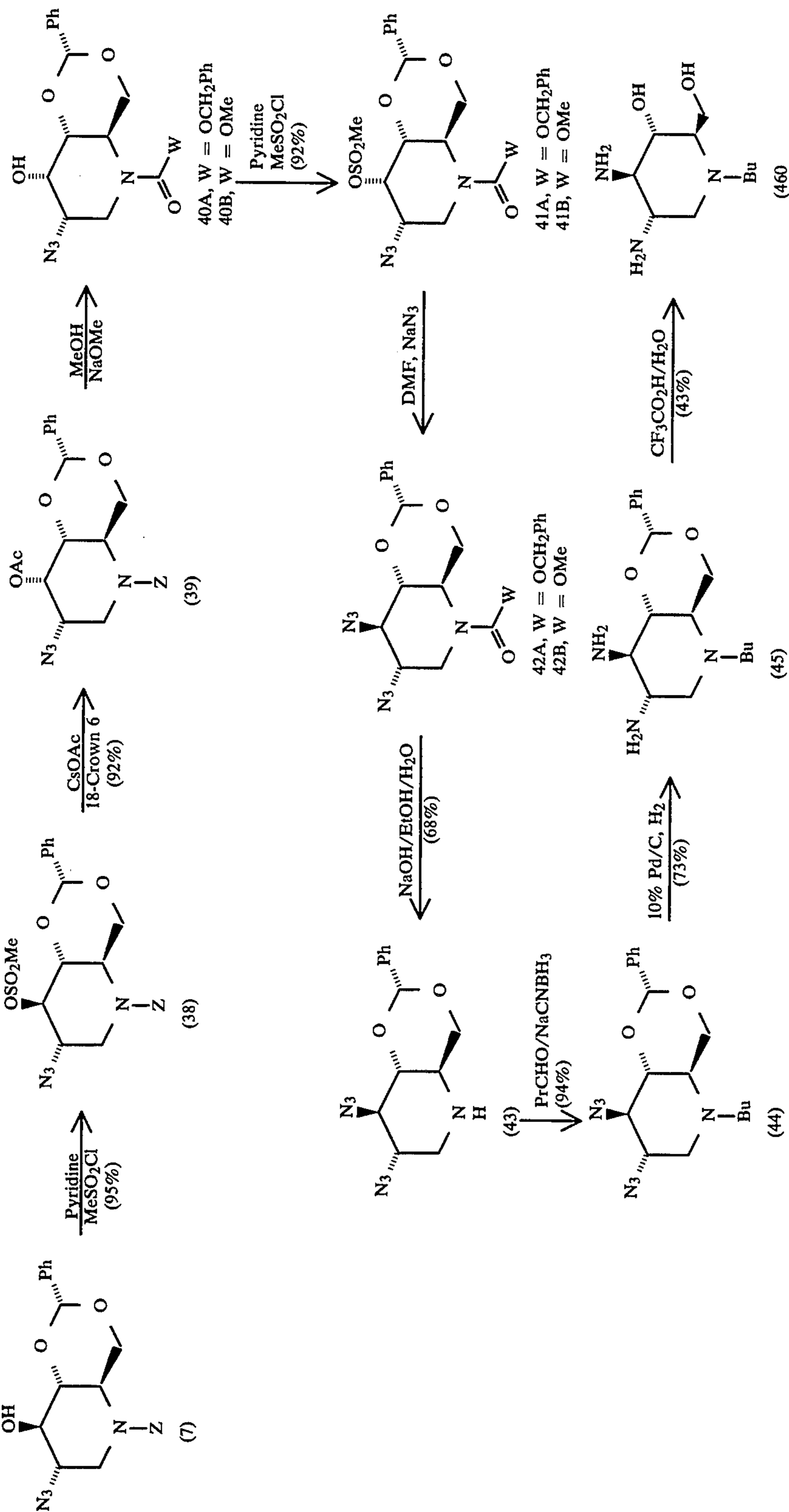
Scheme G: Synthesis of 2,3-diamino-1,5-iminosugars.
