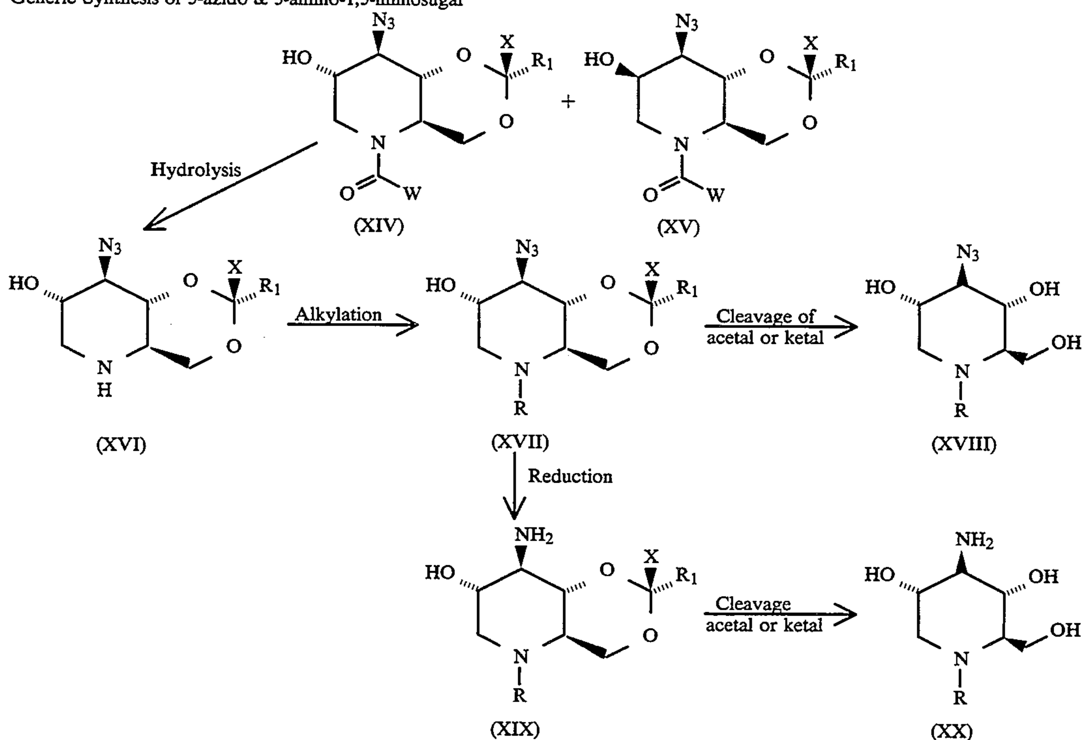
Scheme D: Generic Synthesis of 3-azido & 3-amino-1,5-iminosugar
