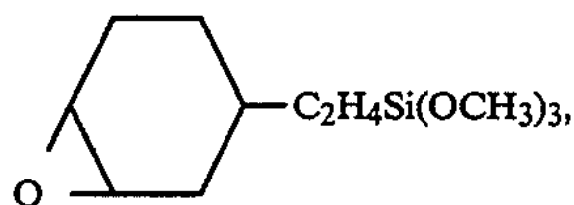
\gamma -glycidoxypropyltrimethoxysilane
