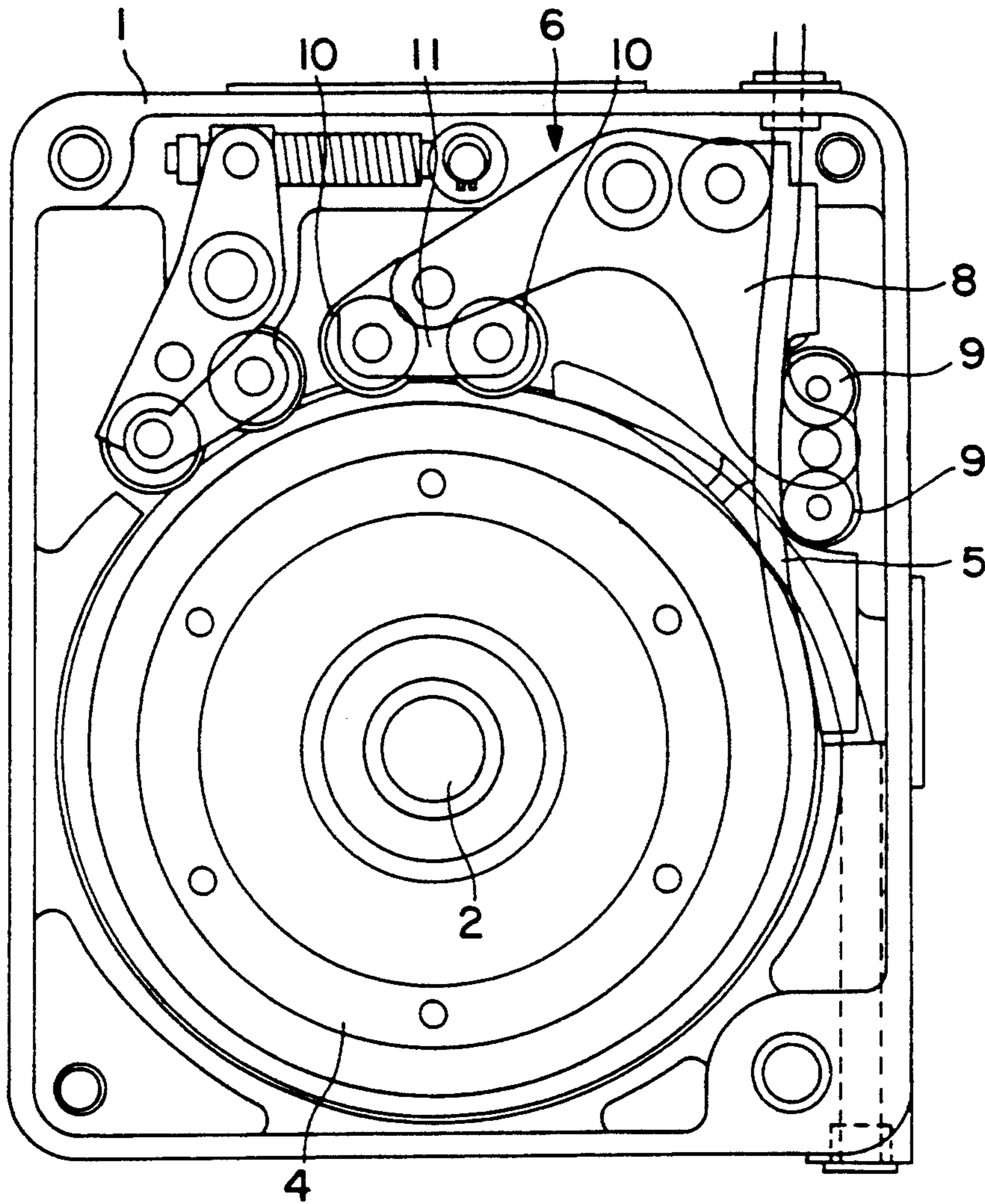
FIG. 7 PRIOR ART
