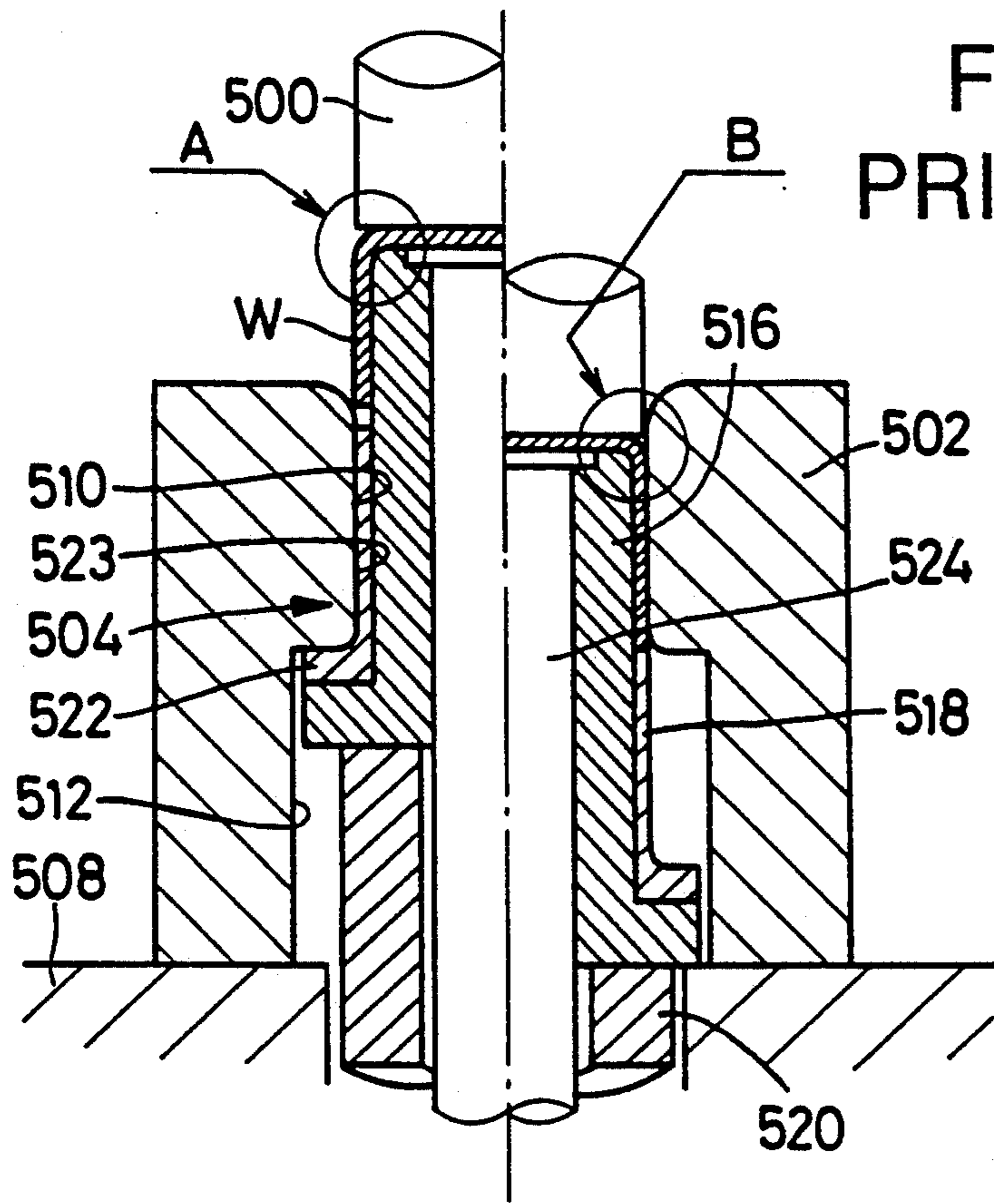
FIG. 22 PRIOR ART
