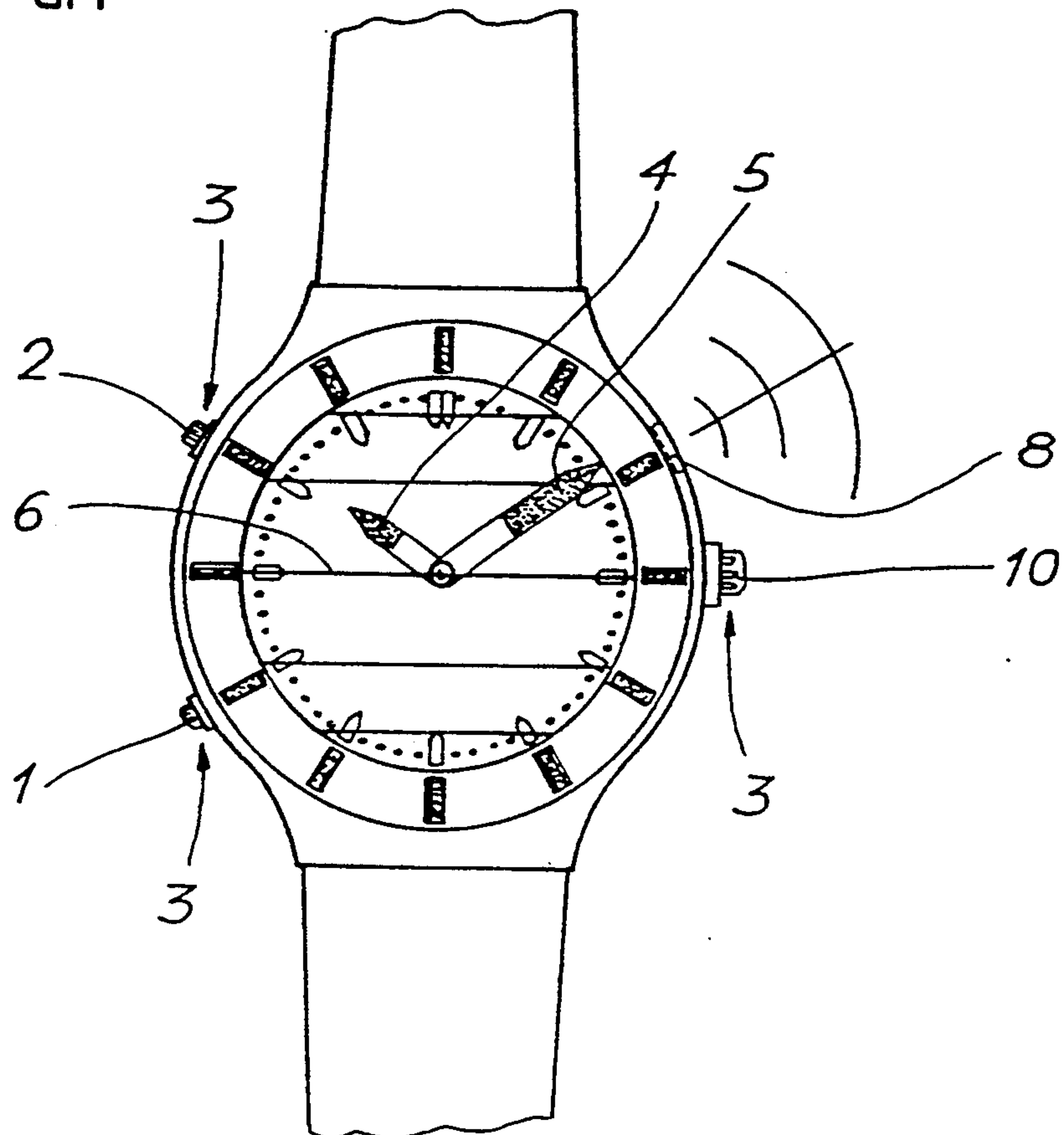
Fig.2 Prior art
