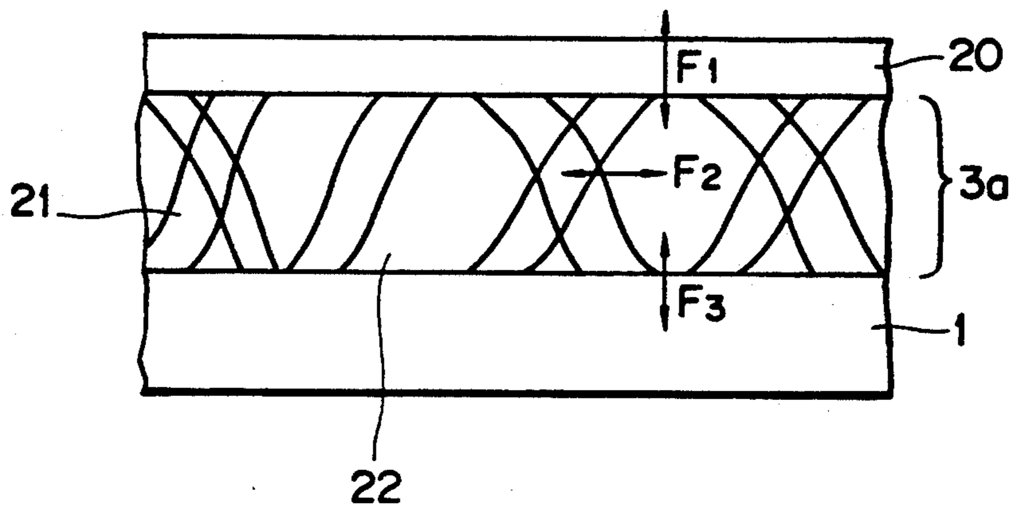
FIG. 5 (PRIOR ART)
