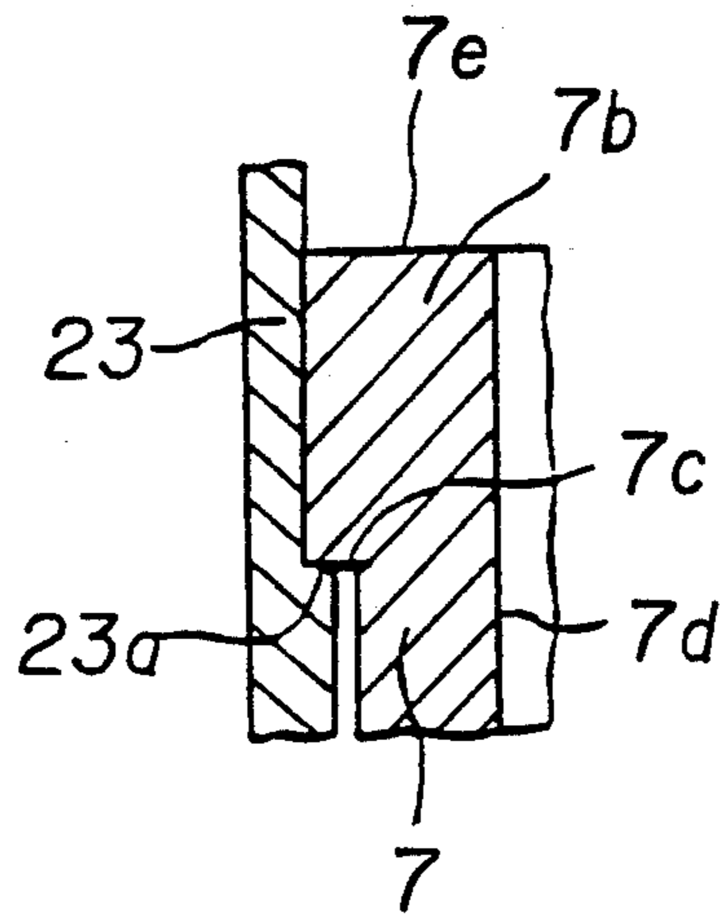
FIGURE 15 (PRIOR ART)
