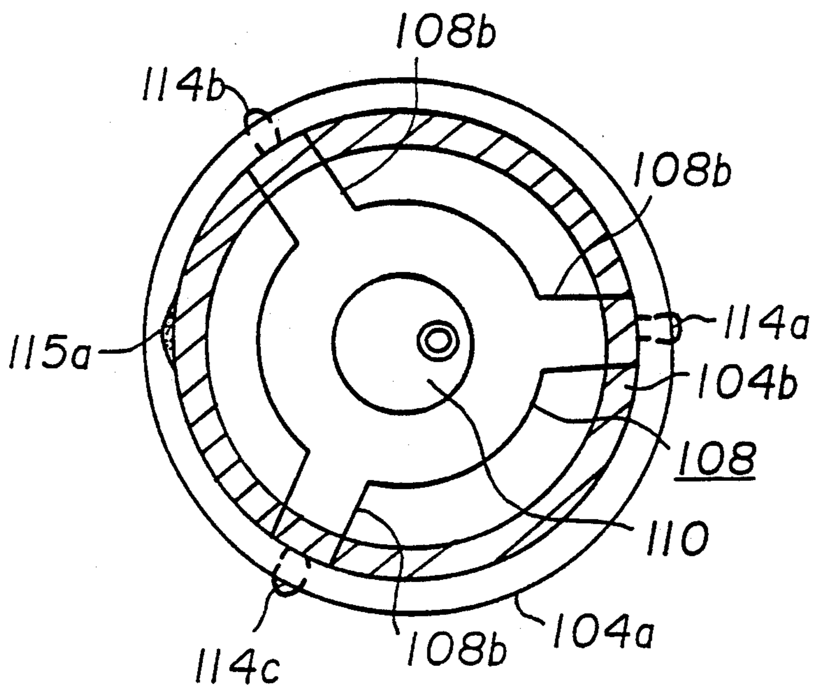
FIGURE 19 (PRIOR ART)
