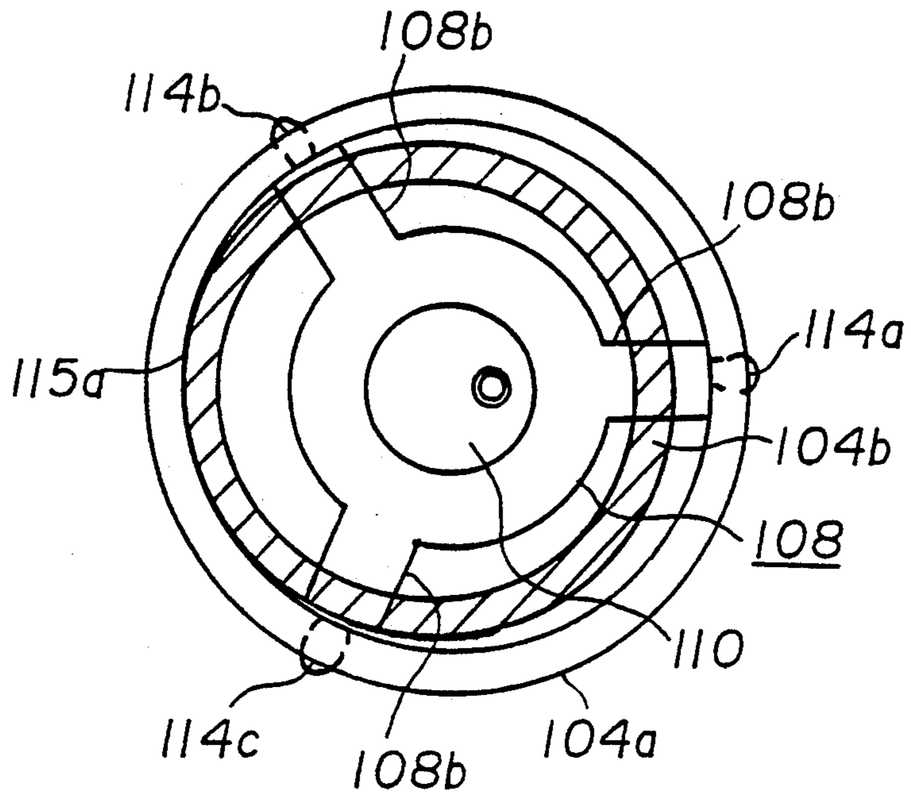
FIGURE 20 (PRIOR ART)
