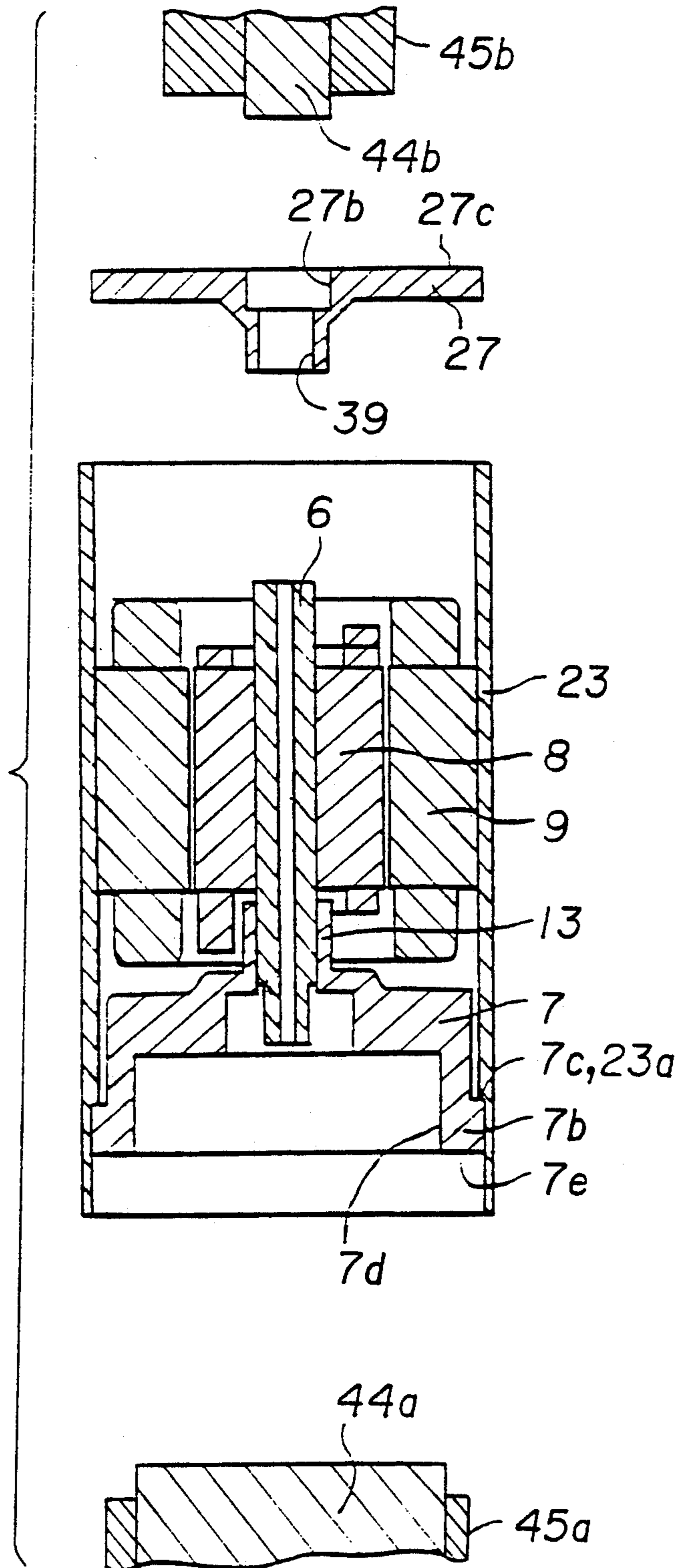
FIGURE 16 (PRIOR ART)
