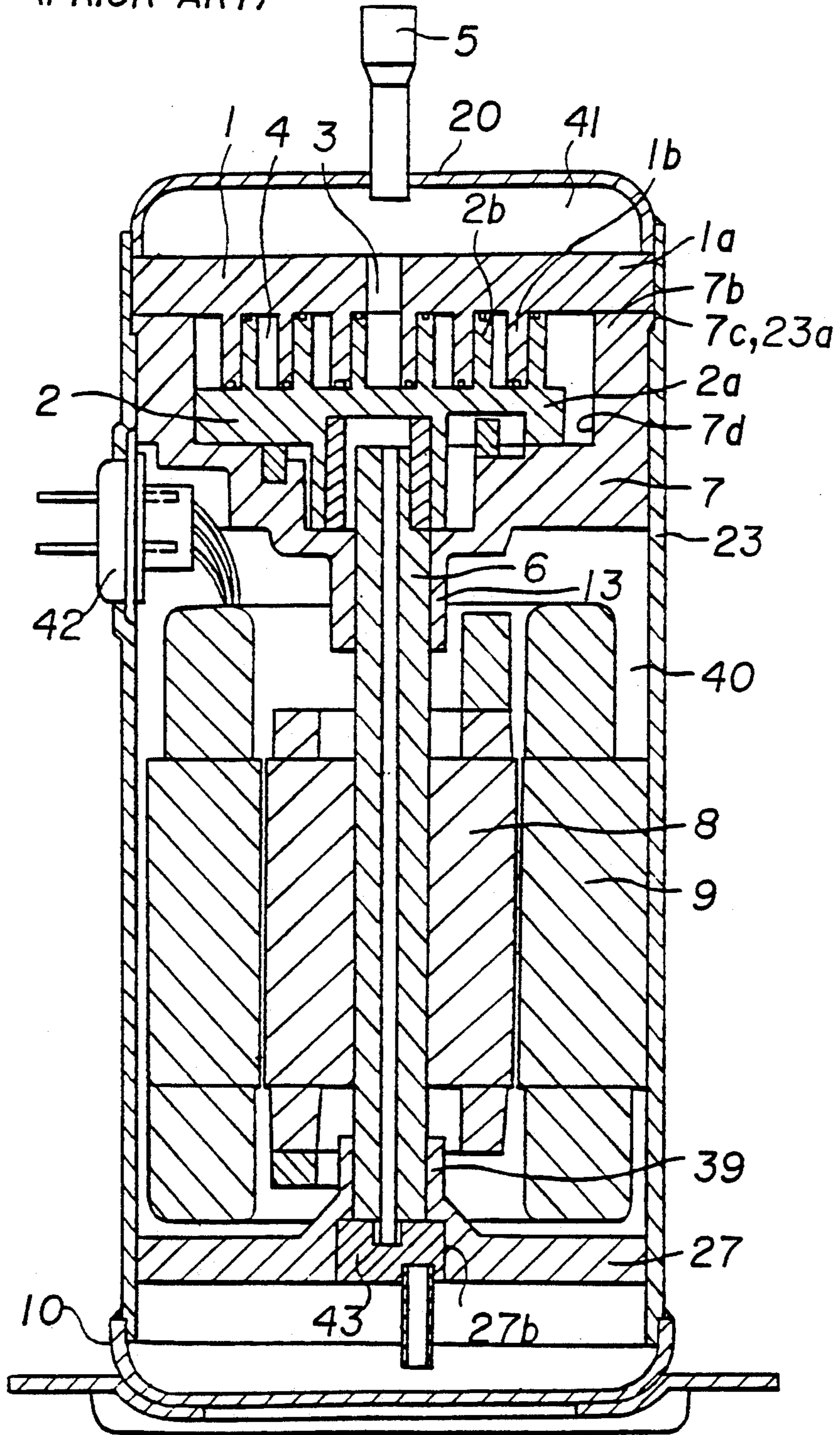
FIGURE 14 (PRIOR ART)
