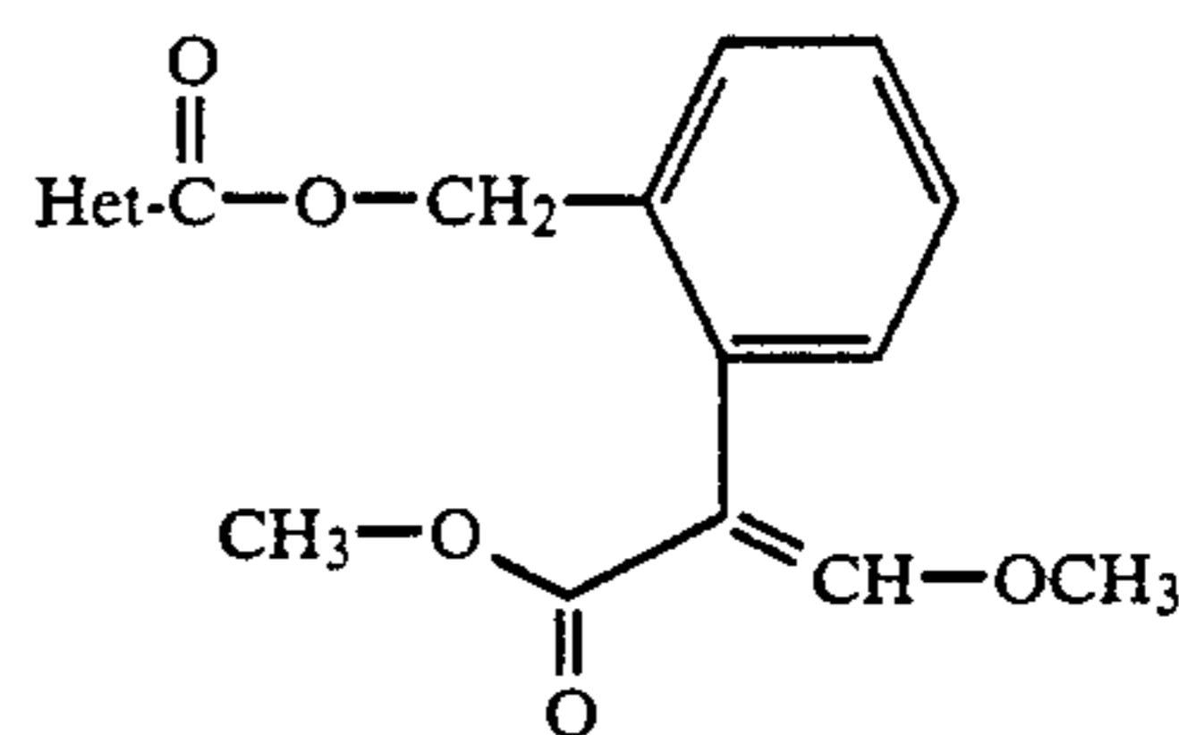
Compounds of the formula Ia (A = carbonyloxy, \text{R}^1 = \text{OCH}_3 , \text{R}^2 = \text{CH}_3 ) The configuration statement refers to the \beta -methoxyacrylate group.
