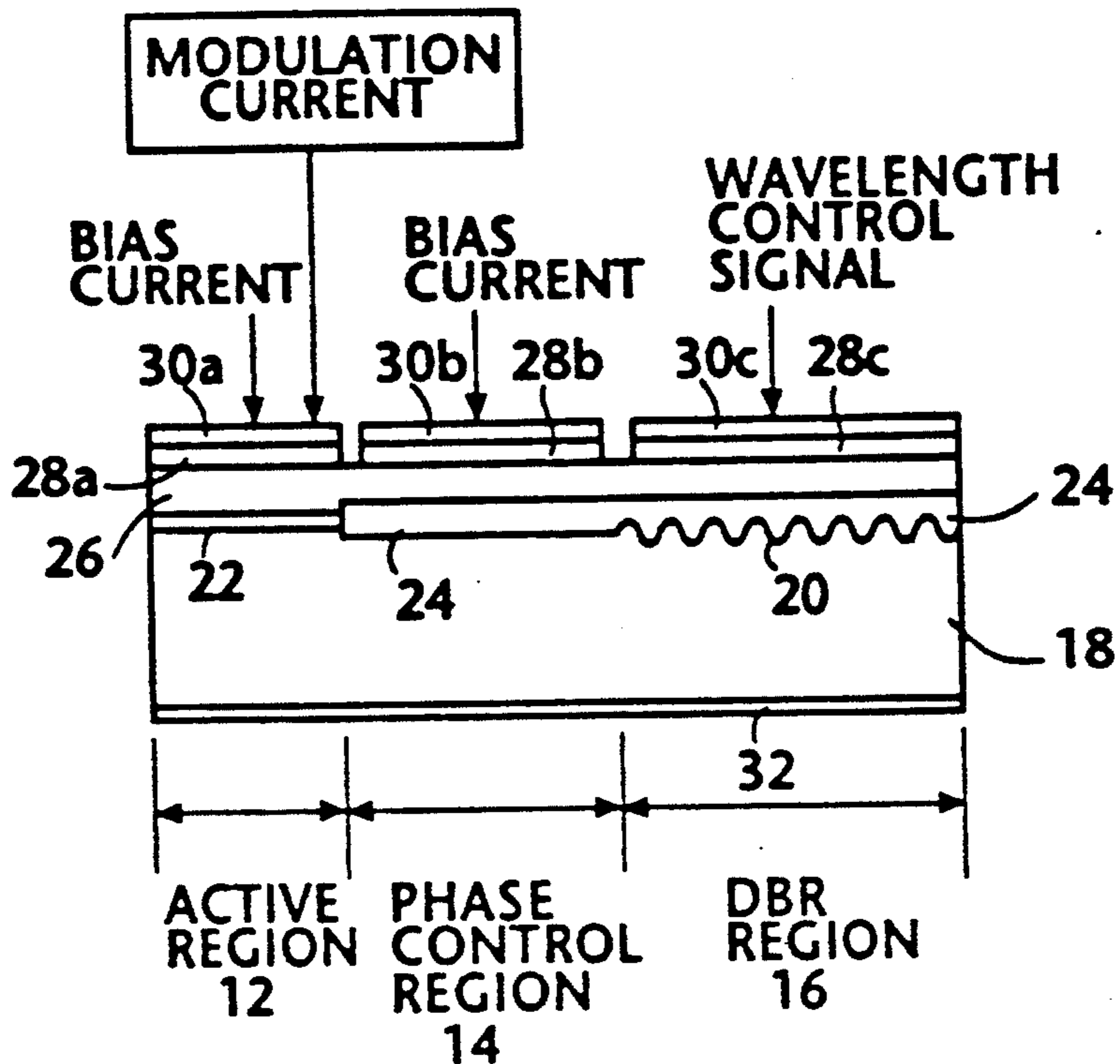
FIG. 2 (PRIOR ART)
