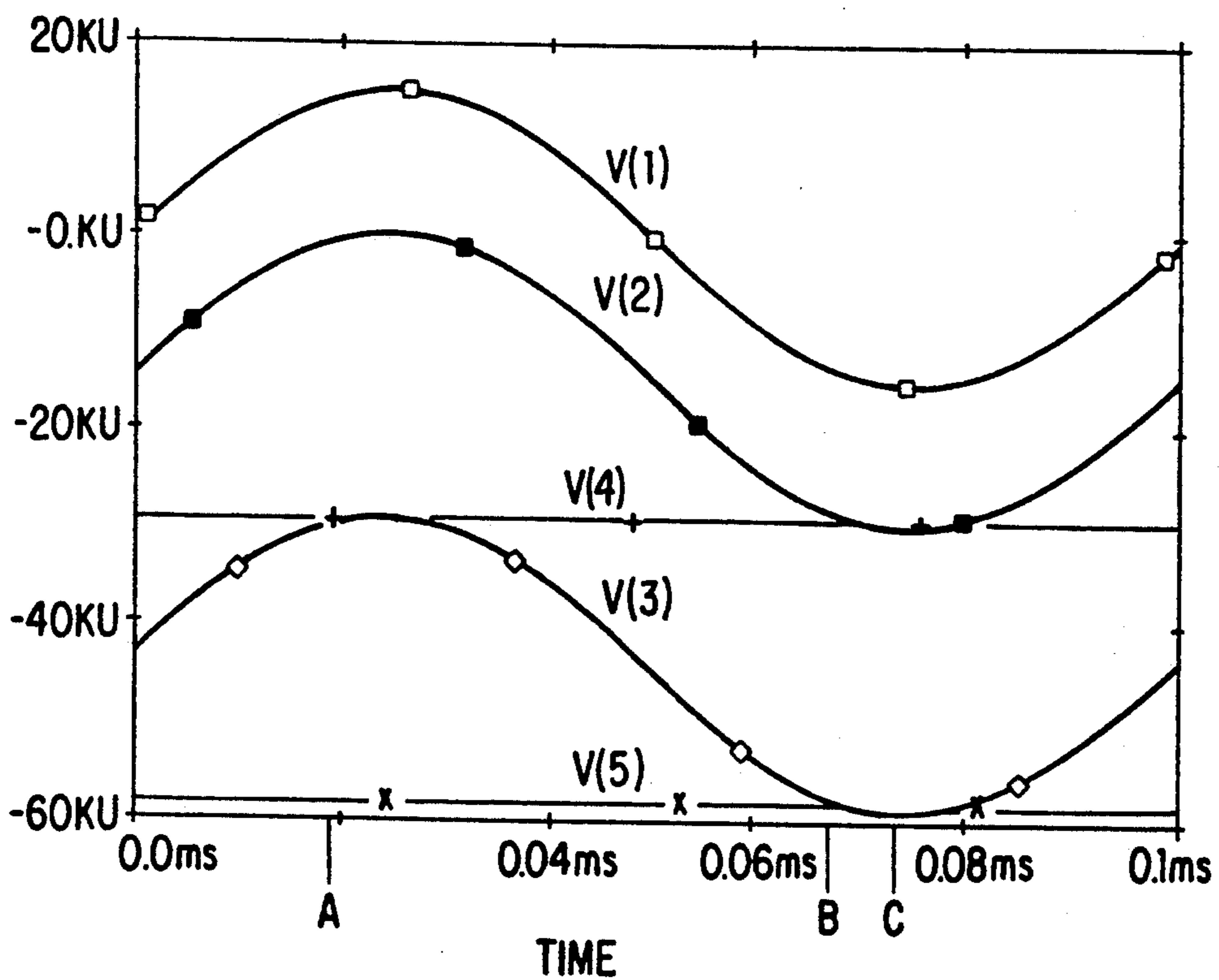
FIG. 3 PRIOR ART
