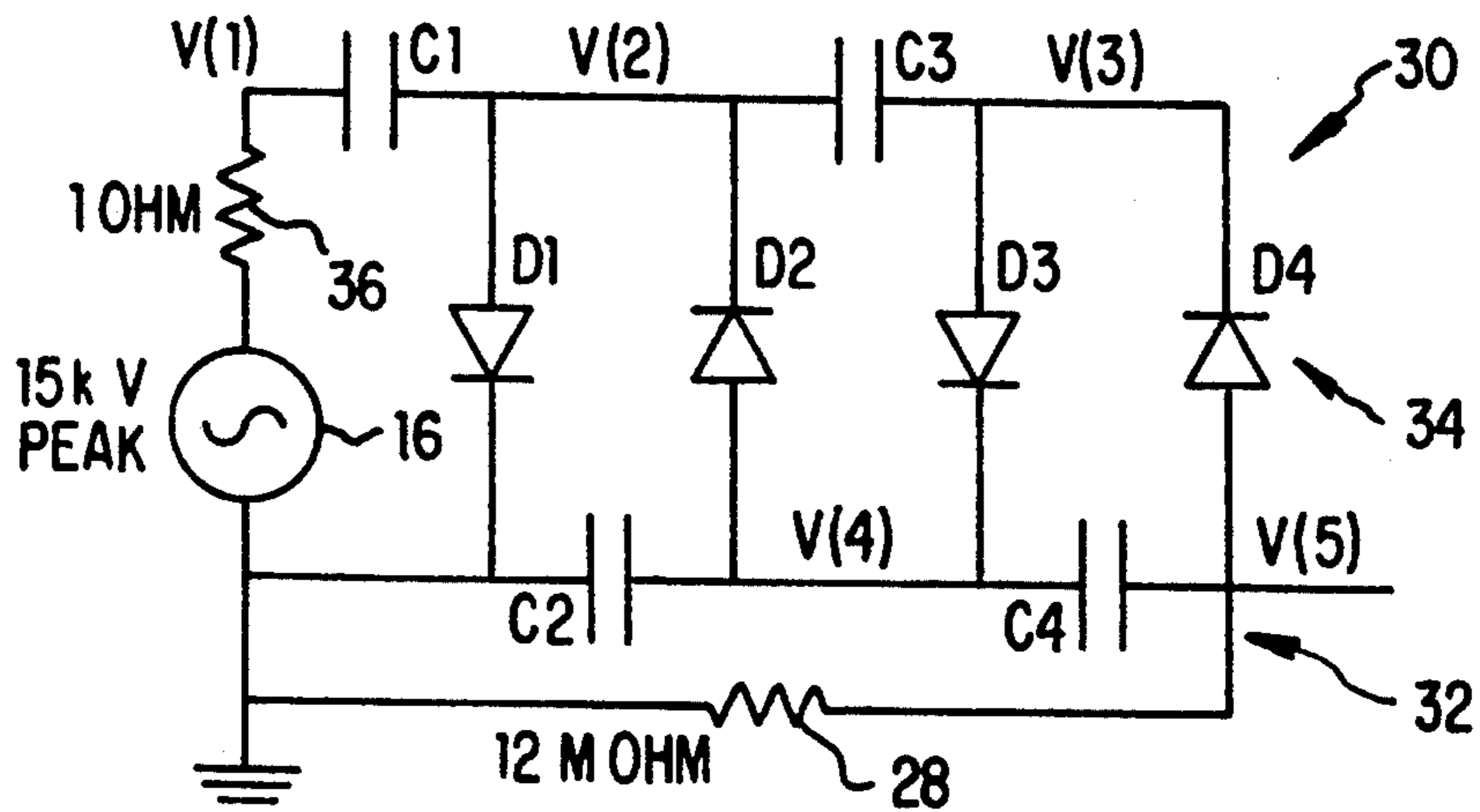
FIG. 2 PRIOR ART
