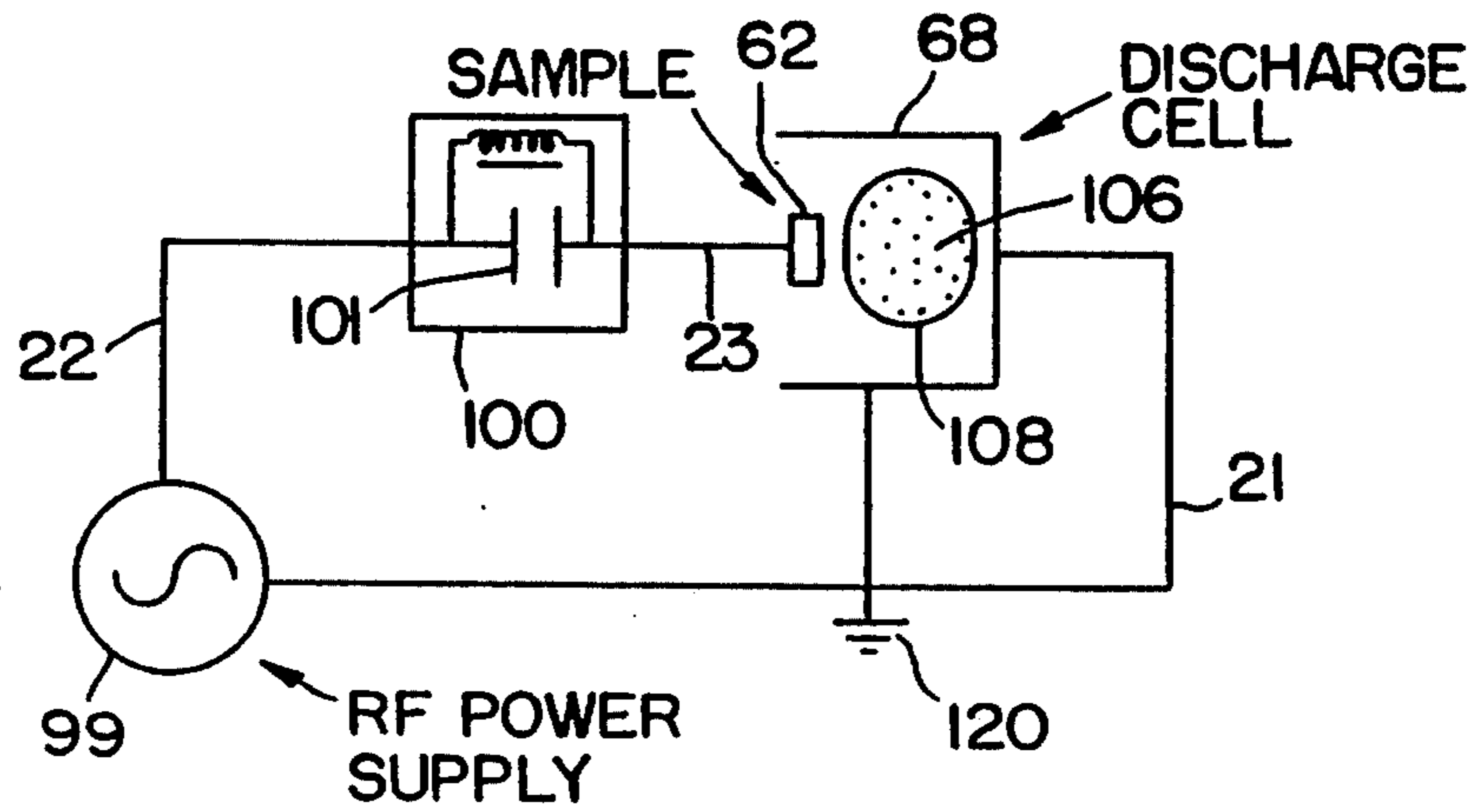
FIG. 3 PRIOR ART
