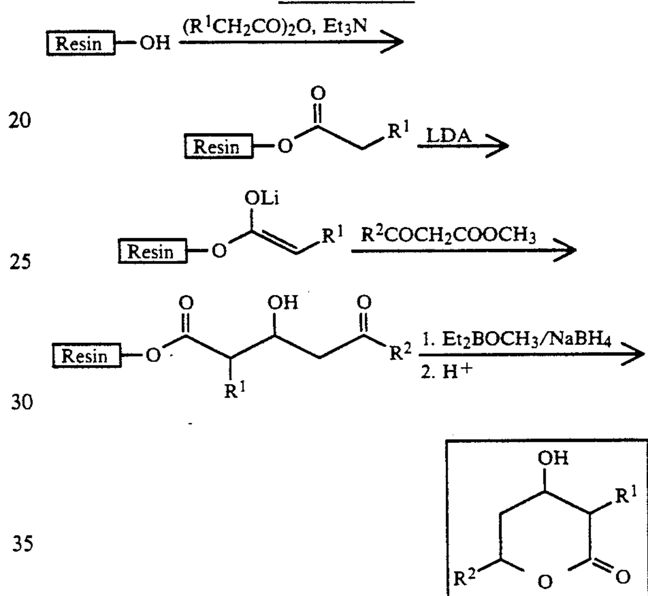
SCHEME 9
