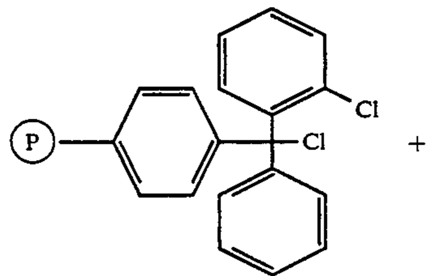
SCHEME 13
