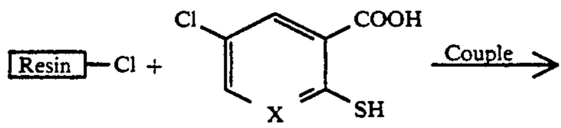
SCHEME 11
