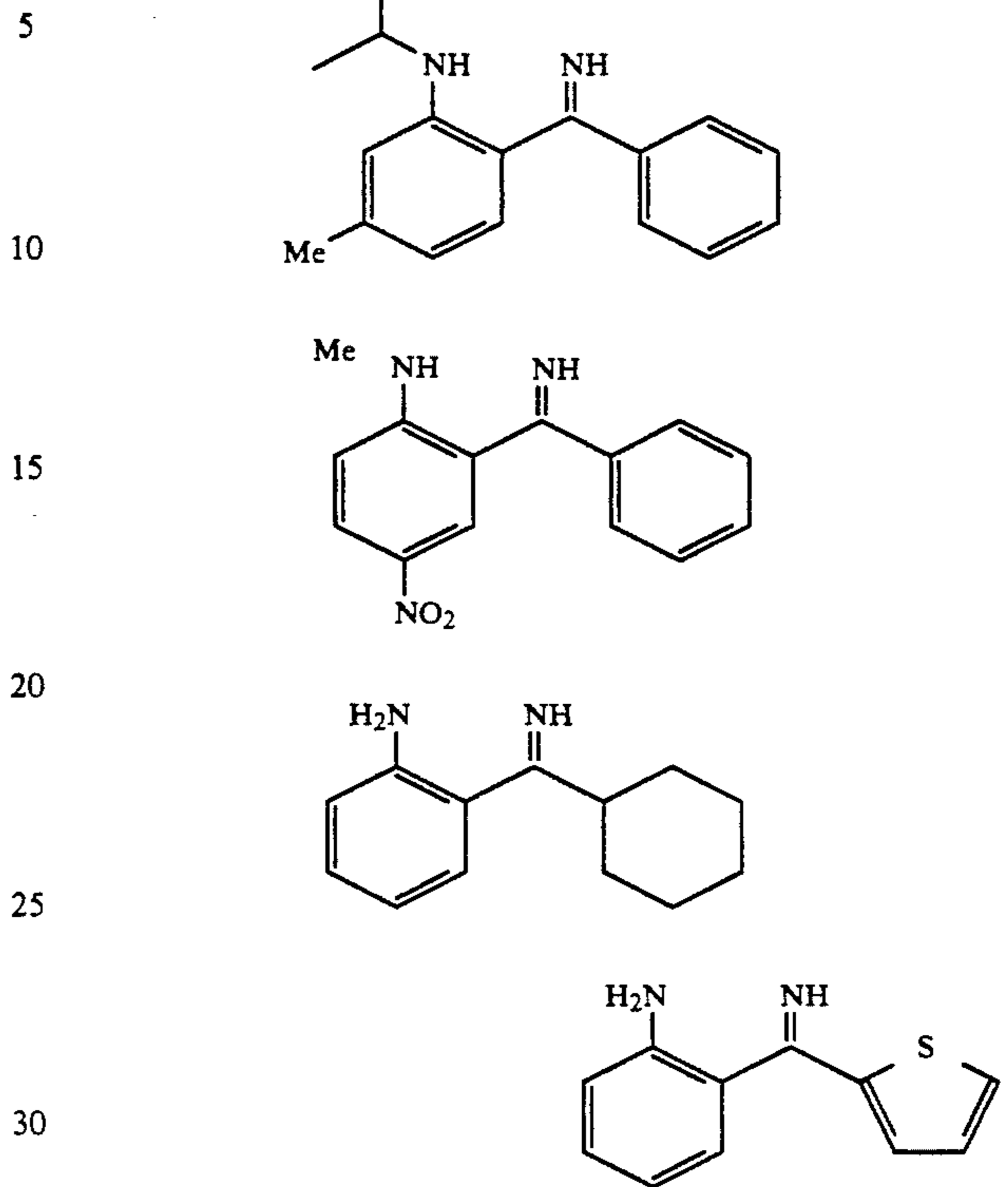
-continued SCHEME 3
