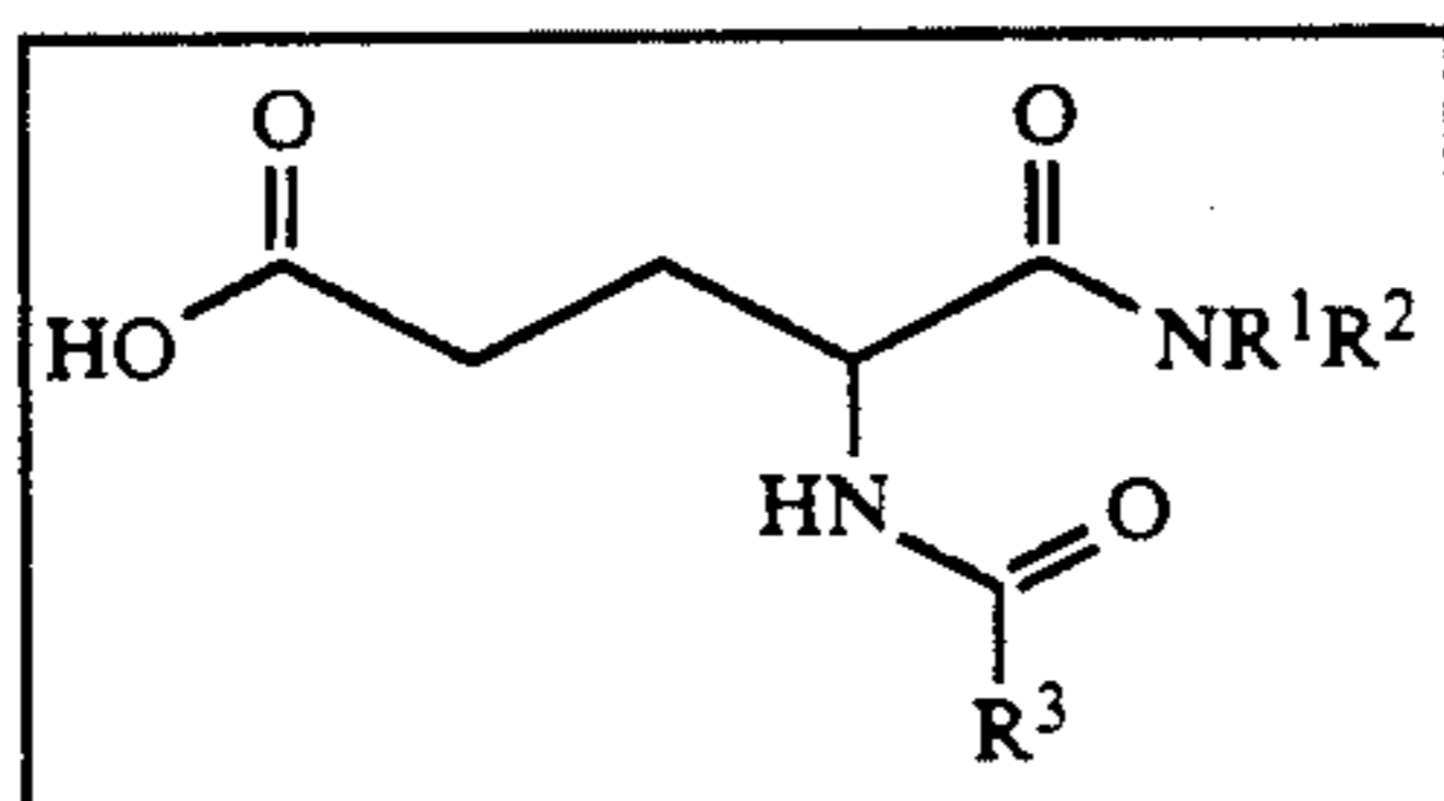
SCHEME 7
