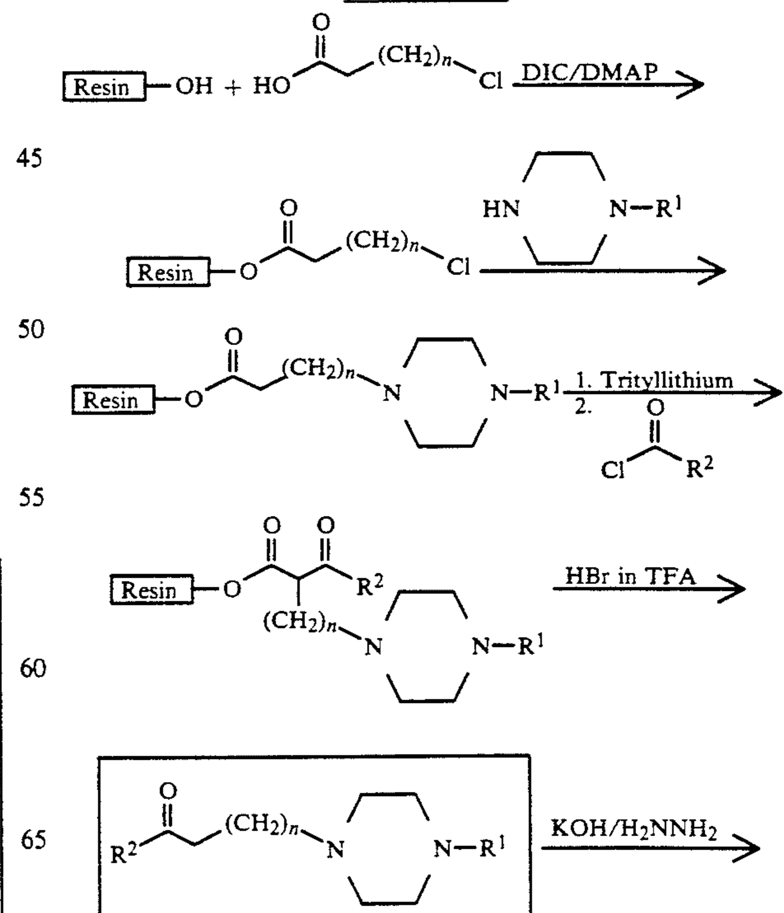
SCHEME 10
