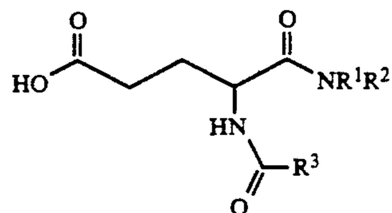
(R)-4-BENZAMIDO-5-OXOPENTANOIC ACIDS
