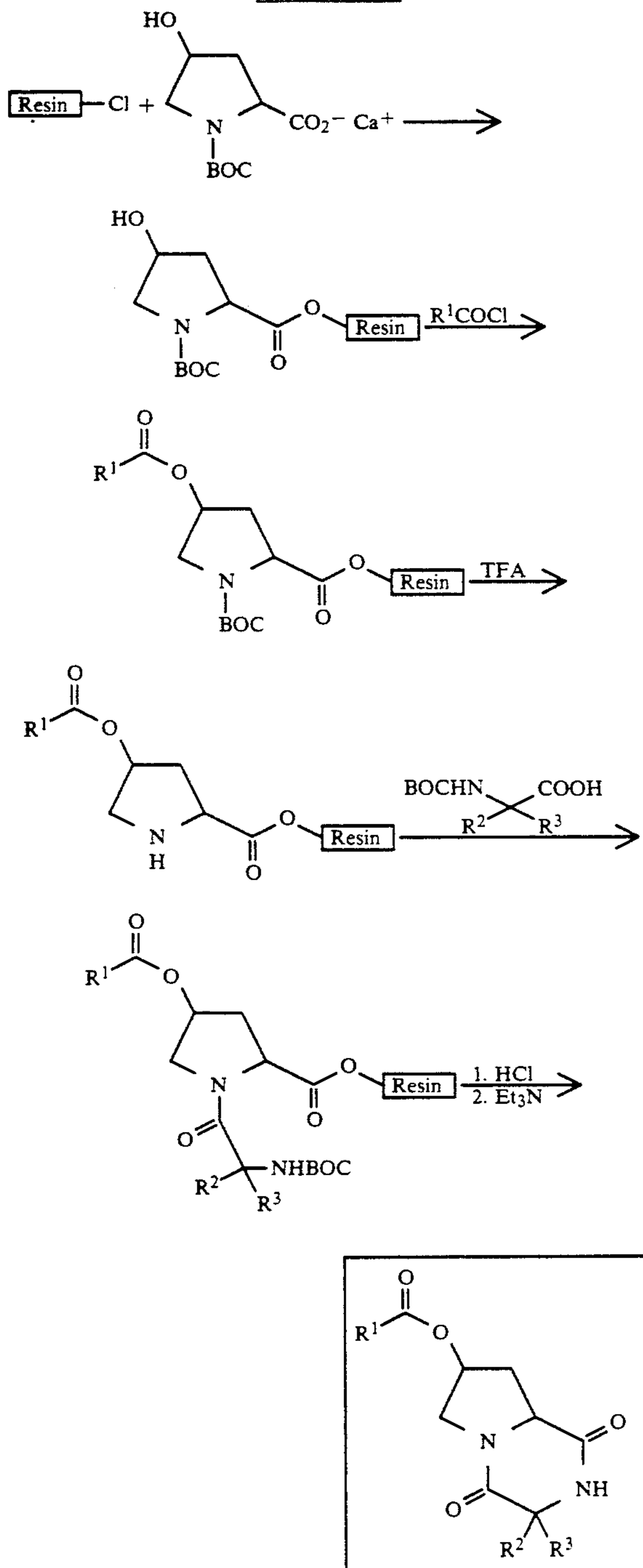
SCHEME 8
