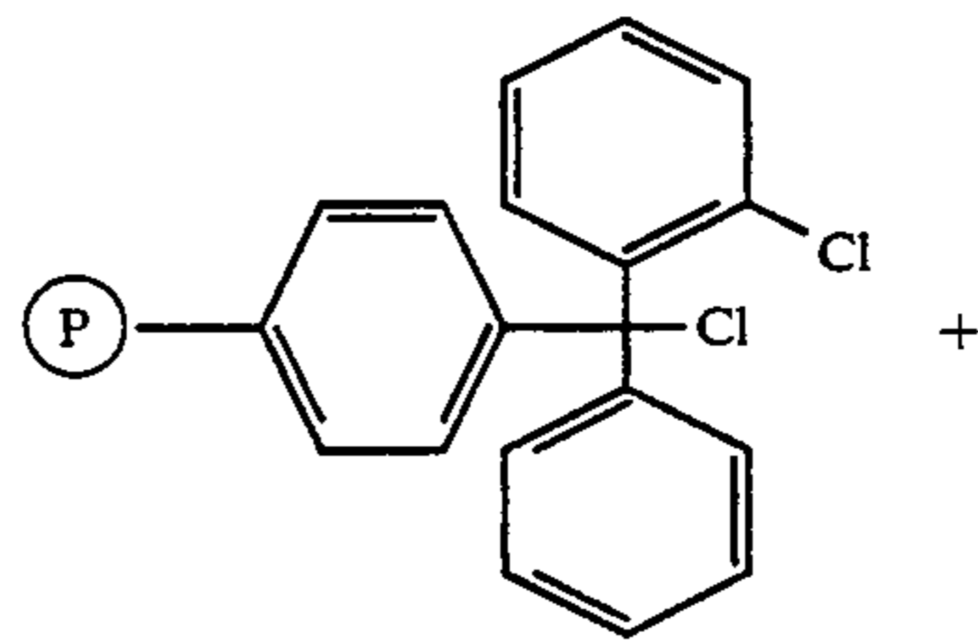
SCHEME 13
