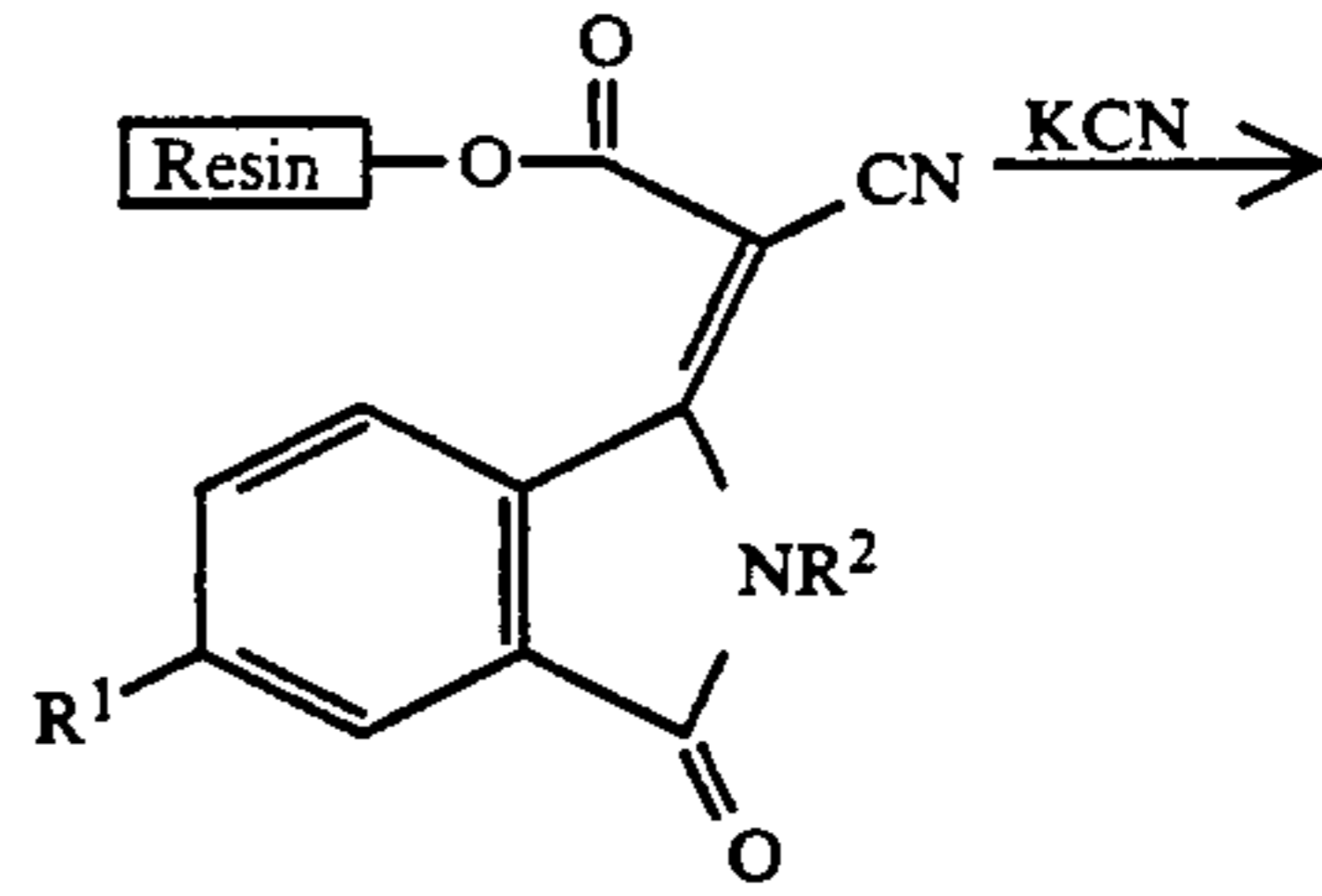
-continued SCHEME 12
