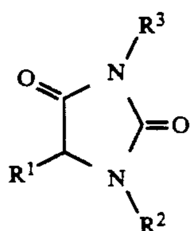
N 2 -Substituted Hydantoins
