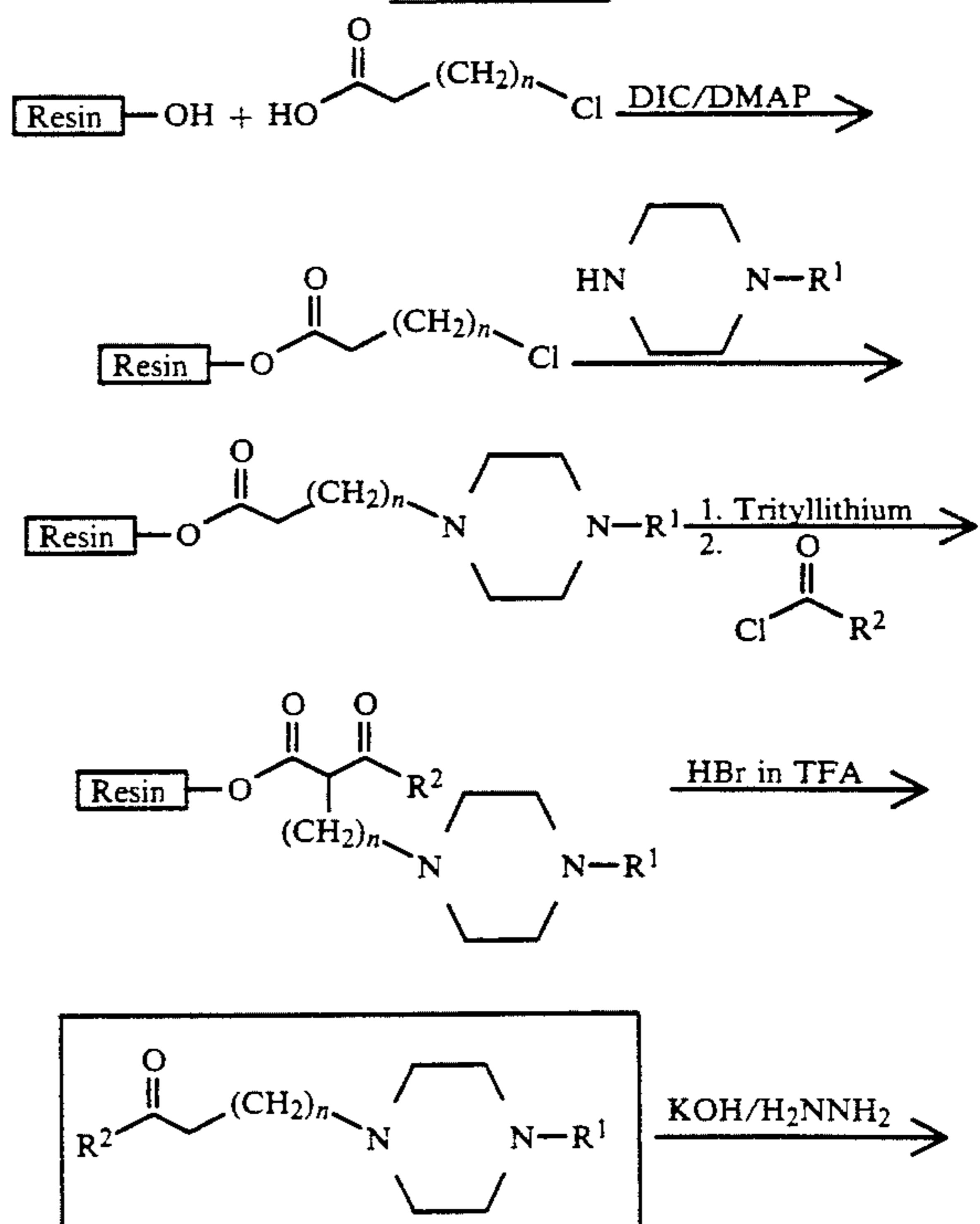
SCHEME 10
