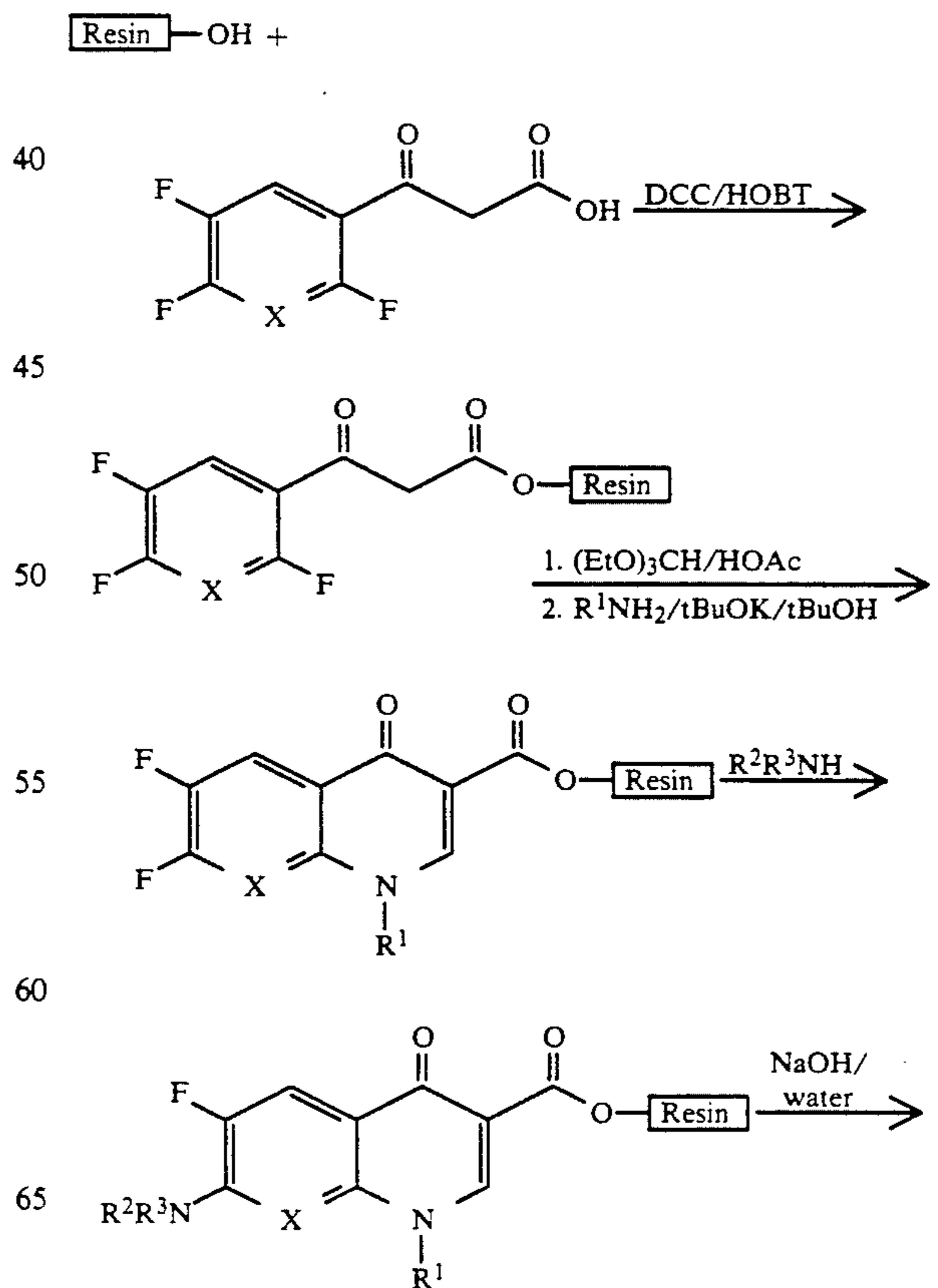
SCHEME 4
