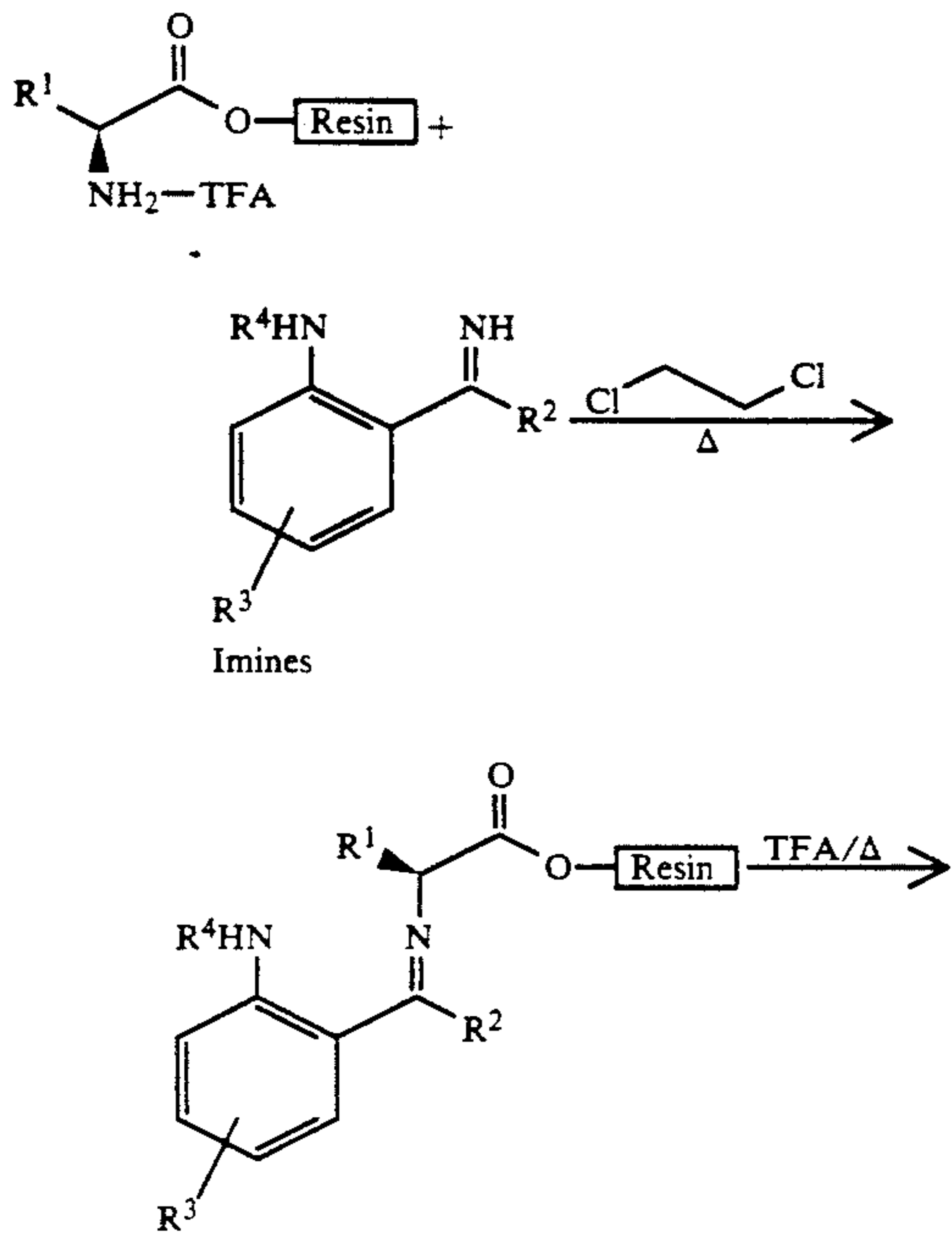
SCHEME 3
