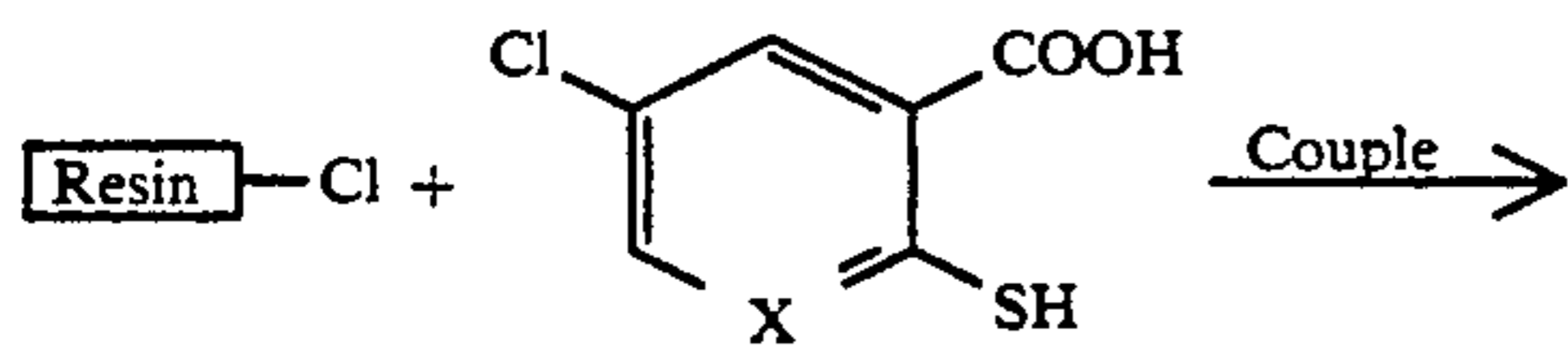
SCHEME 11
