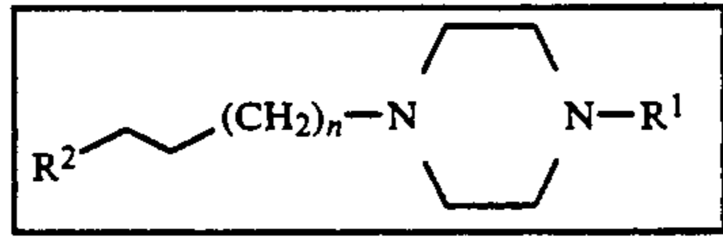
-continued SCHEME 10
