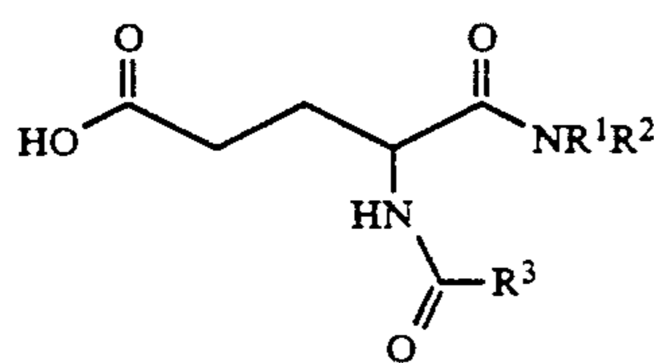
(R)-4-BENZAMIDO-5-OXOPENTANOIC ACIDS
