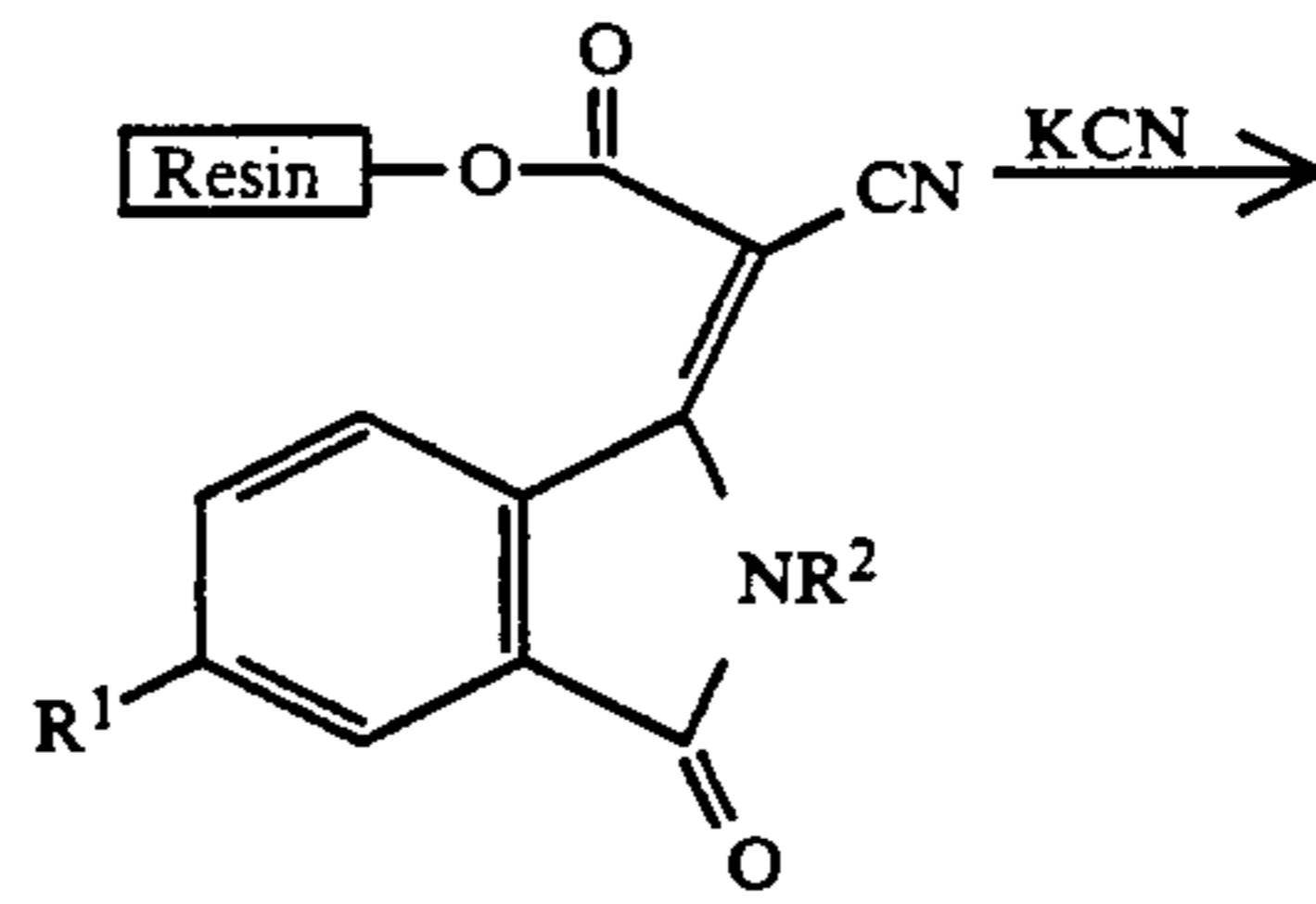
-continued SCHEME 12
