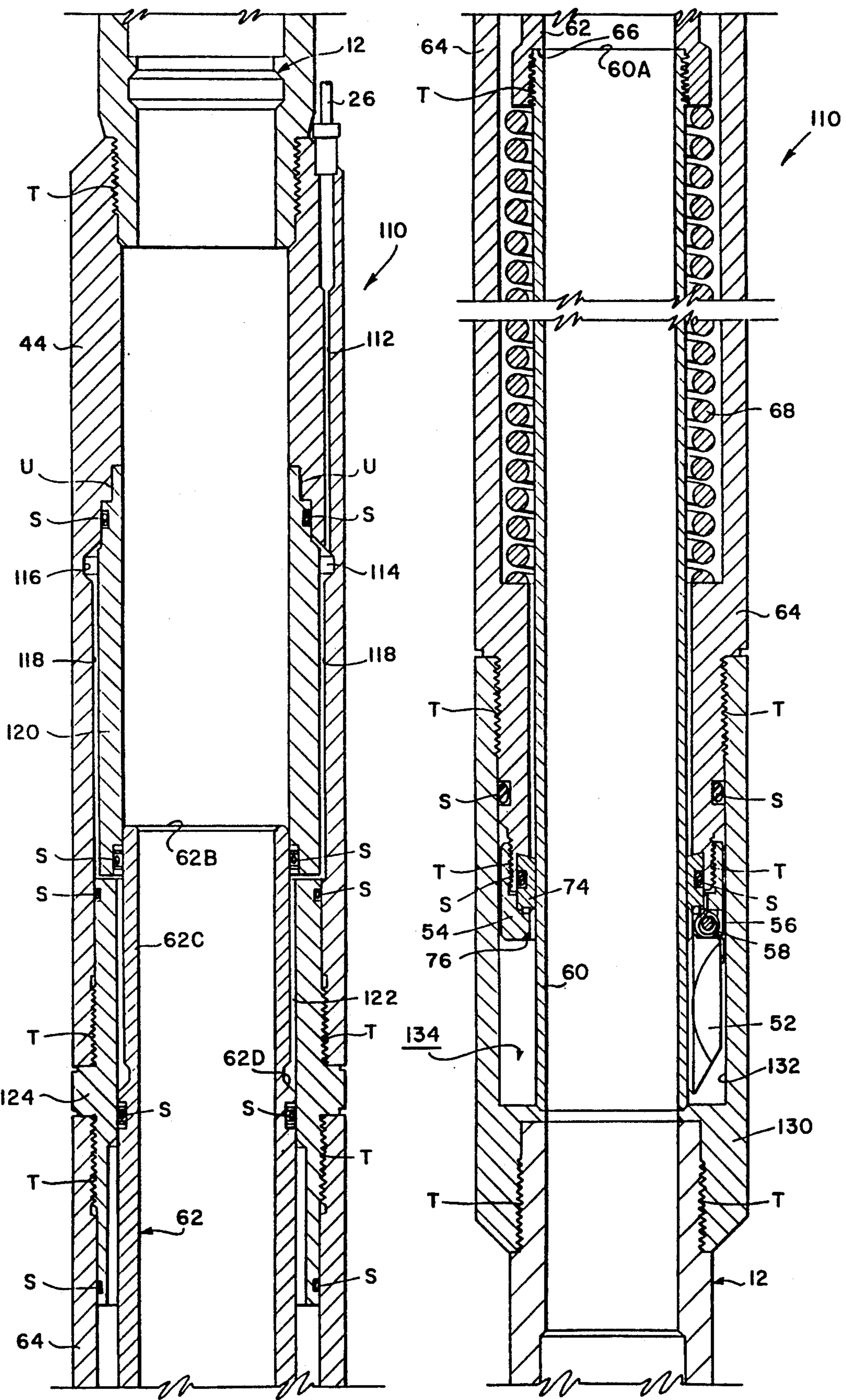
FIG. 17 VALVE OPEN
