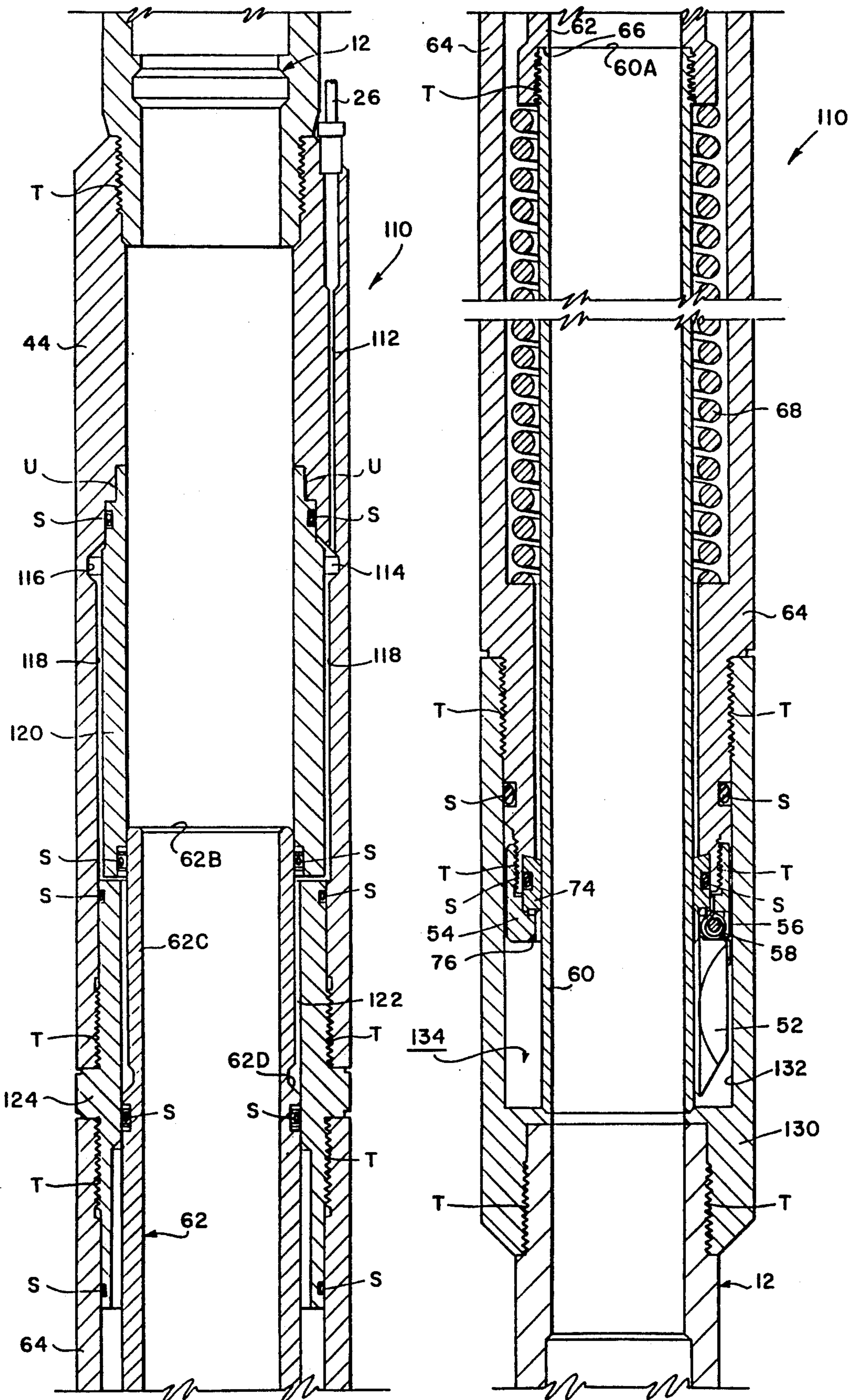
FIG. 17 VALVE OPEN
