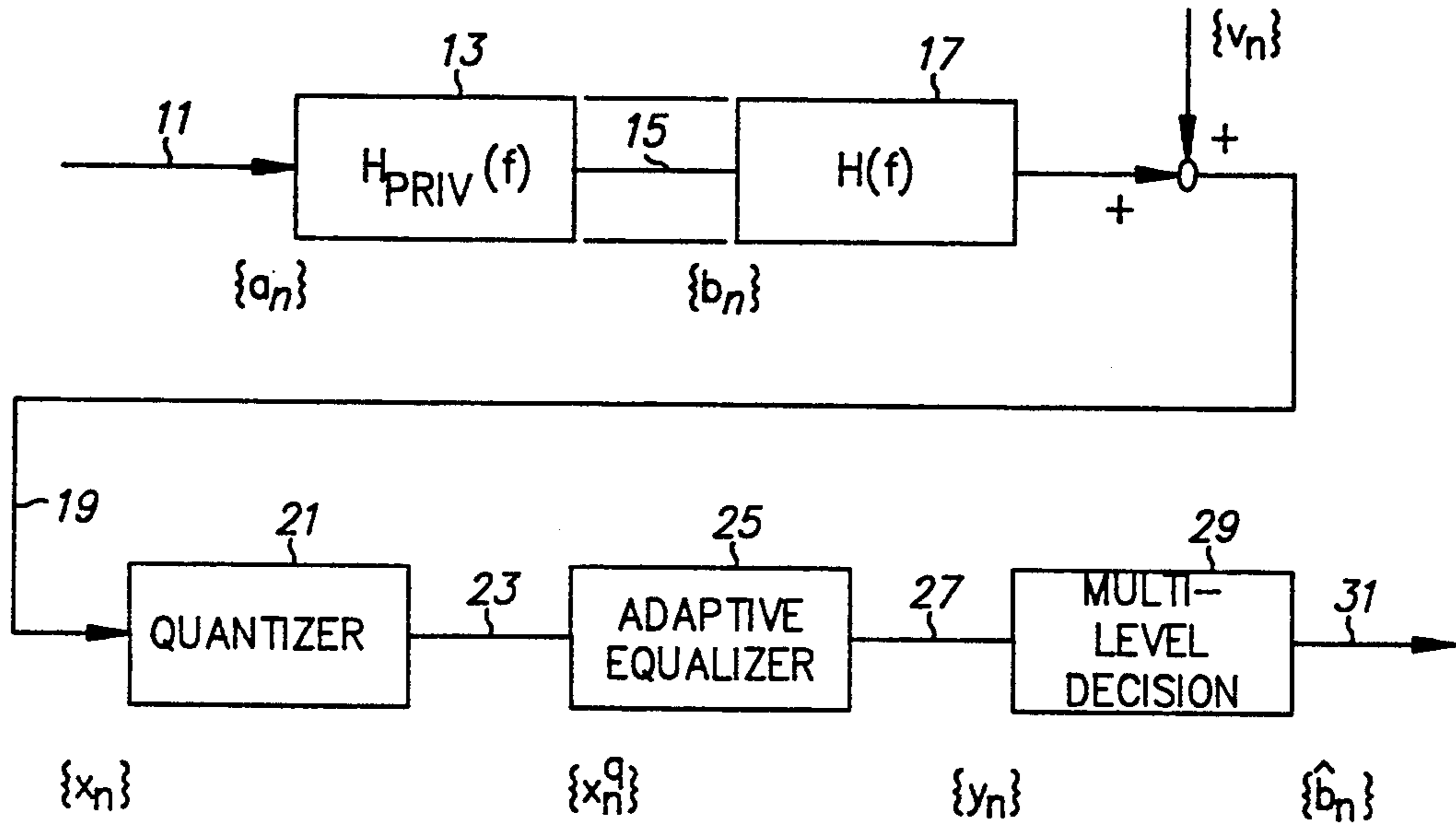
TIME-DISCRETE MODEL OF A PR IV SYSTEM
