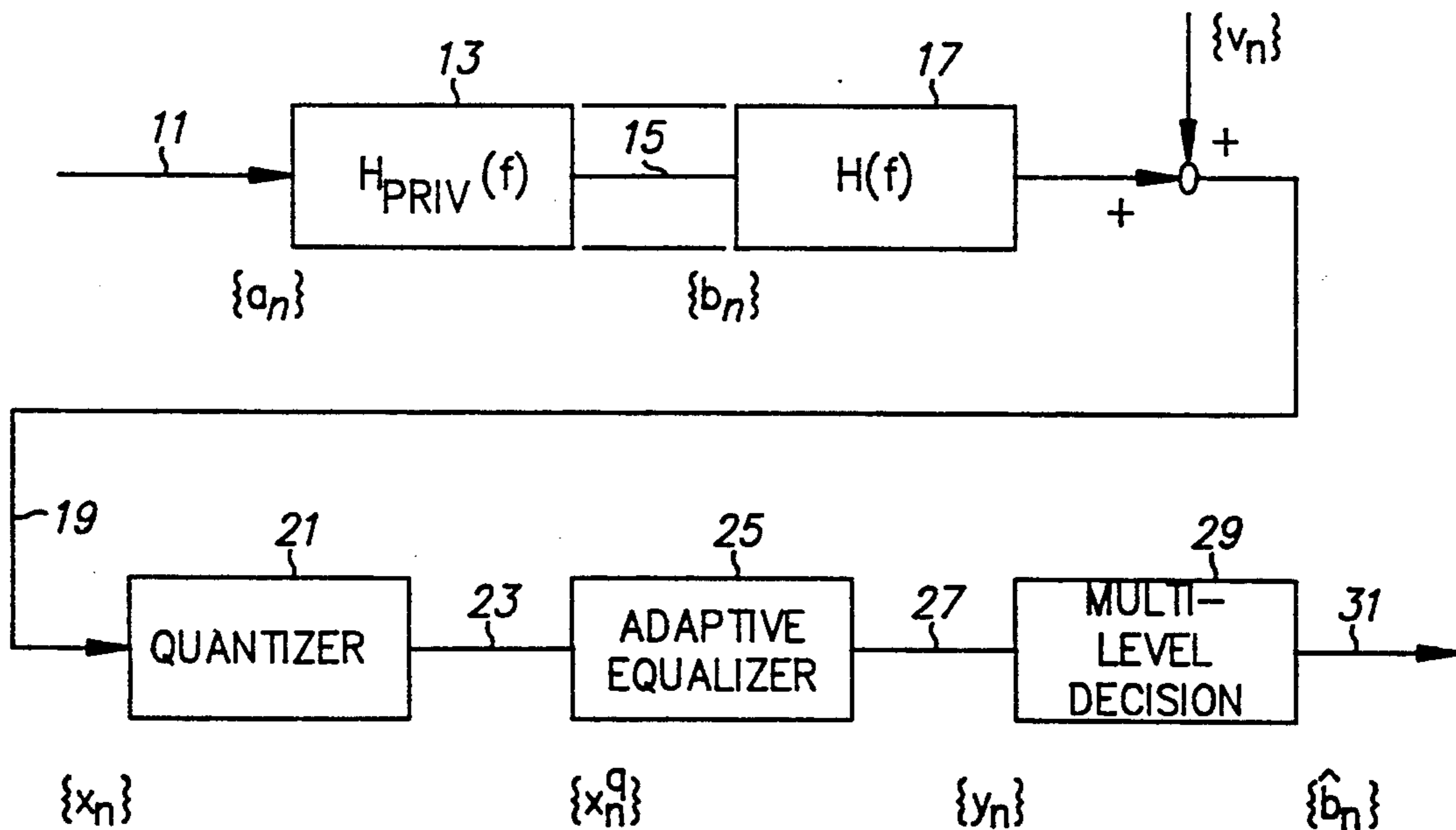
TIME-DISCRETE MODEL OF A PR IV SYSTEM
