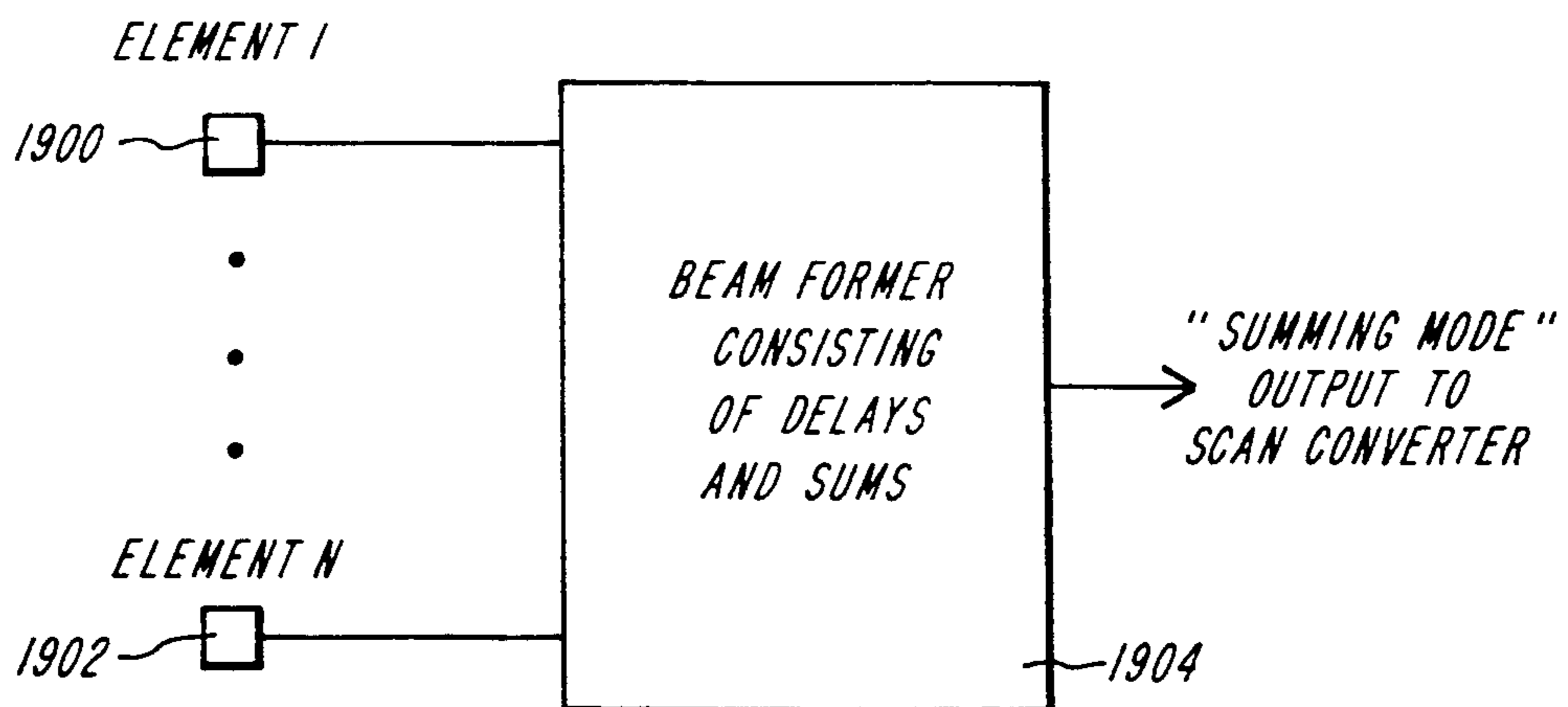
FIG. 19 (PRIOR ART)
