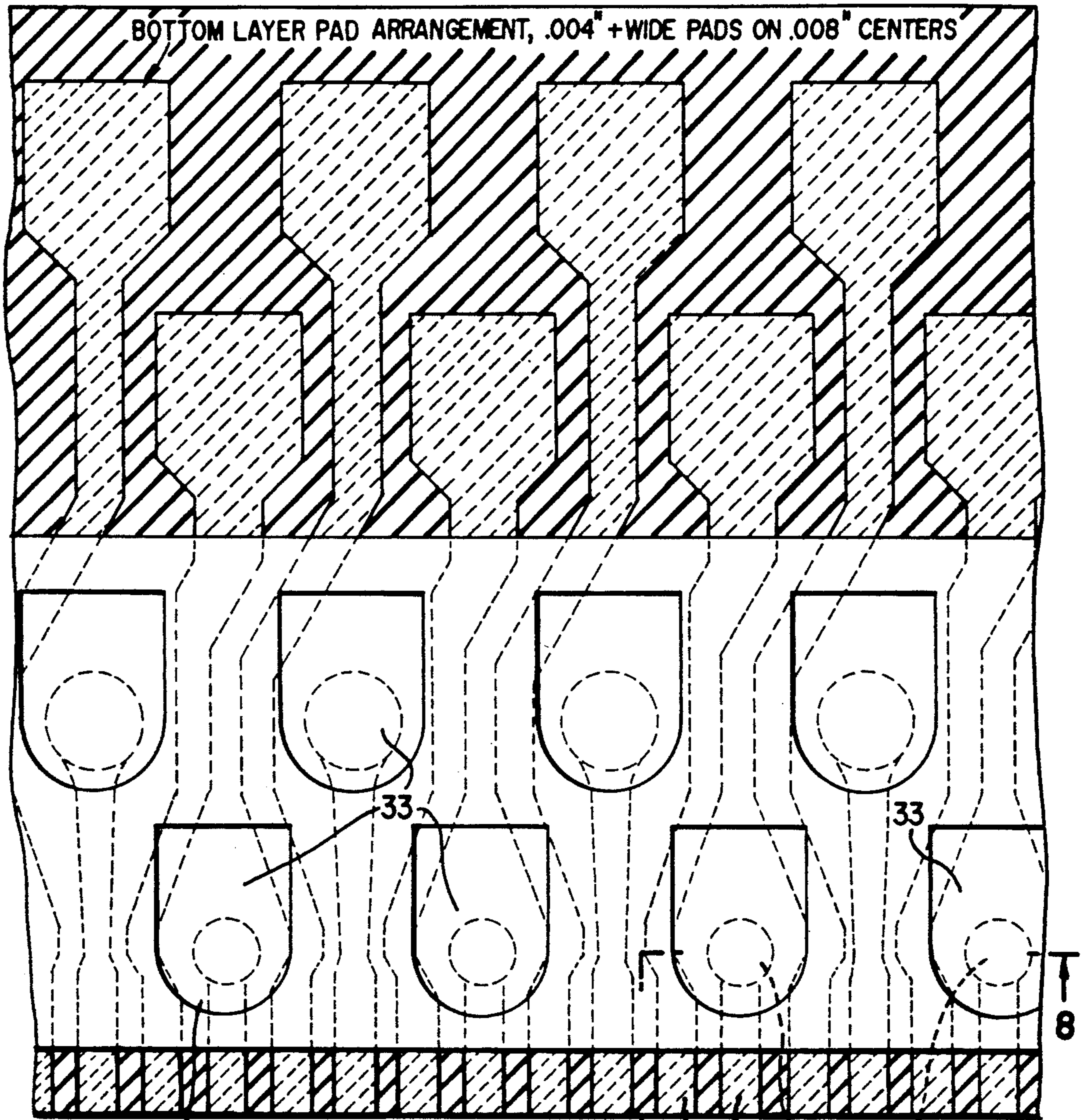
FIG. 7 .002"-.003" ETCHED THROUGH LAYER CONNECTING HOLES
