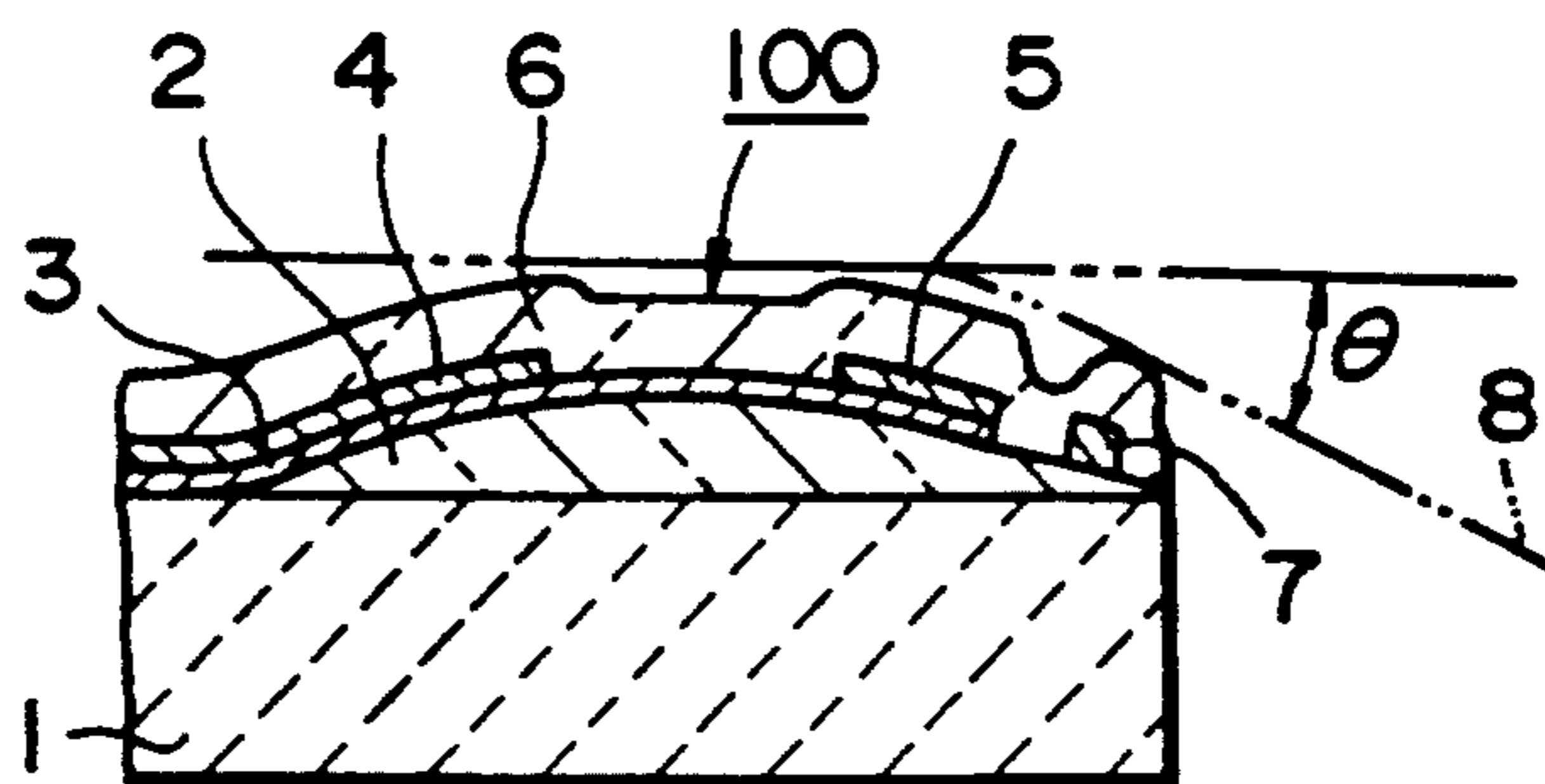
FIG. 6c PRIOR ART
