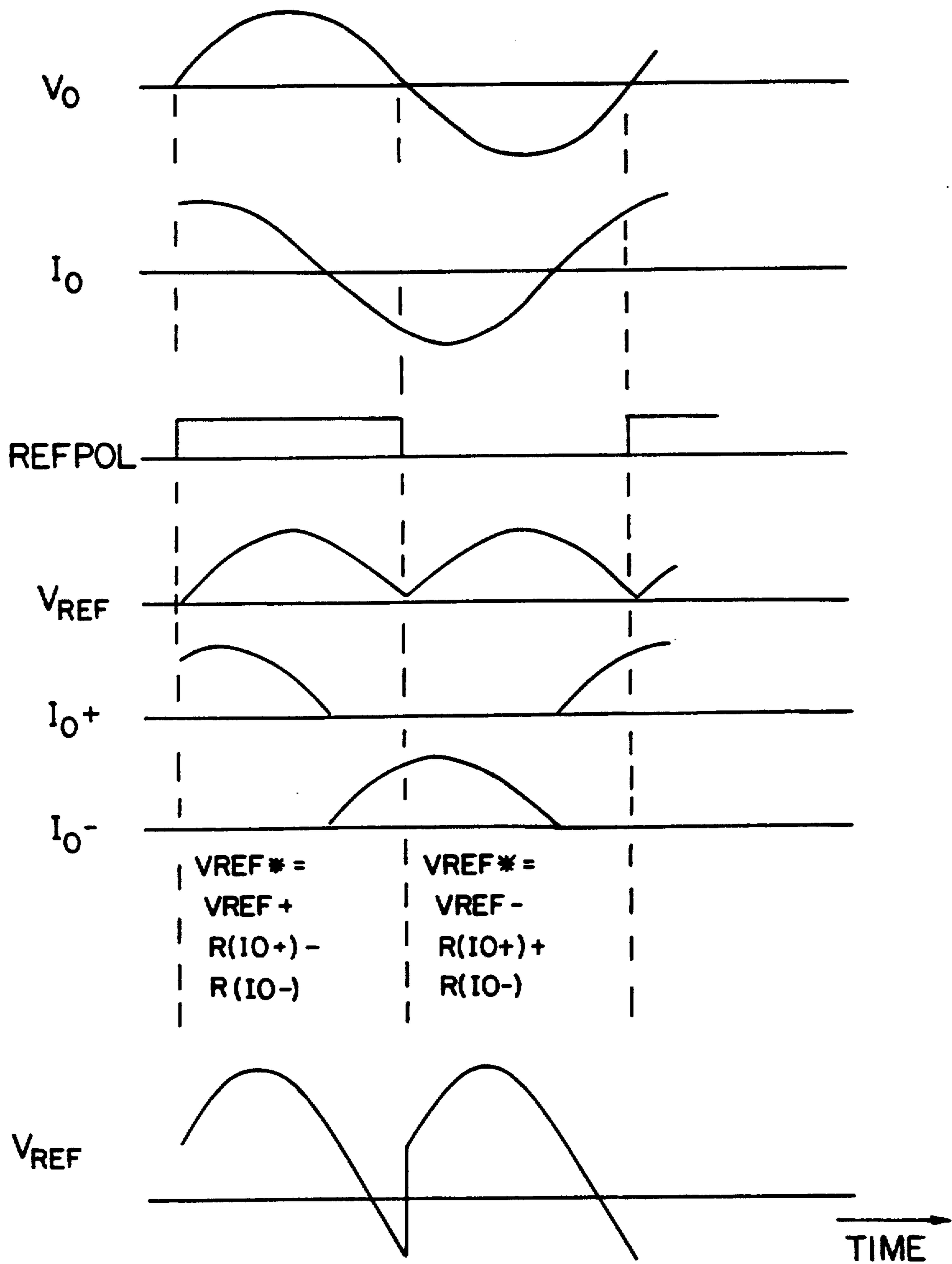
FIG. 7 REFERENCE COMPENSATION FOR LEADING POWER FACTOR LOAD
