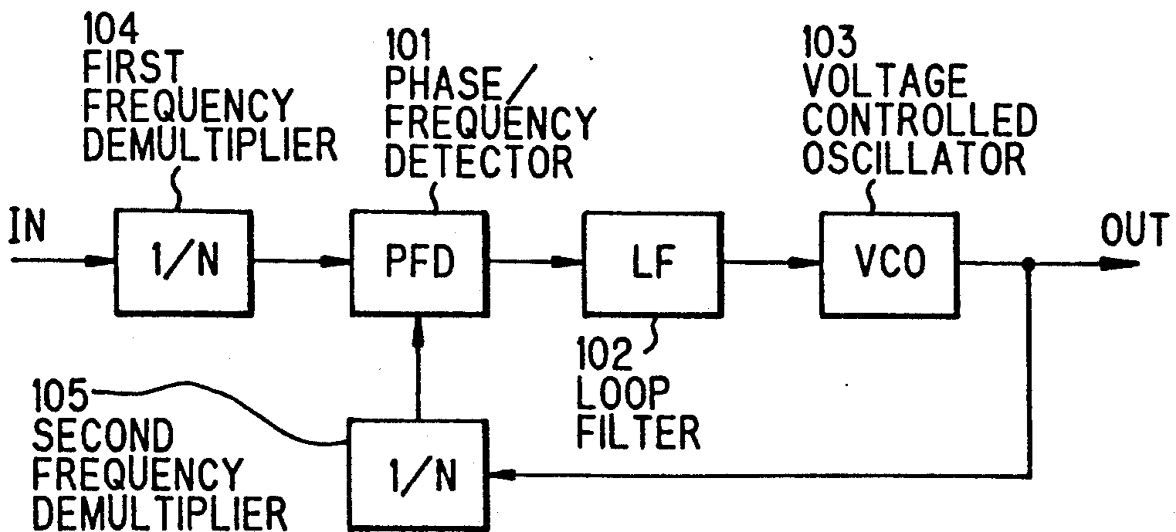
FIG.5 PRIOR ART
