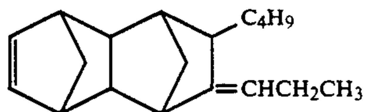
8-n-Propylidene-9-butyltetracyclo[4,4,0,1 2.5 ,1 7.10 ]-3-dodecene
