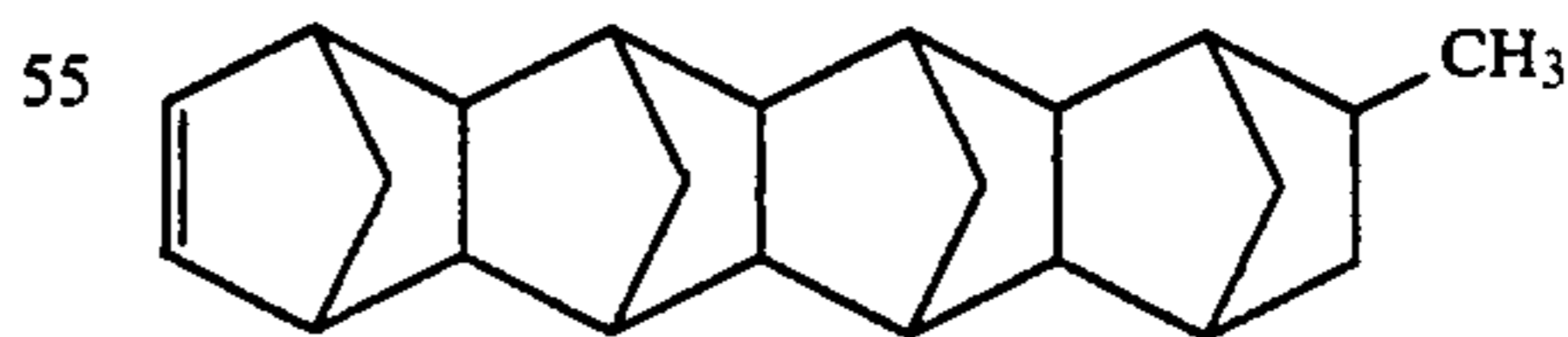
15-Methyloctacyclo[8,8,0,1 2.9 ,1 4.7 ,1 11.18 ,1 13.16 ,0 3.8 ,0 12.17 ]-5-docosene
