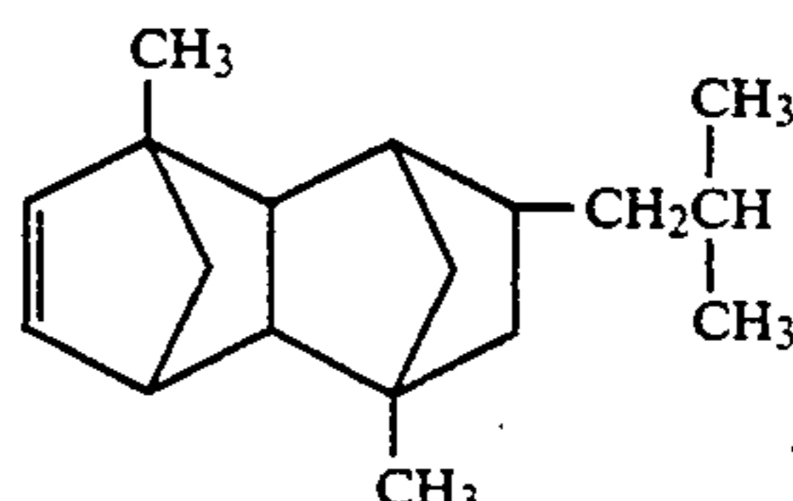
9-Isobutyl-2,7-dimethyltetracyclo[4,4,0,1 2.5 ,1 7.10 ]-3-dodecene
