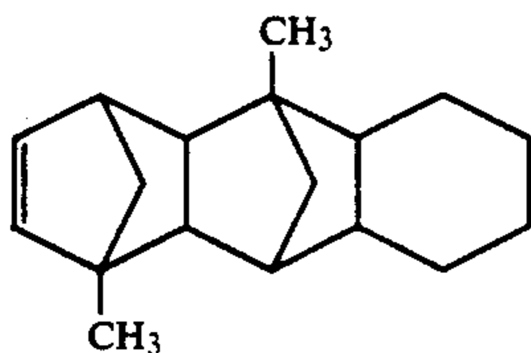
1,6-Dimethylpentacyclo[6,6,1,1,3,6,0,2,7,0,9,14]-4-hexadecene
