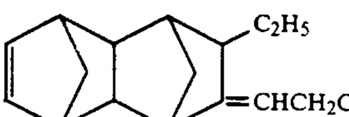
8-n-Propylidene-9-ethyltetracyclo[4,4,0,1 2.5 ,1 7.10 ]-3-dodecene
