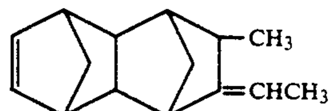
8-Ethylidene-9-methyltetracyclo[4,4,0,1 2.5 ,1 7.10 ]-3-dodecene
