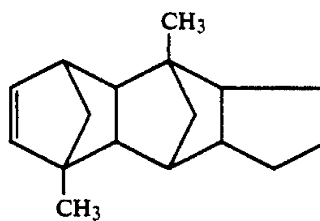
1,6-Dimethylpentacyclo[6,5,1,1,3,6,0,2,7,0,9,13]-4-pentadecene
