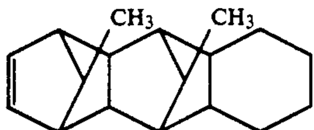
15,16-Dimethylpentacyclo[6,6,1,1,3,6,0,2,7,0,9,14]-4-hexadecene
