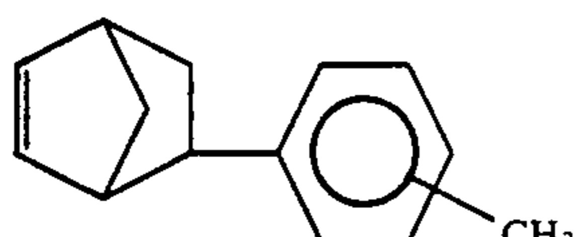
5-Tolylbicyclo[2,2,1]hept-2-ene
