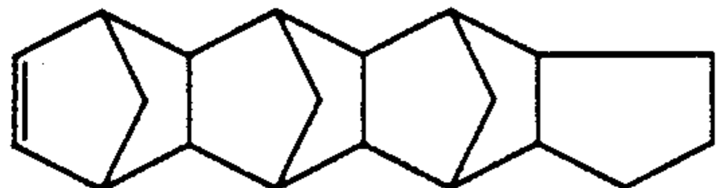
Heptacyclo[8,7,0,1,2,9,14,7,11,17,0,3,8,0,12,16]-5-icosene
