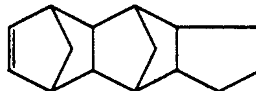
Pentacyclo[6,5,1,1,3,6,0,2,7,0,9,13]-4-pentadecene
