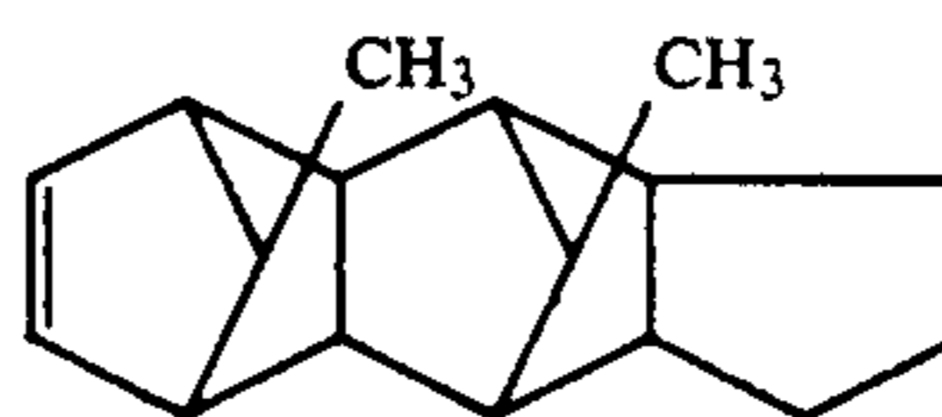
14,15-Dimethylpentacyclo[6,5,1,1,3,6,0,2,7,0,9,13]-4-pentadecene
