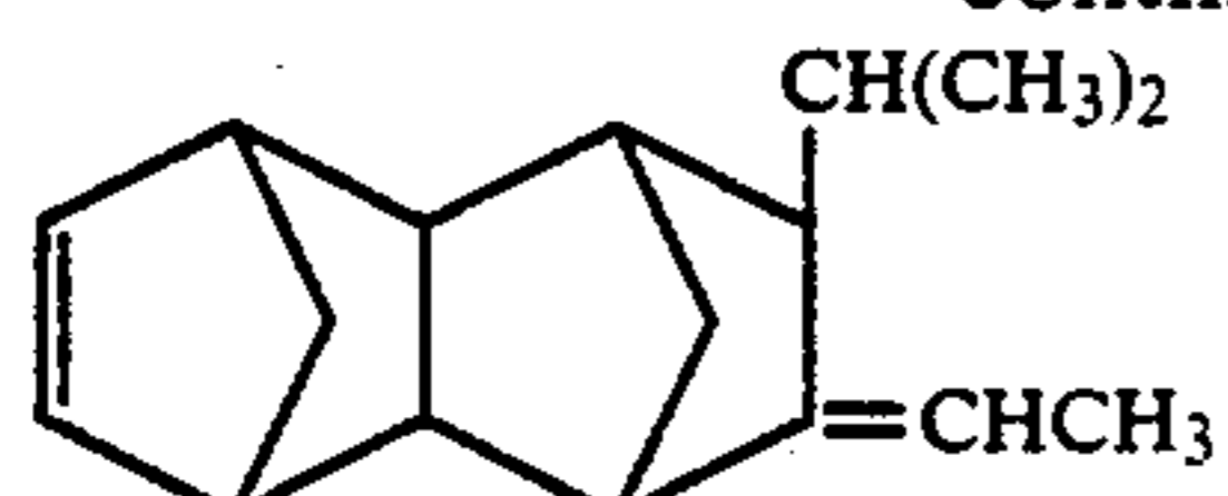
8-Ethylidene-9-isopropyltetracyclo[4,4,0,1 2.5 ,1 7.10 ]-3-dodecene
