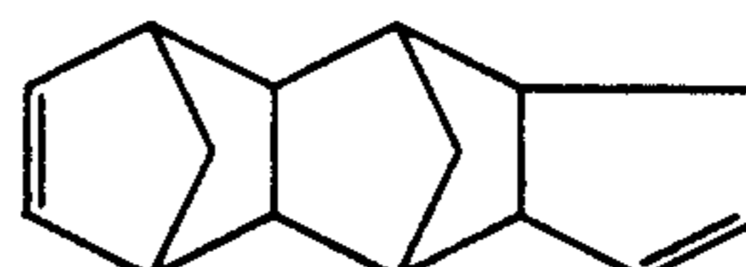
Pentacyclo[6,5,1,1,3,6,0,2,7,0,9,13]-4,10-pentadecadiene:
