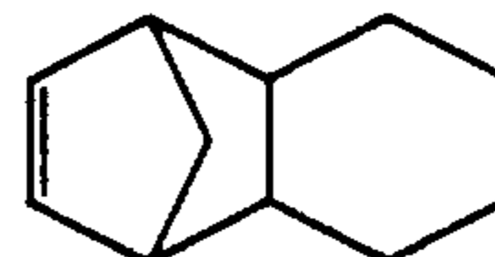
Tricyclo[4,4,0,1,2,5]-3-undecene
