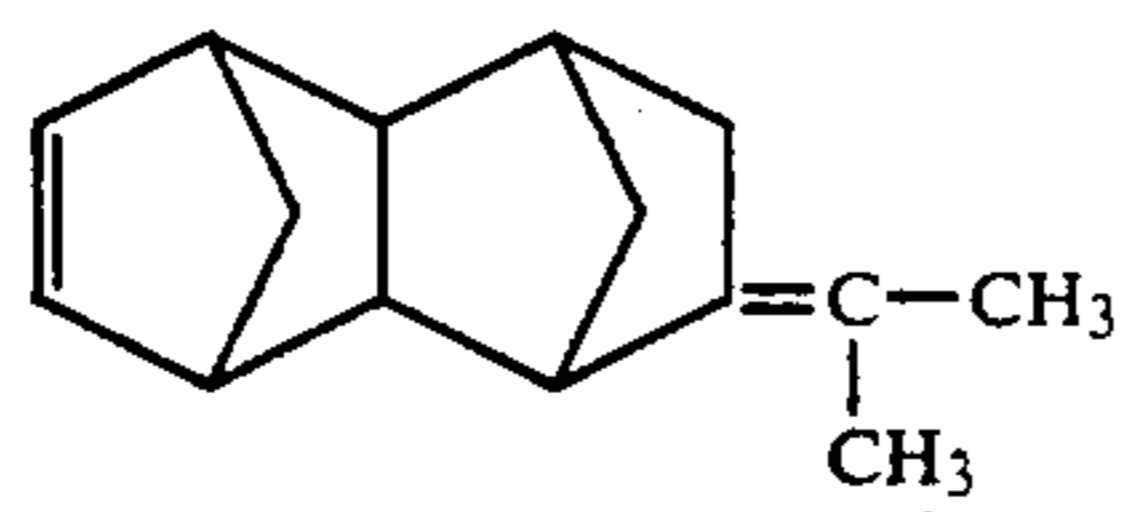
8-Isopropylidene-9-methyltetracyclo[4,4,0,1 2.5 ,1 7.10 ]-3-dodecene
