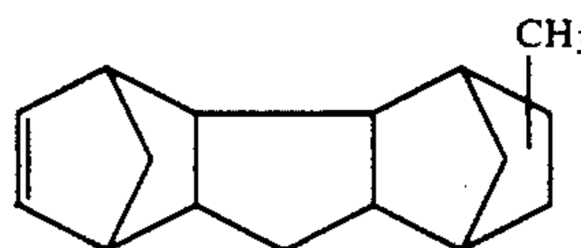
Methyl-substituted pentacyclo[7,4,0,1,2,5,0,8,13,19,12]-3-pentadecene
