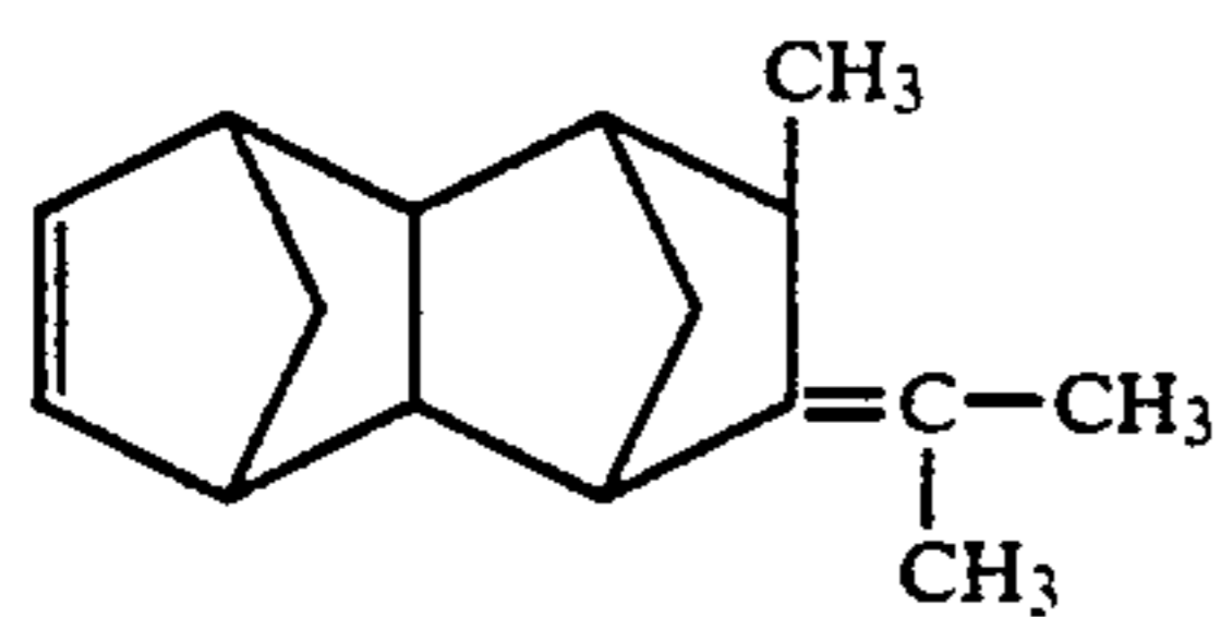
8-Isopropylidene-9-methyltetracyclo[4,4,0,1 2.5 ,1 7.10 ]-3-dodecene
