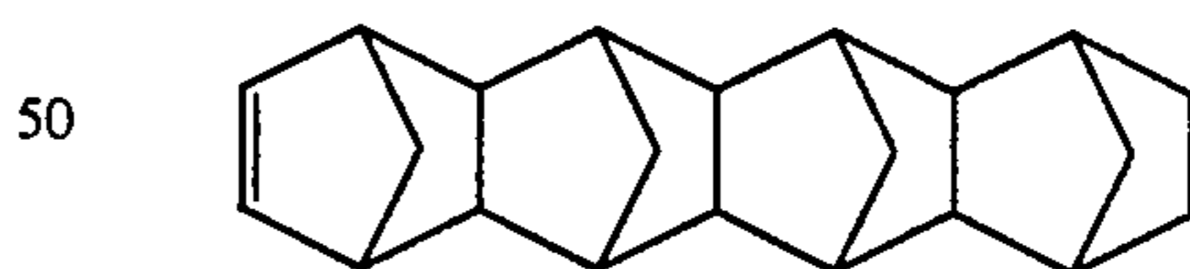
Octacyclo[8,8,0,1 2.9 ,1 4.7 ,1 11.18 ,1 13.16 ,0 3.8 ,0 12.17 ]-5-docosene
