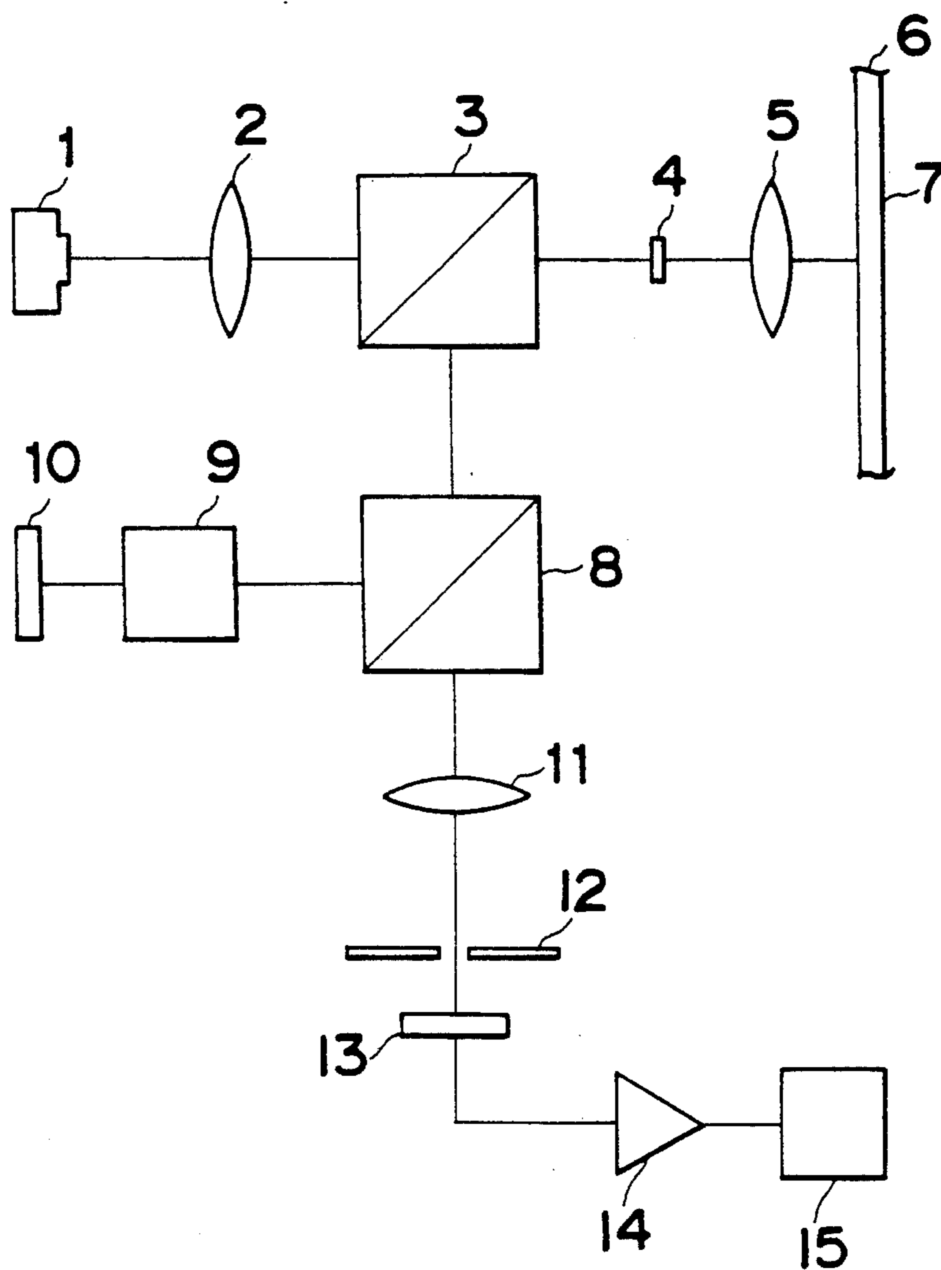
Fig. 1 PRIOR ART
