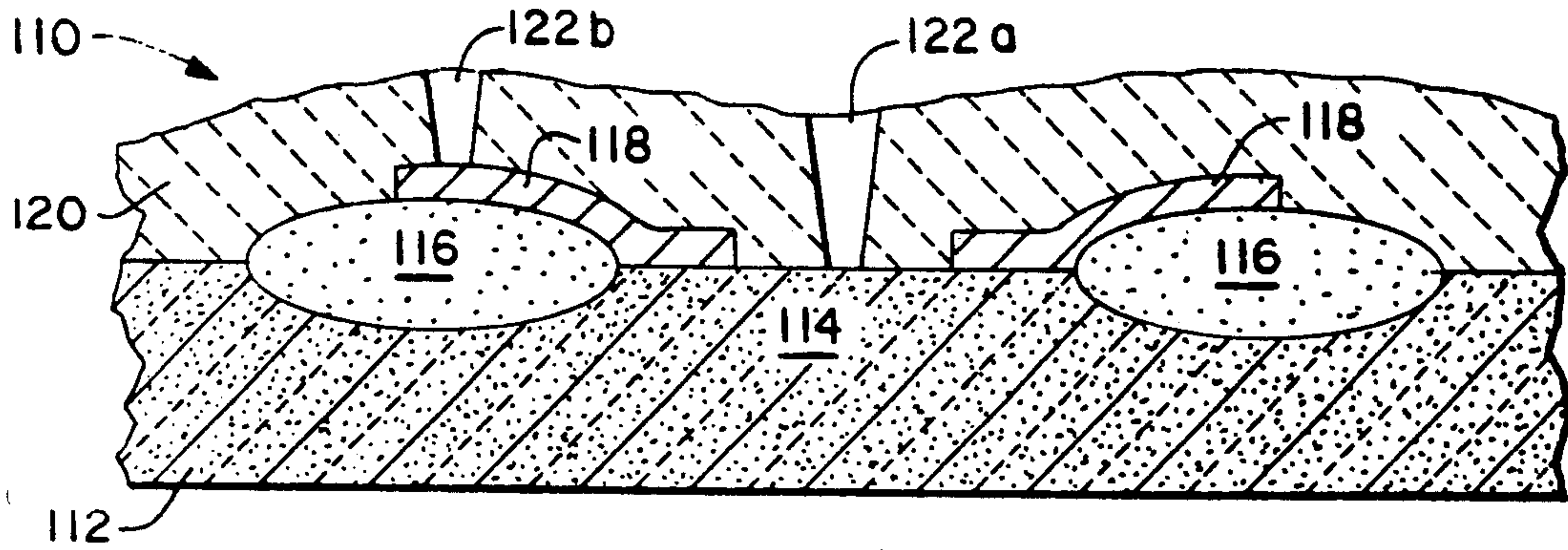
FIG. 1 PRIOR ART
