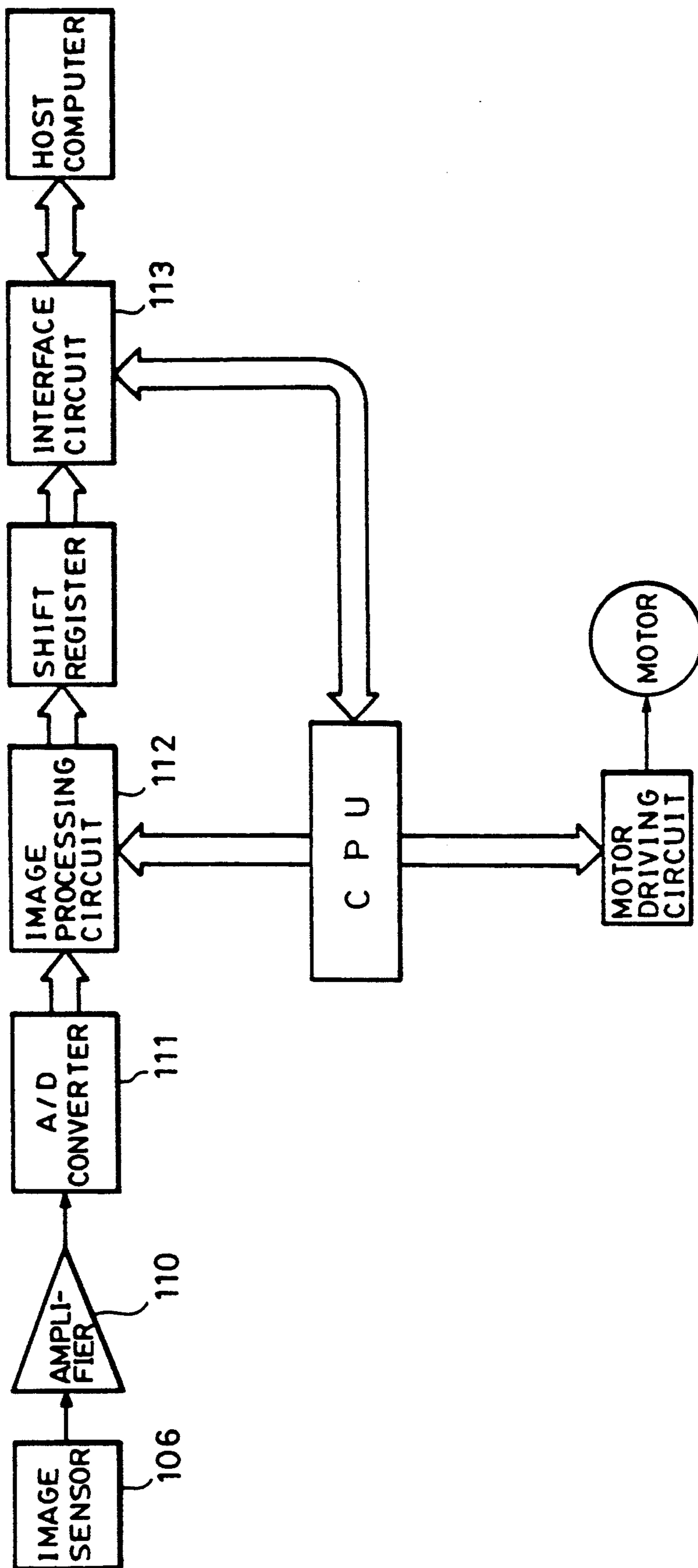
FIG. 6 (PRIOR ART)
