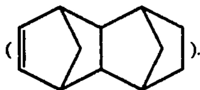
tetracyclo[4,4,0,1 2,5 ,17,10]-3-dodecene
