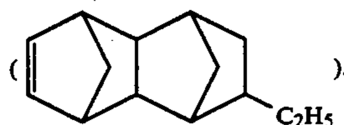
8-ethyl-tetracyclo[4,4,0,1 2,5 ,17,10]-3-dodecene
