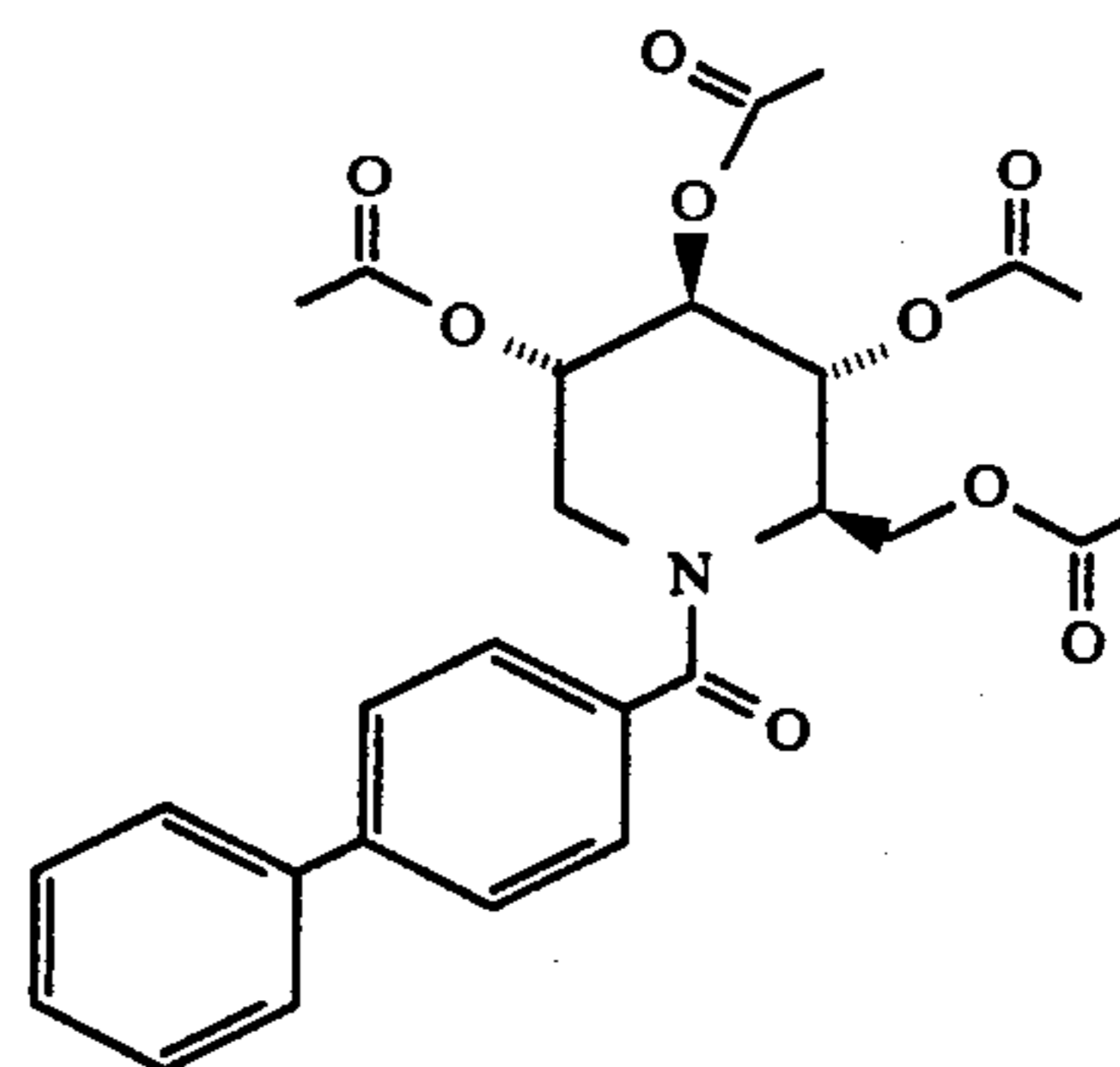
1,5-[[[1,1'-biphenyl]-4-ylcarbonyl]imino]-1,5-dideoxy-D-glucitol, tetraacetate
