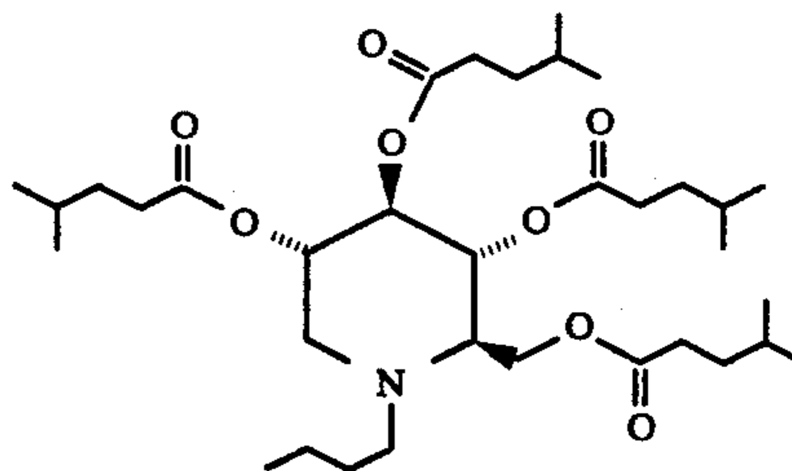
1,5-(Butylimino)-1,5-dideoxy-D-glucitol, tetra(4-methylpentanoate)
