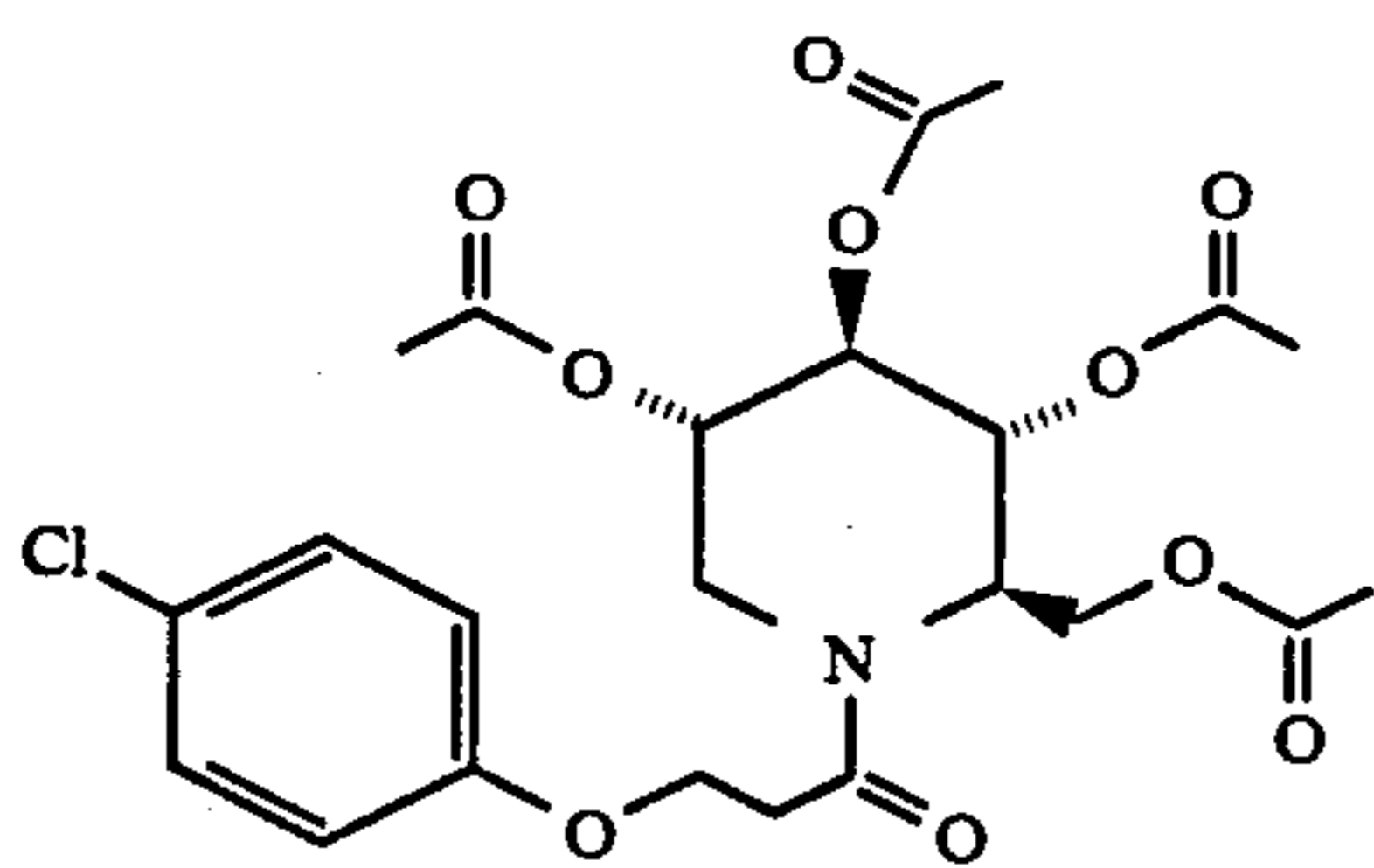
1,5-Dideoxy-1,5-[[3-(4-chlorophenoxy)-1-oxopropyl]imino]-D-glucitol, tetraacetate
