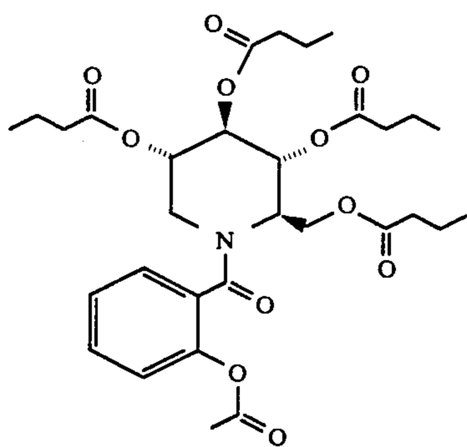
1,5-[[2-(Acetyloxy)benzoyl]imino]-1,5-dideoxy-D-glucitol, tetrabutanoate
