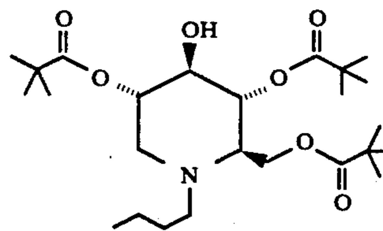
1,5-(Butylimino)-1,5-dideoxy-D-glucitol, (2,4,6-tri(2,2-dimethylpropanoate))
