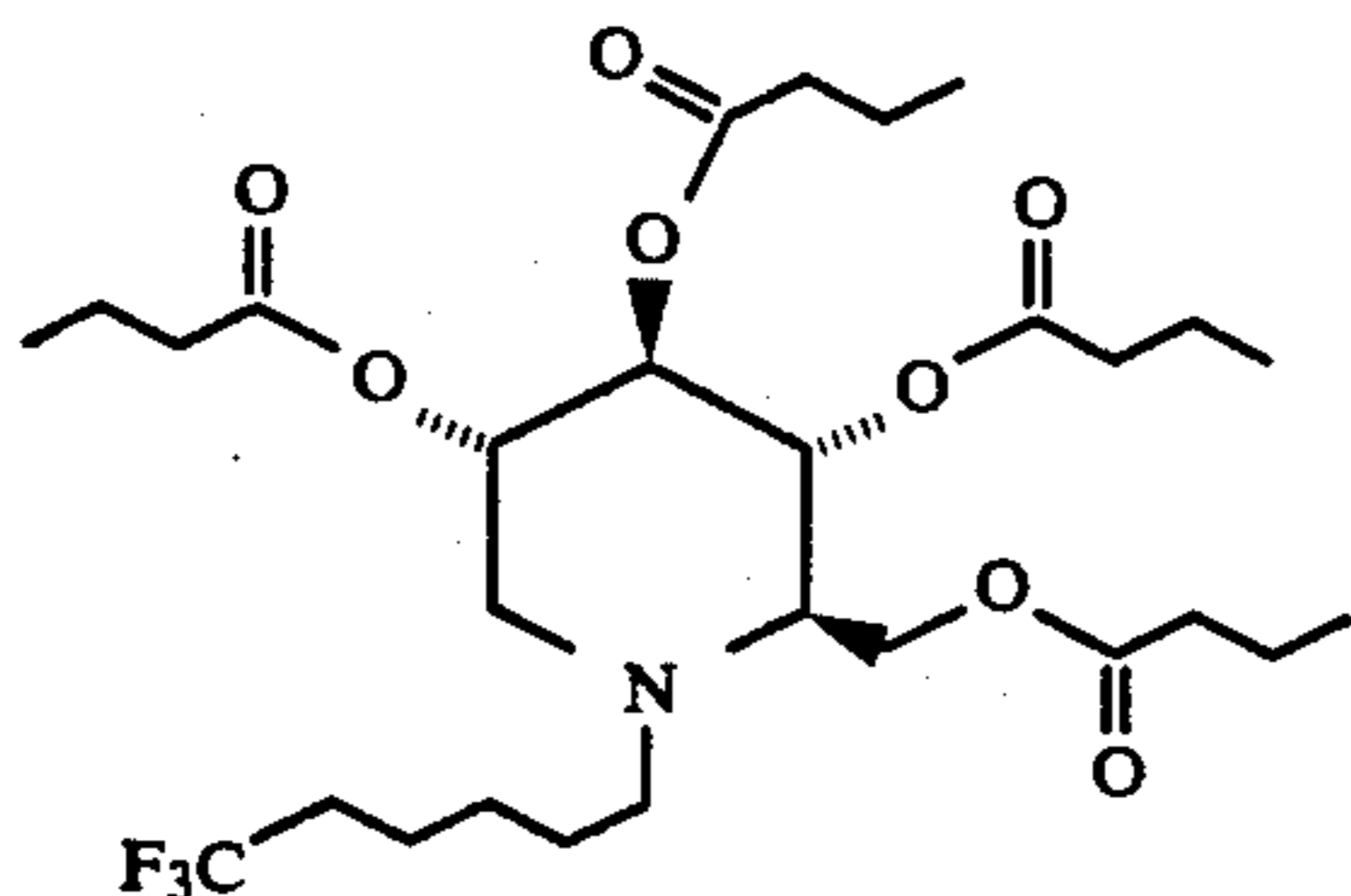
1,5-(6,6,6-Trifluorohexylimino)-1,5-dideoxy-D-glucitol, tetrabutyrates
