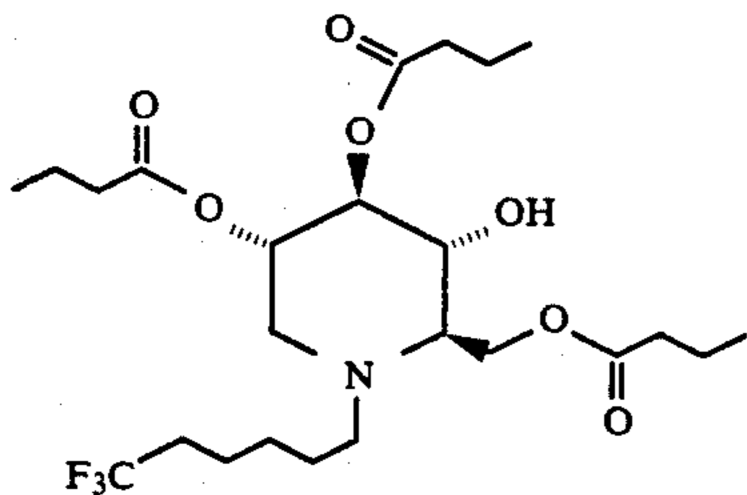
1,5-(6,6,6-Trifluorohexylimino)-1,5-dideoxy-D-glucitol, 2,3,6-tributyrates
