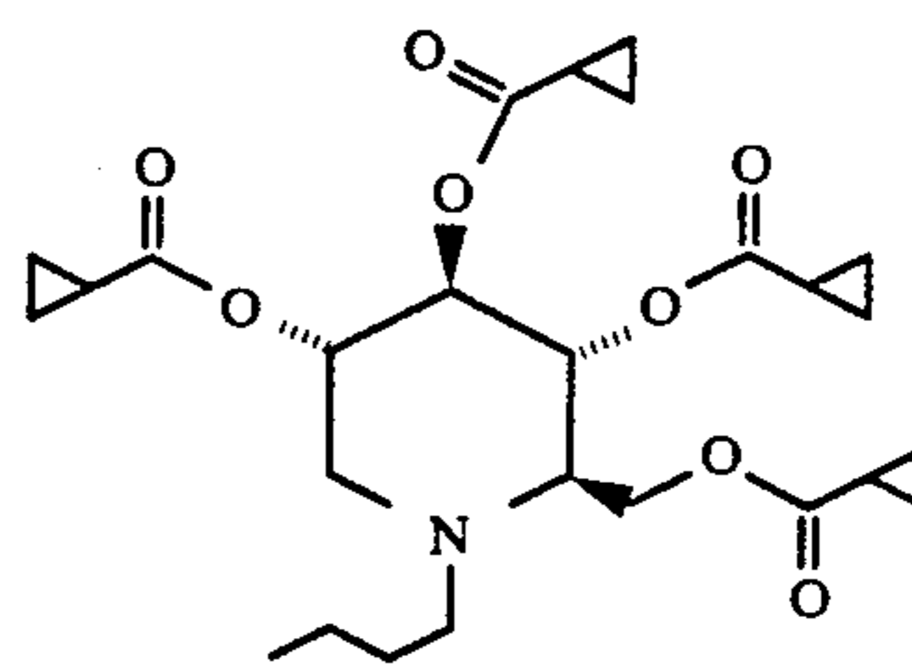
1,5-(Butylimino)-1,5-dideoxy-D-glucitol, tetra(cyclopropylcarboxylate)
