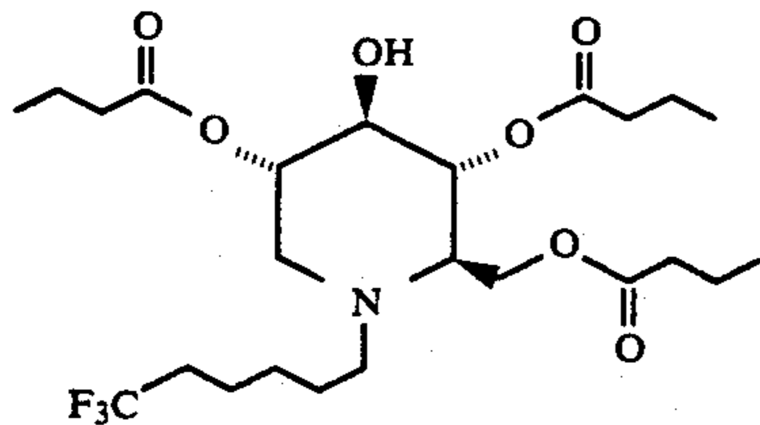
1,5-(6,6,6-Trifluorohexylimino)-1,5-dideoxy-D-glucitol, 2,4,6-tributyrates
