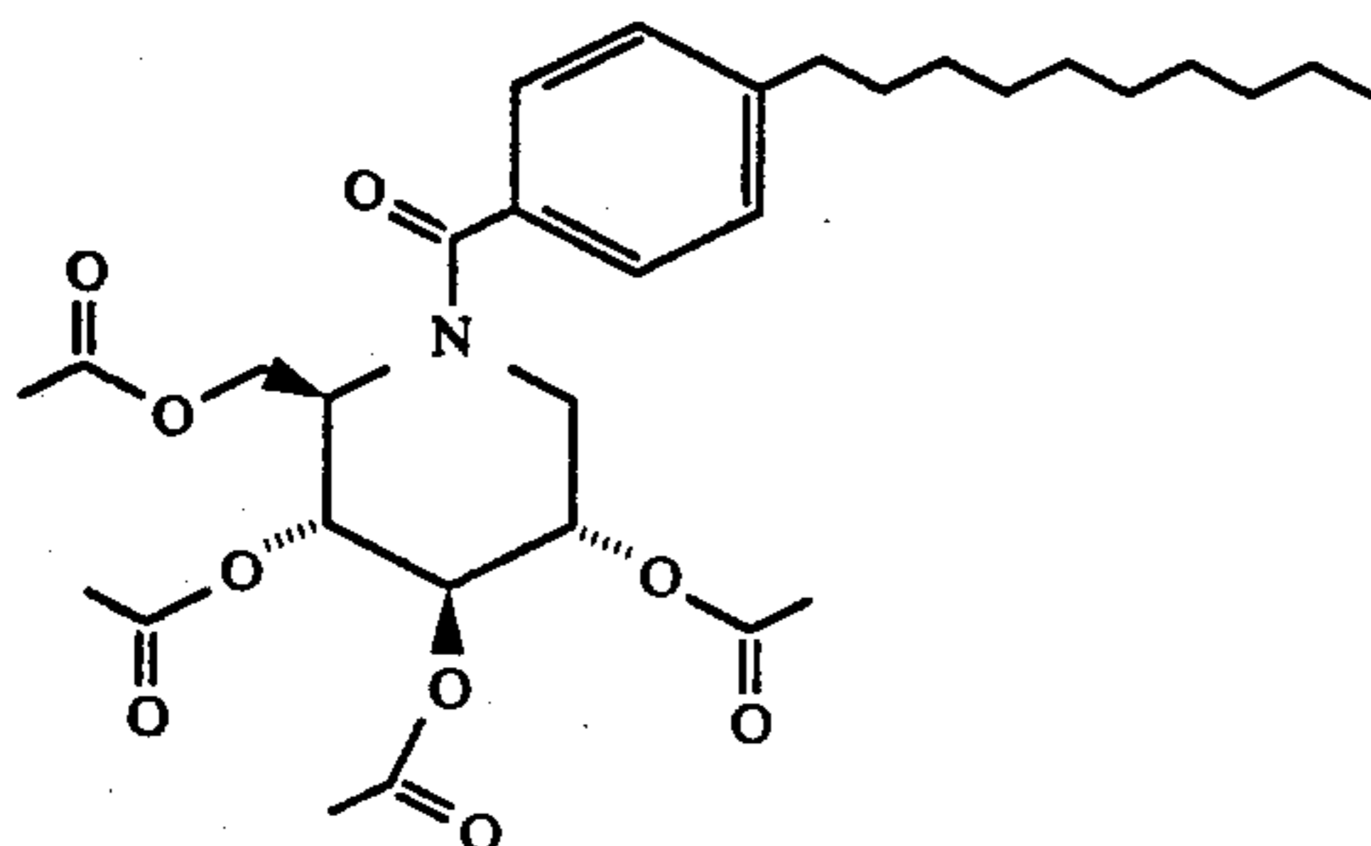
1,5-[(4-Decylbenzoyl)imino]-1,5-dideoxy-D-glucitol, tetraacetate
