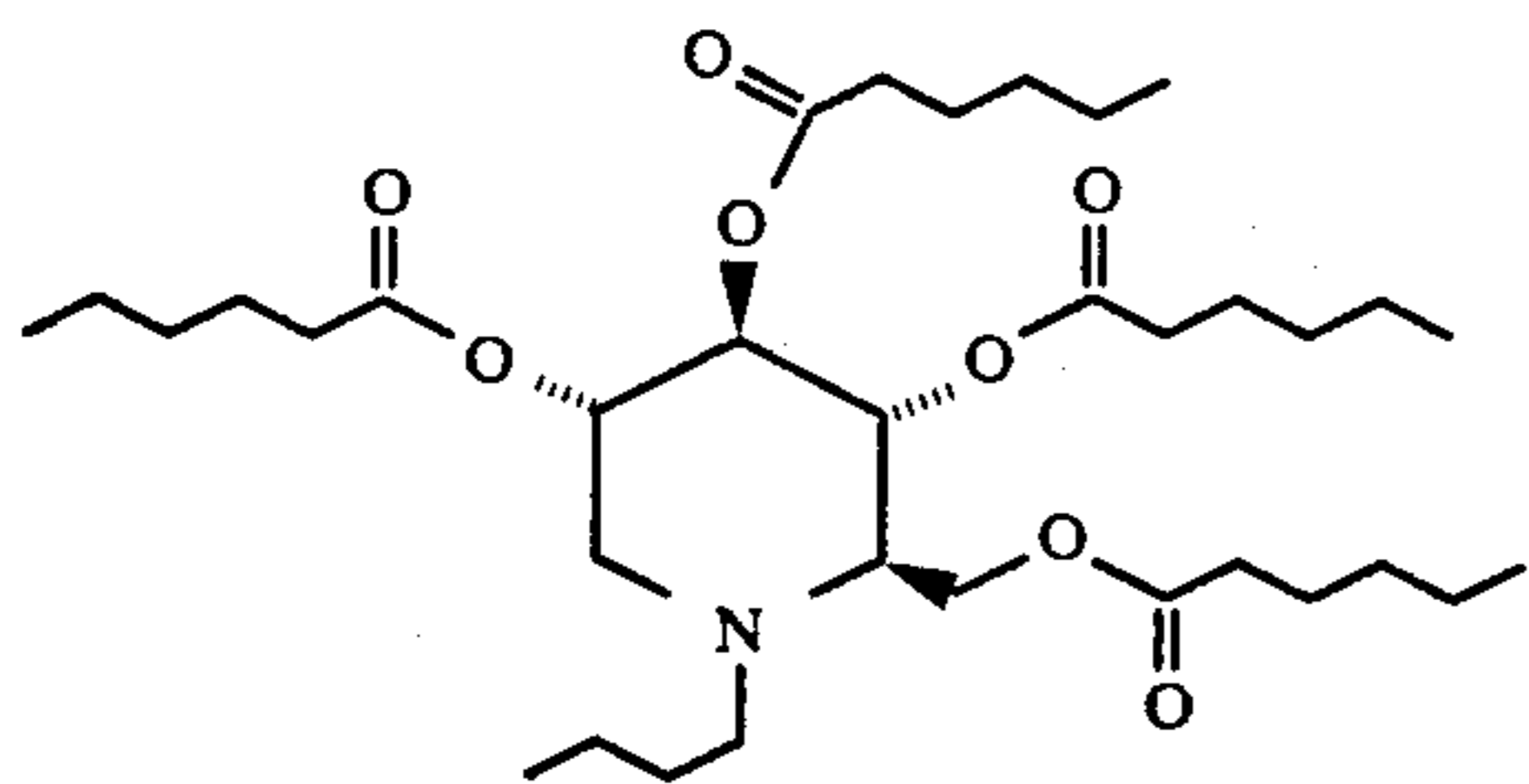
1,5-(Butylimino)-1,5-dideoxy-D-glucitol, tetrahexanoate
