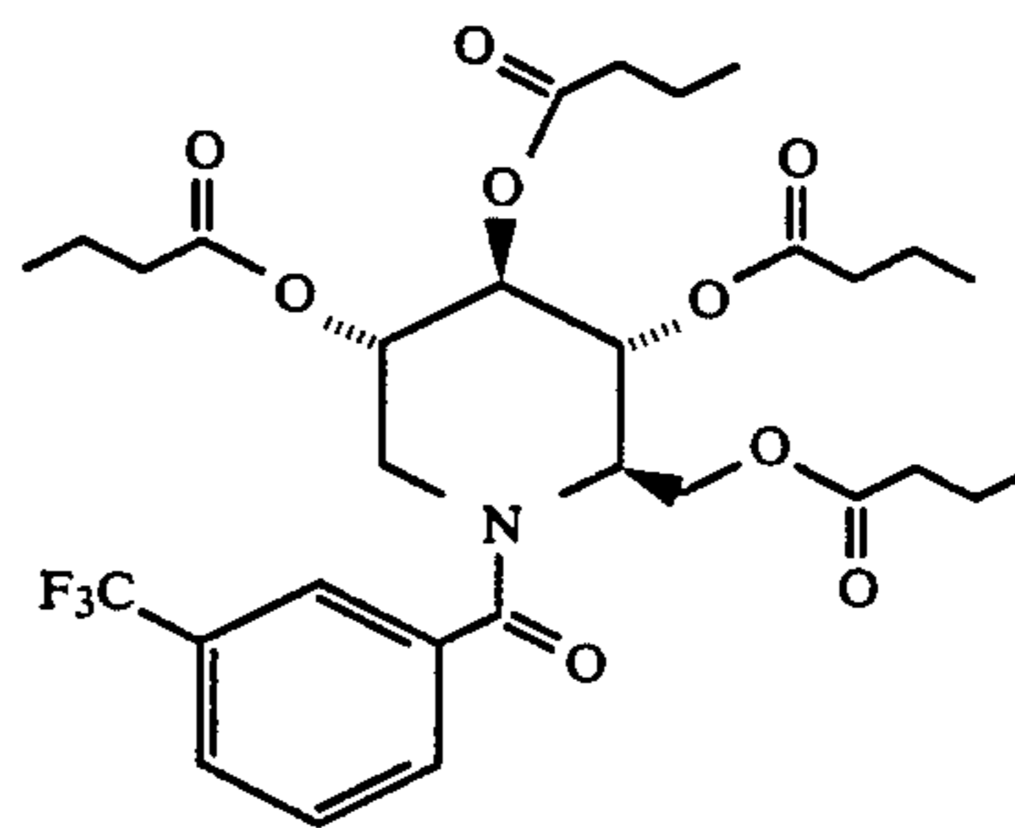
1,5-Dideoxy-1,5-[[3-(trifluoromethyl)benzoyl]imino]-D-glucitol, tetrabutanoate
