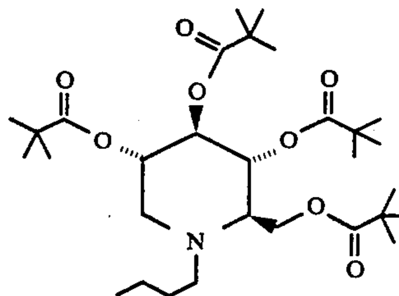
1,5-(Butylimino)-1,5-dideoxy-D-glucitol, tetra(2,2-dimethylpropanoate)
