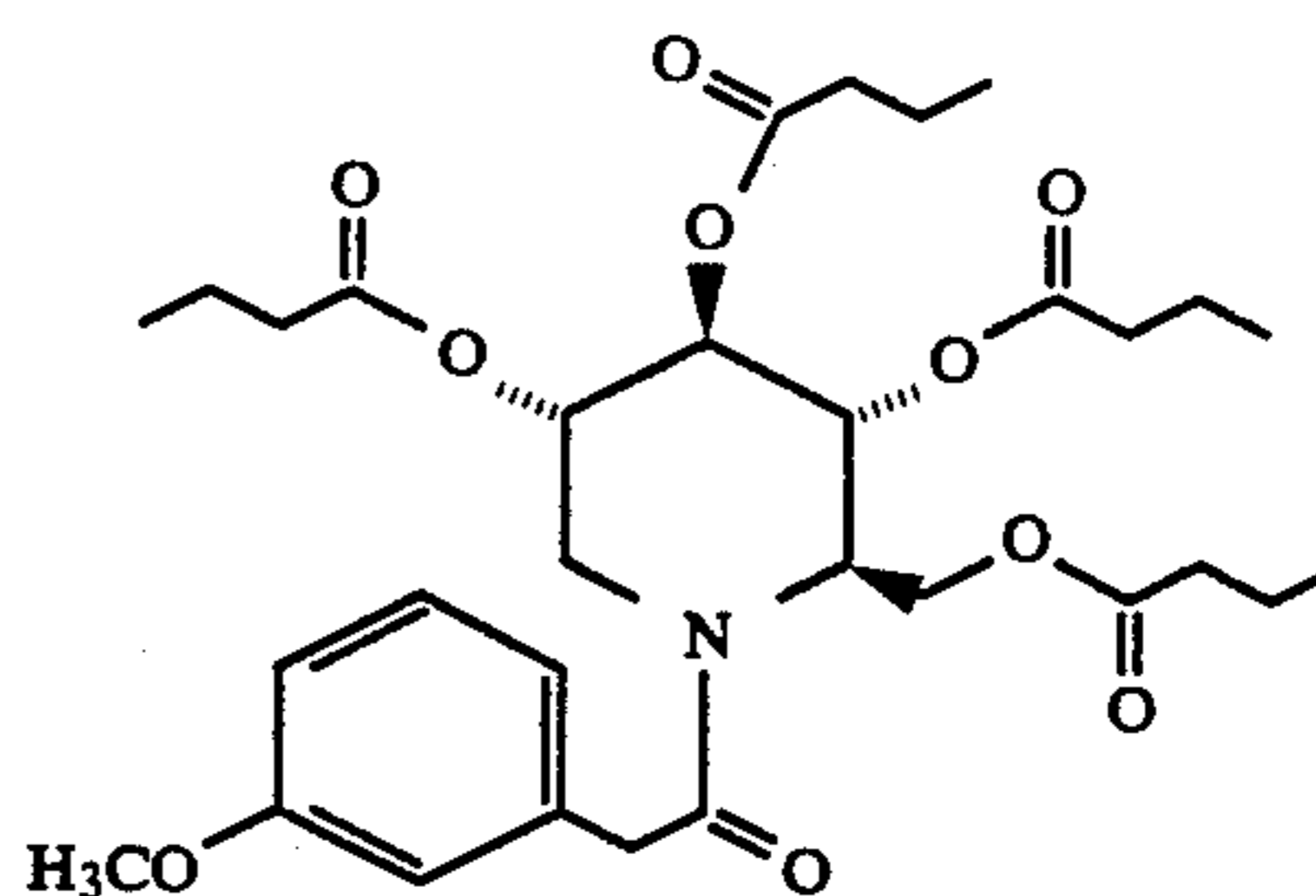
1,5-Dideoxy-1,5-[[2-(3-methoxyphenyl)-1-oxoethyl]imino]-D-glucitol, tetrabutanoate
