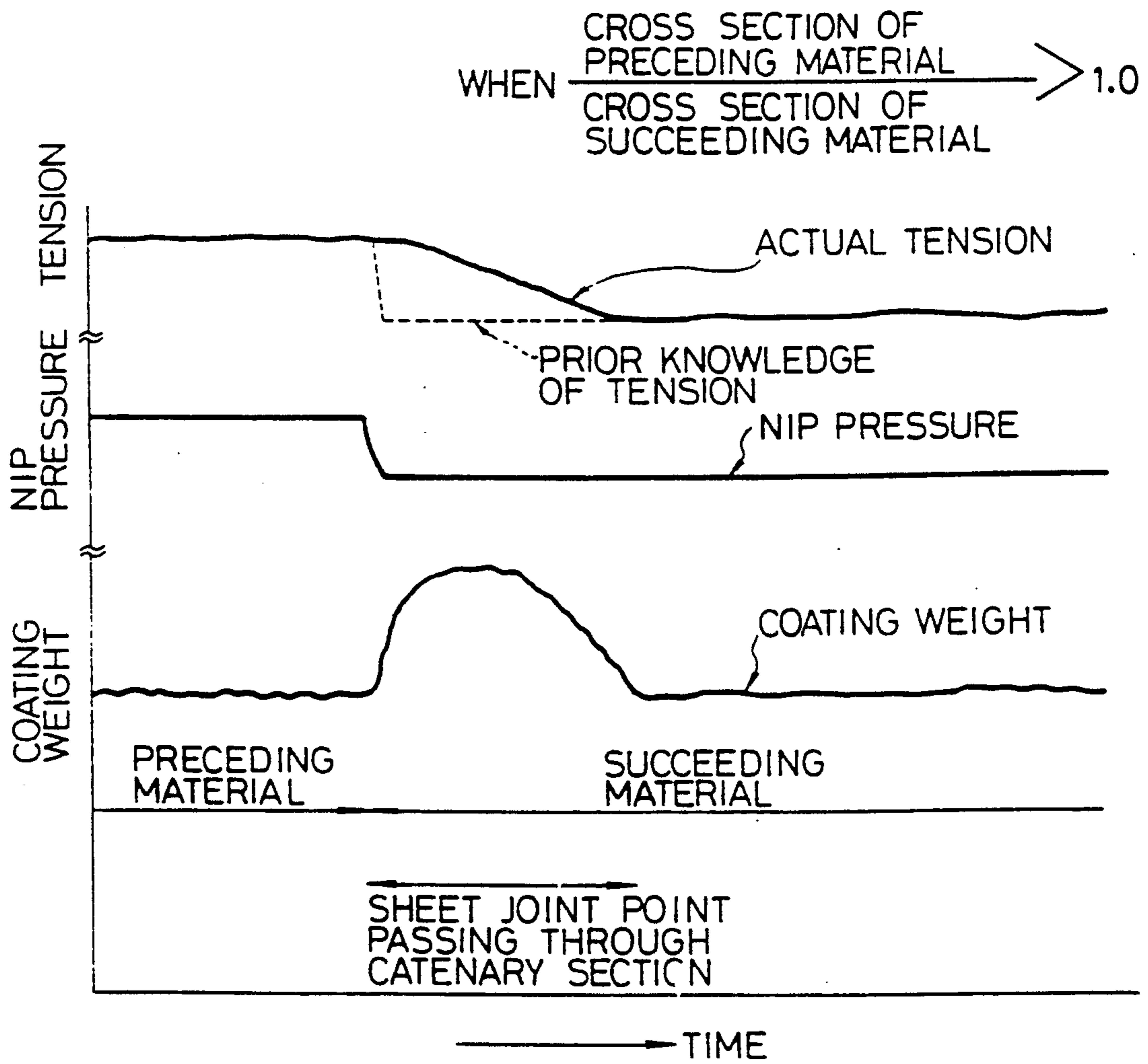
FIG. 45 PRIOR ART
