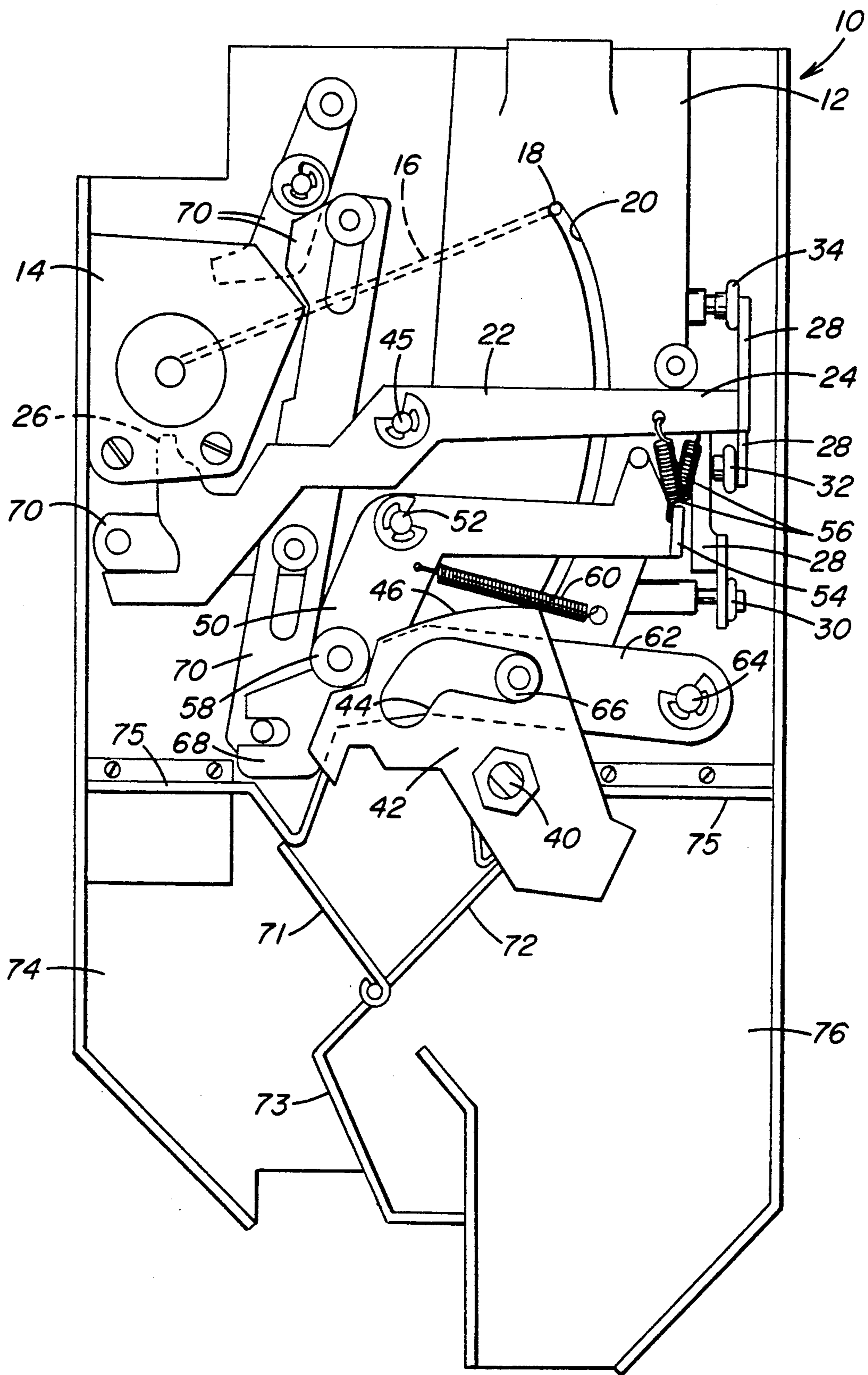
FIG. 4 PRIOR ART
