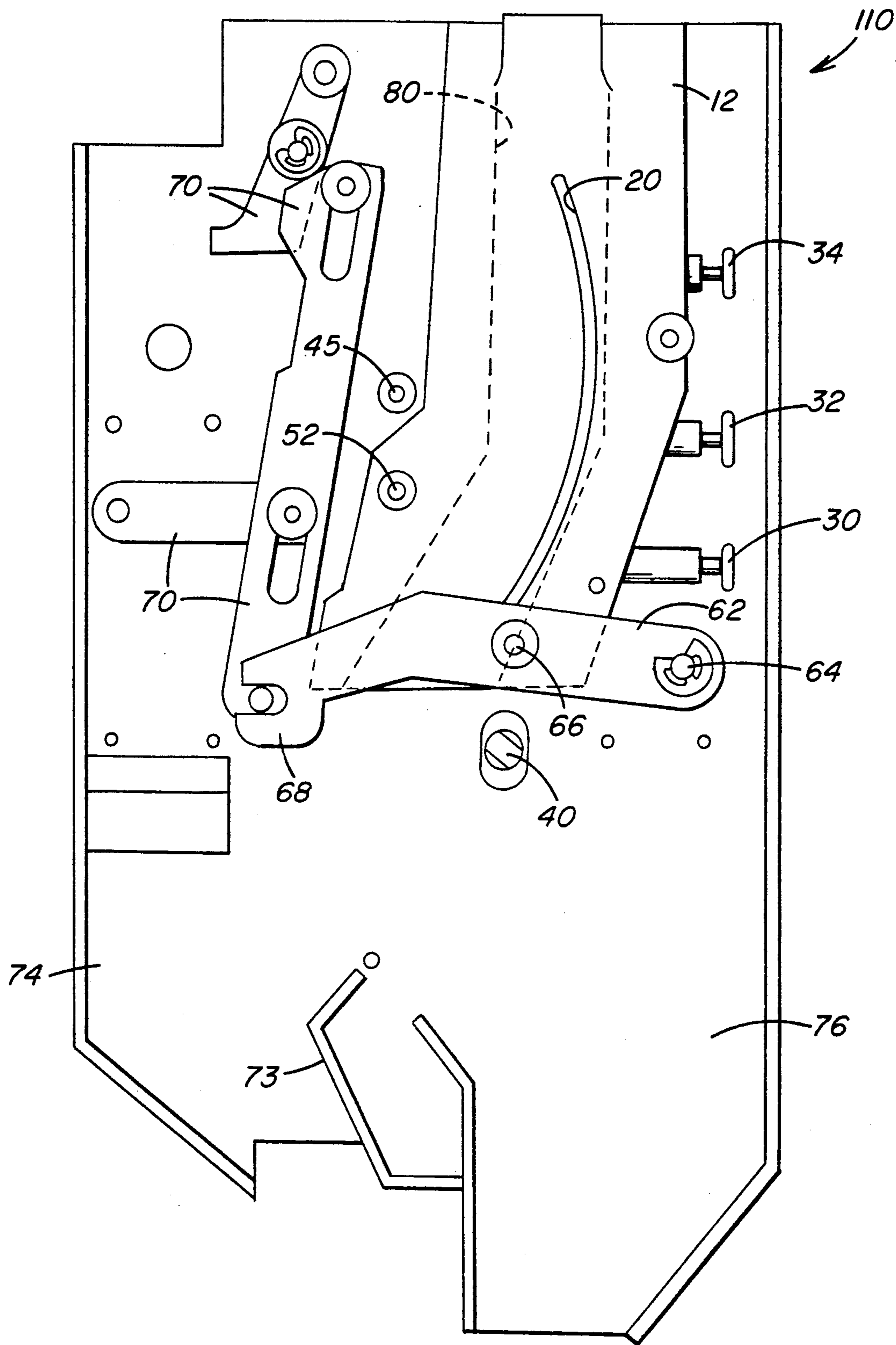
FIG. 5 PRIOR ART
