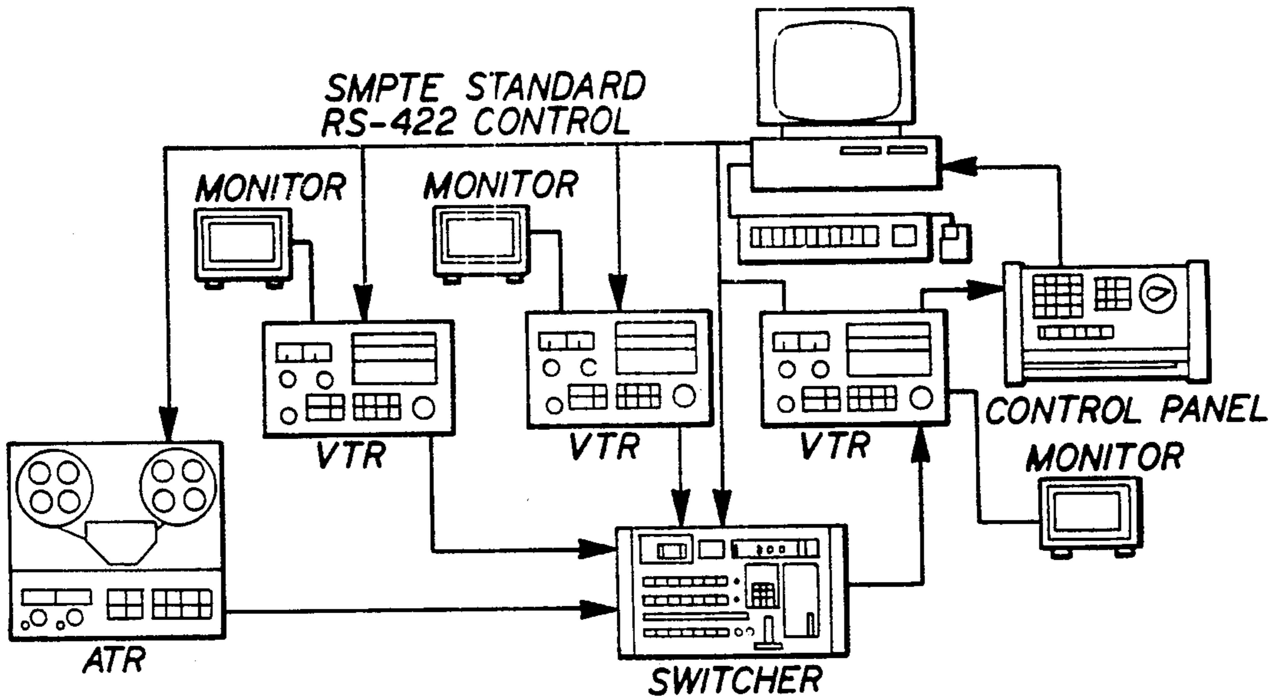
FIG. 1 PRIOR ART
