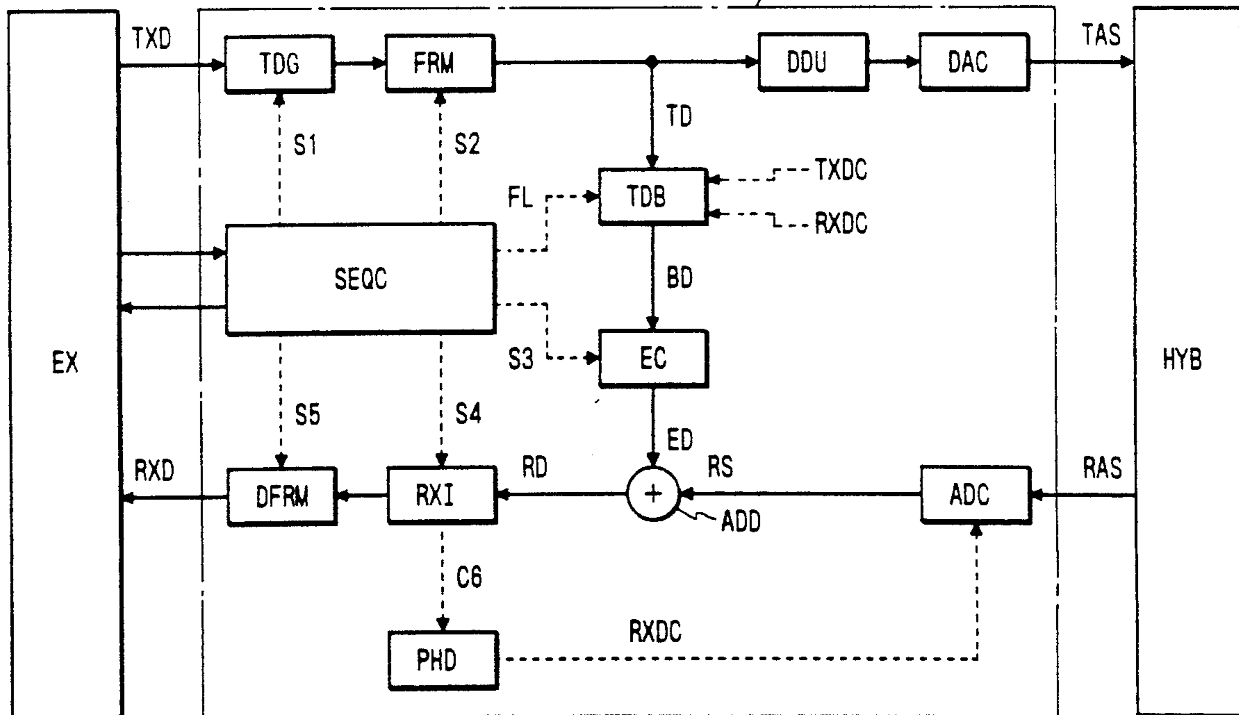
ECIC : ECHO CANCELER INTEGRATED CIRCUIT
