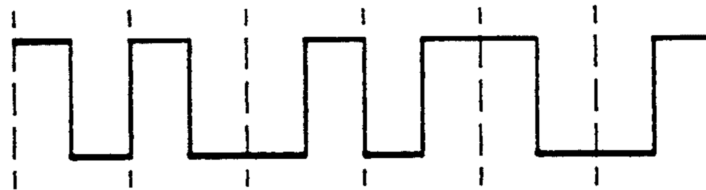
(c) MANCHESTER
