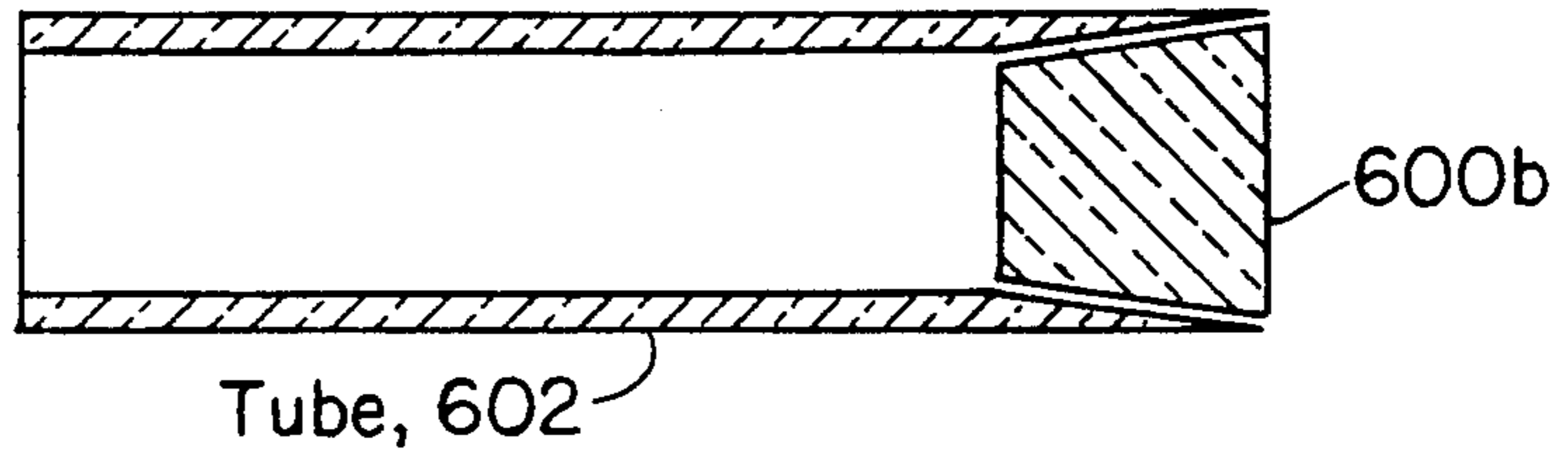
FIG. 9B CONICAL CONSTRUCTION
