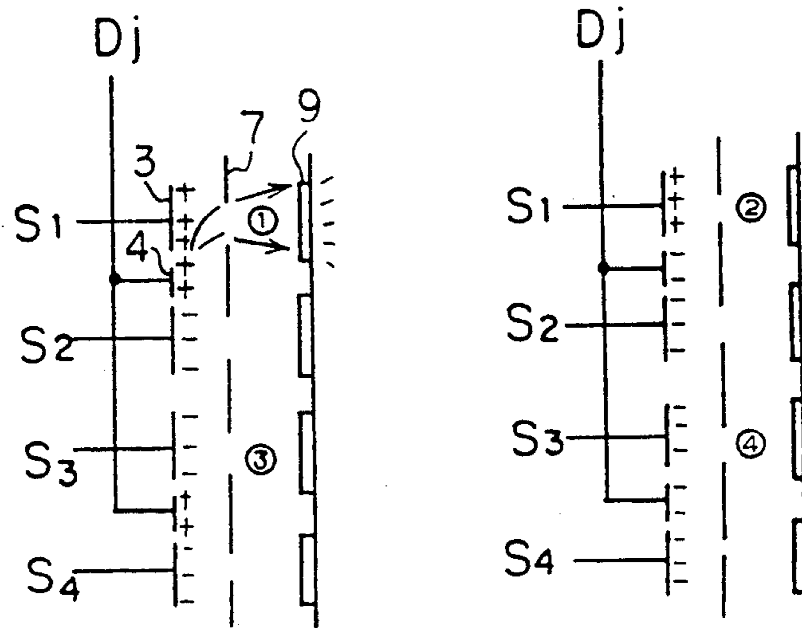
FIG. 5 (PRIOR ART)
