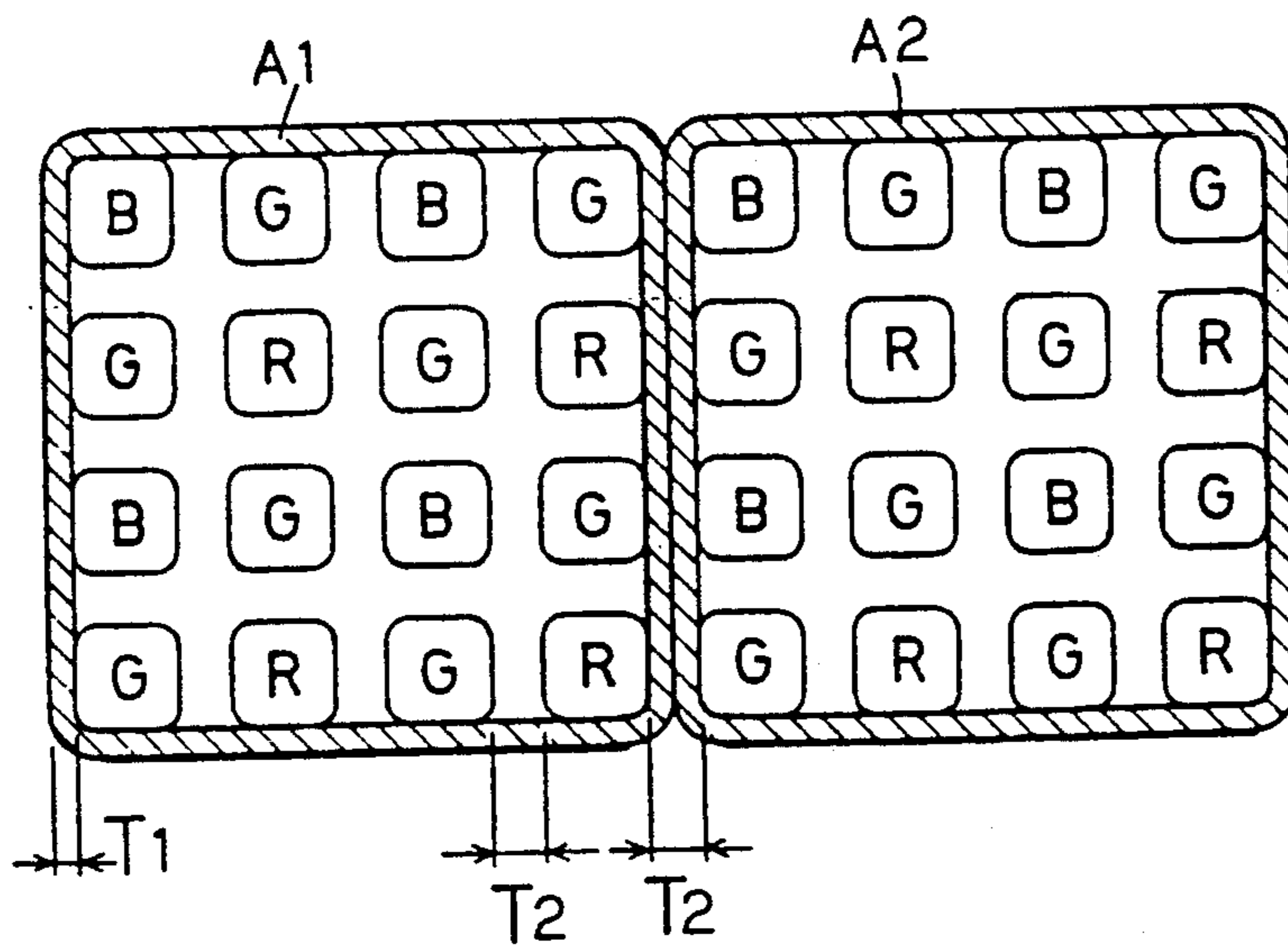
FIG. 6 (PRIOR ART)
